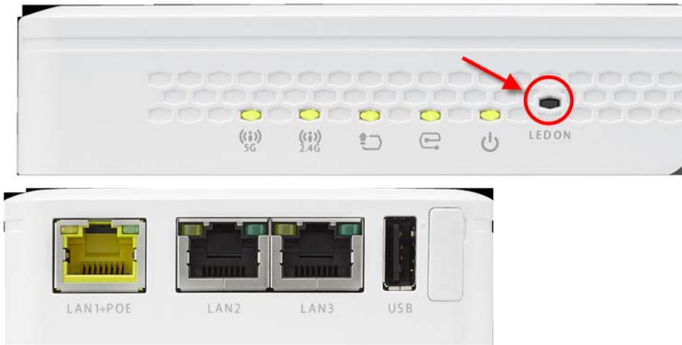
Figure 24 WAC5302D-S LEDs
