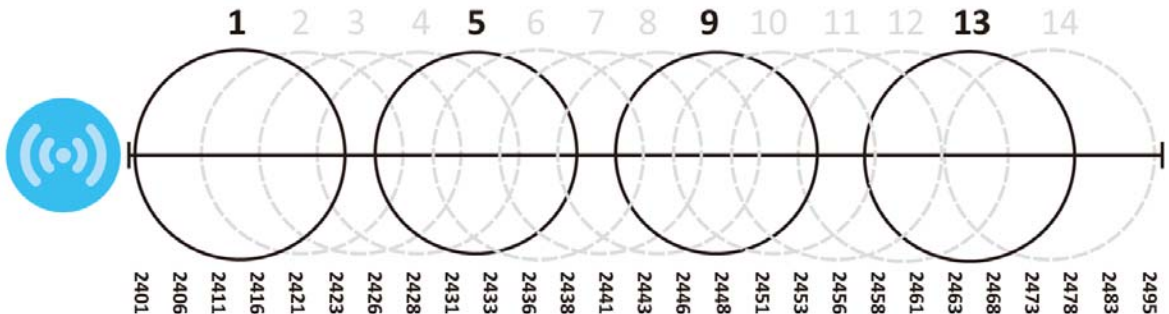
Figure 81 An Alternative Four-Channel Deployment
