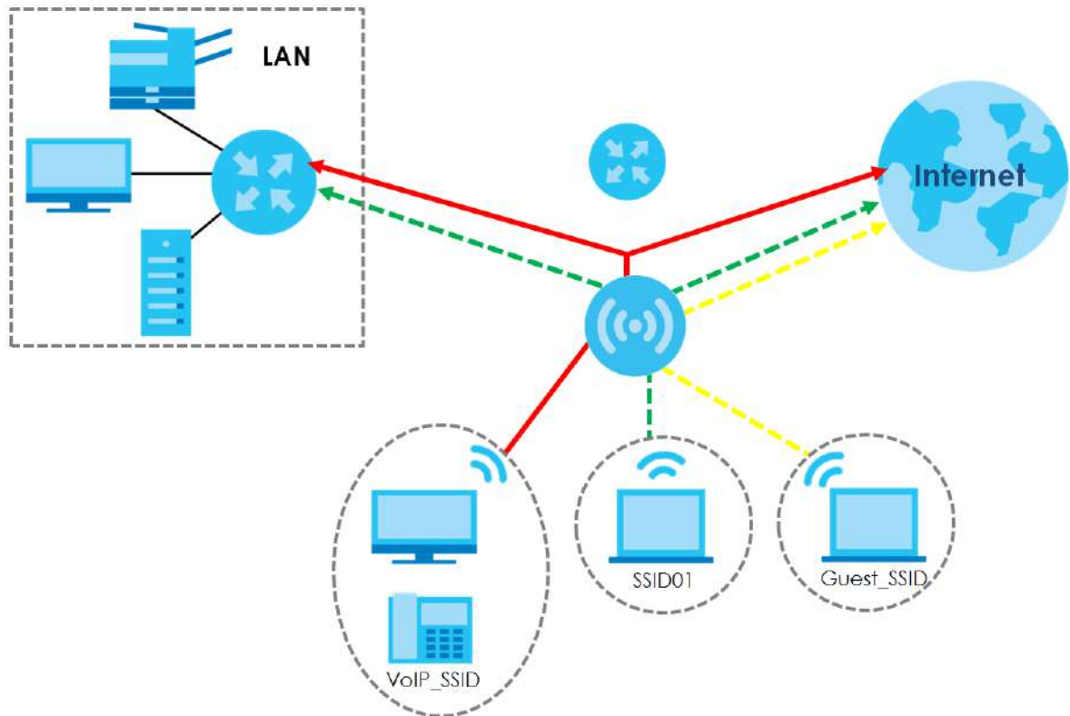
Figure 5 Multiple BSSs
