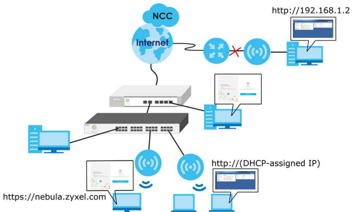
Figure 163 Cloud Mode Application
