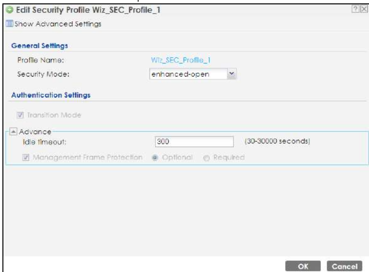
Figure 100 Configuration > Object > AP Profile > SSID > Security List > Add/Edit Security Profile> Security Mode: enhanced-open
