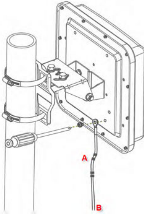
Figure 15 Grounding Example
