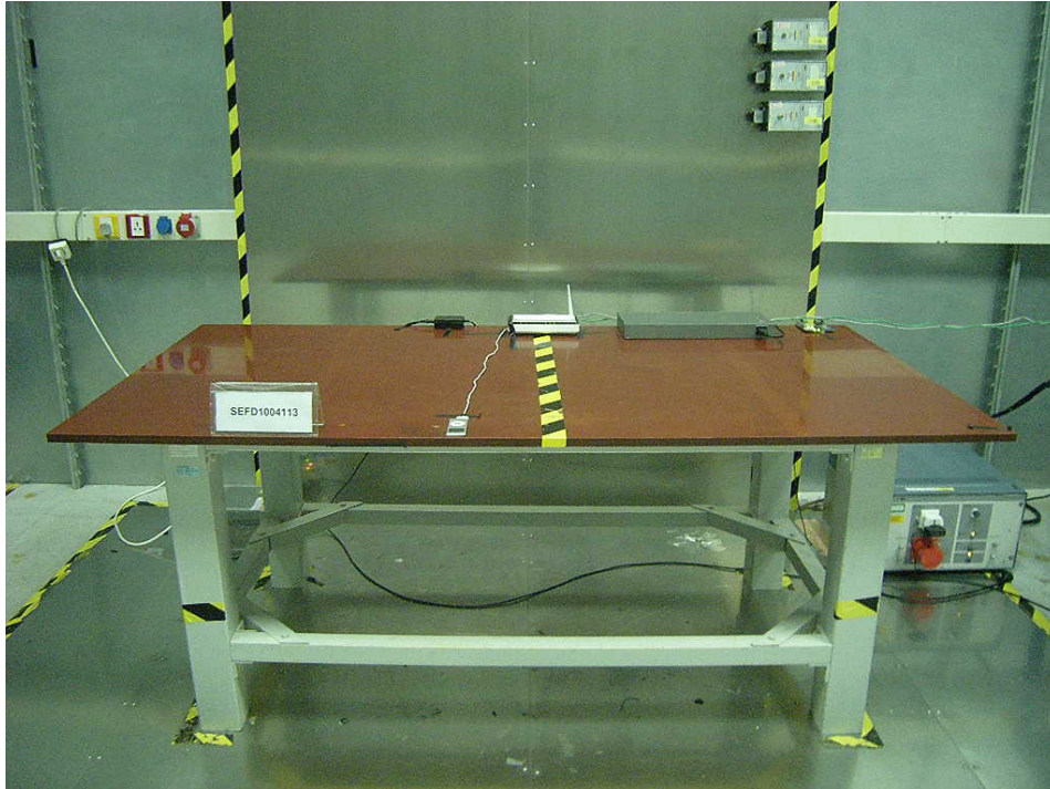
Front View of Conducted Emission Test
