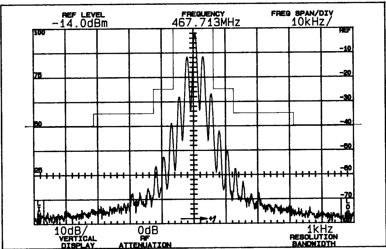
FIGURE 4 OCCUPIED BANDWIDTH
