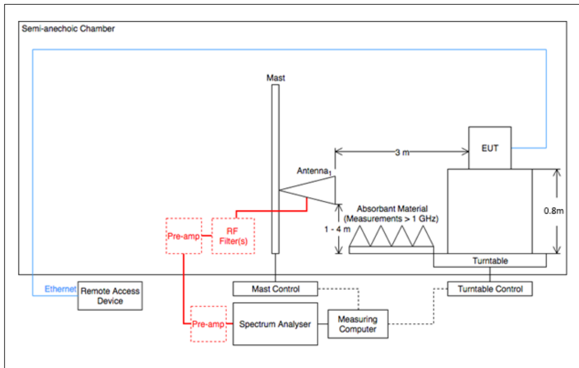
Figure 5 - Radiated Disturbance Example Test Setup
