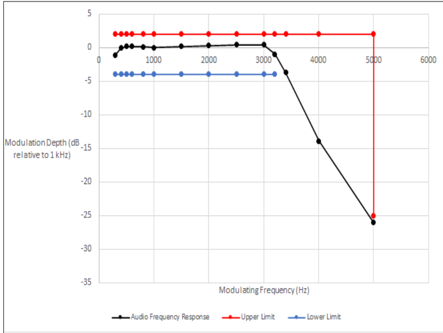
Figure 37 - Frequency Response
