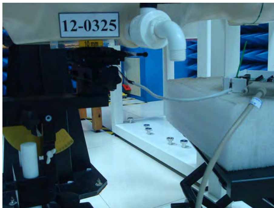
Figure 1. Body SAR Test Setup (Flat Section)
