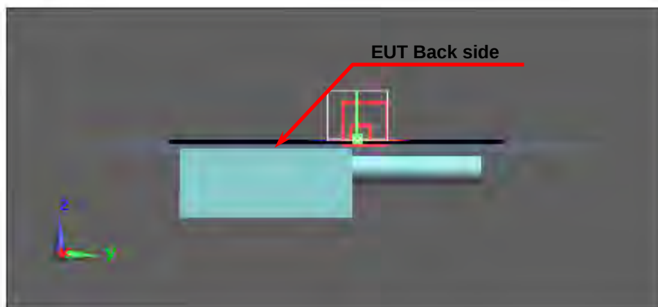
Figure 2. Body SAR Test Setup (Flat Section)
