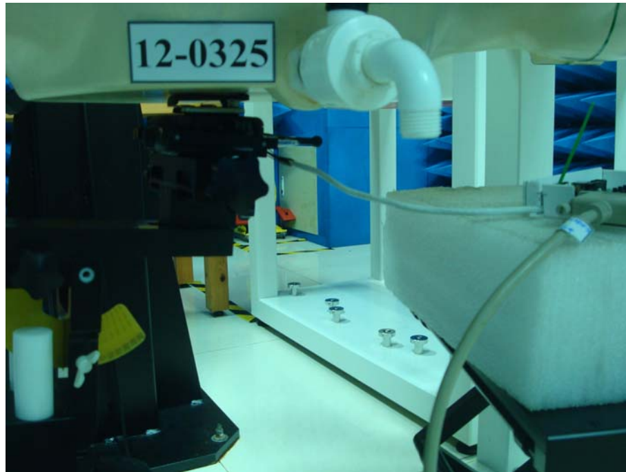
Figure 4. Body SAR Test Setup (Flat Section)
