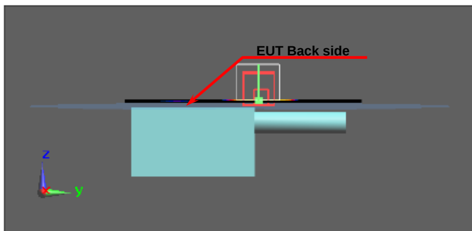
Figure 4. Body SAR Test Setup (Flat Section)
