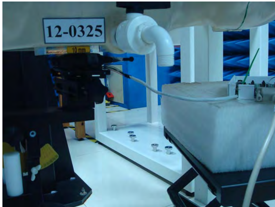
Figure 3. Body SAR Test Setup (Flat Section)
