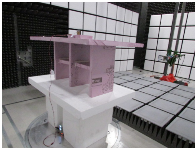
Figure 2: Radiated Spurious Emissions – Front View
