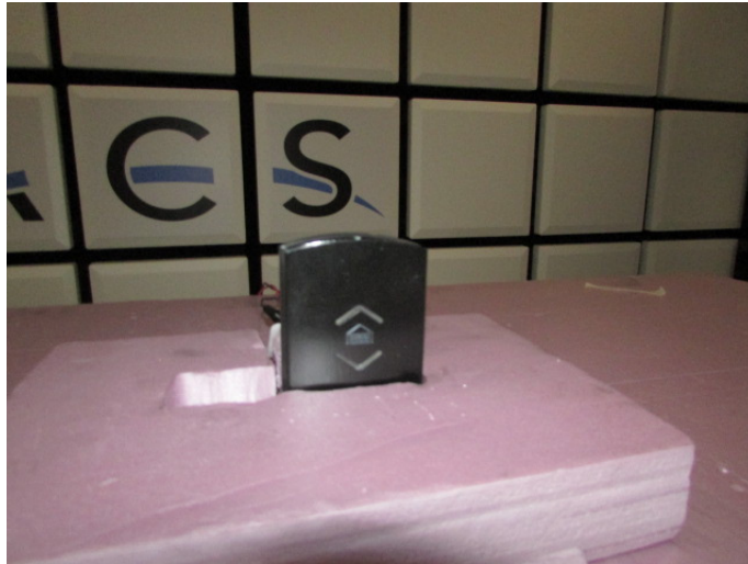
Figure 3: Radiated Spurious Emissions Test Setup – Front View
