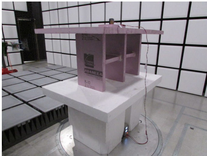
Figure 1: Radiated Spurious Emissions – Rear View
