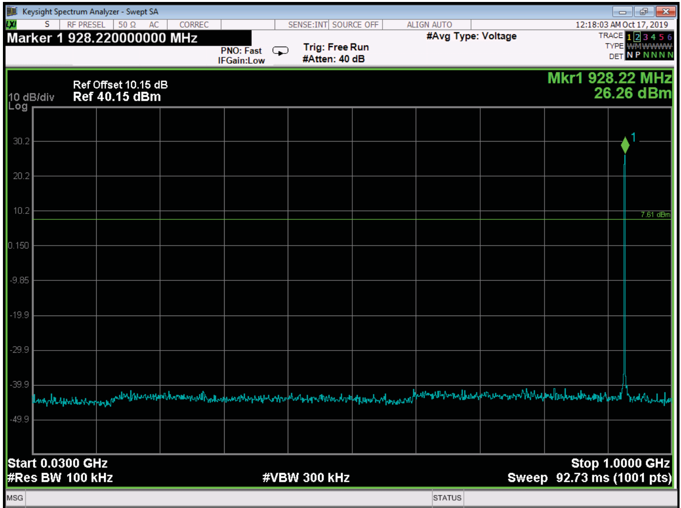
RF Antenna Conducted – High Channel – 30 MHz to 1000 MHz
