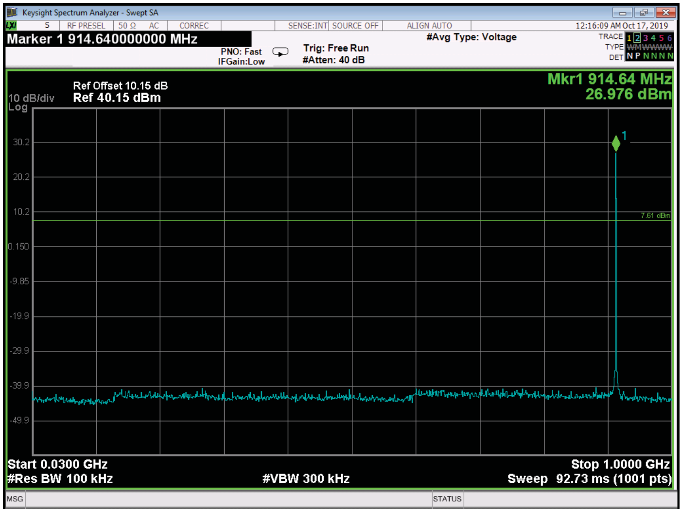
RF Antenna Conducted – Middle Channel – 30 MHz to 1000 MHz
