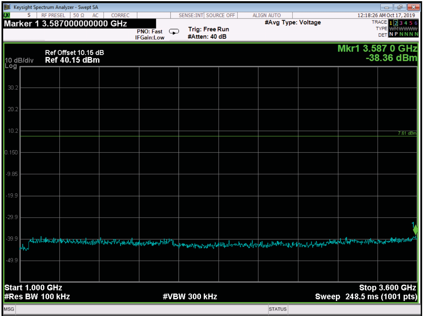
RF Antenna Conducted – High Channel – 1000 MHz to 3600 MHz
