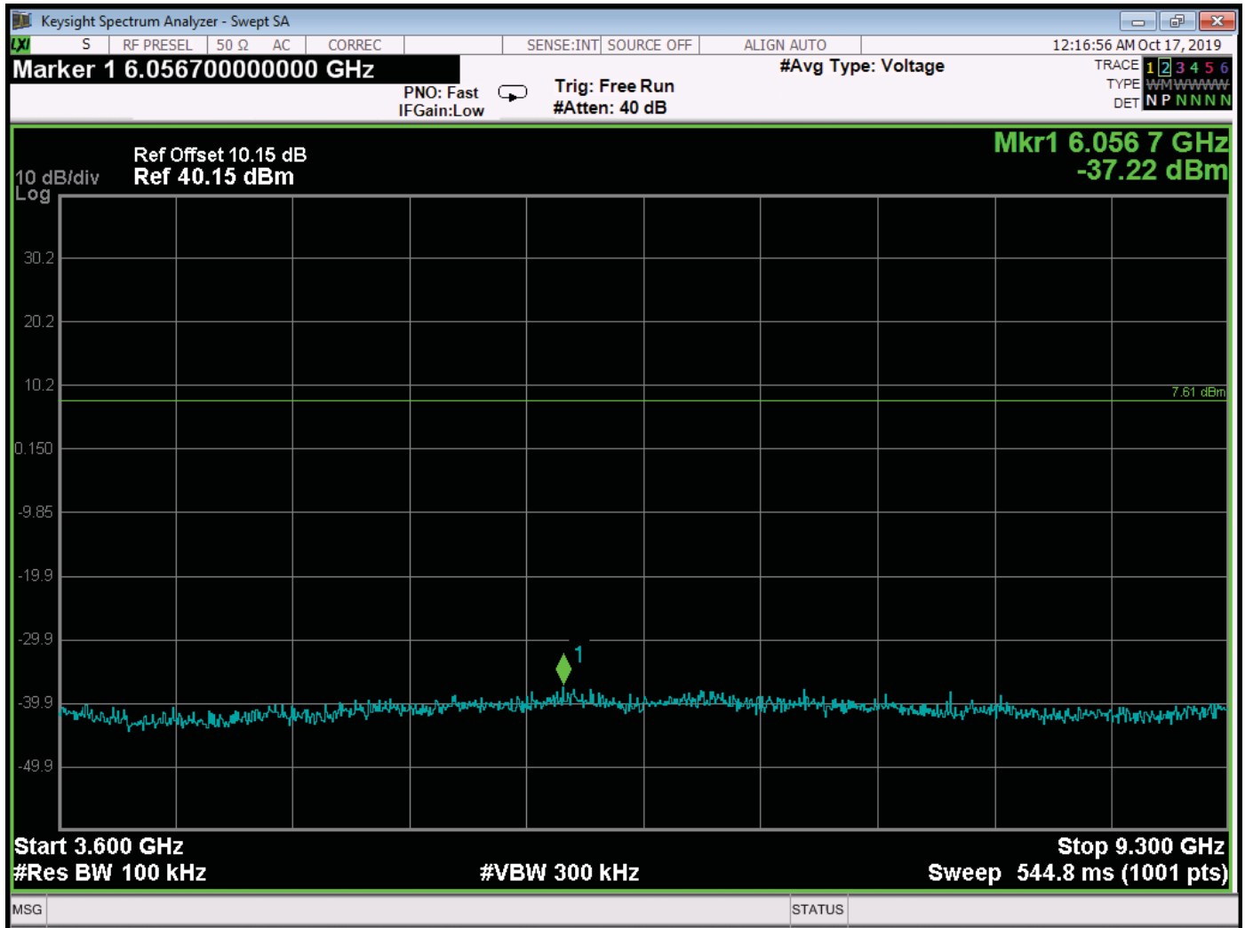
RF Antenna Conducted – Middle Channel – 3600 MHz to 9300 MHz
