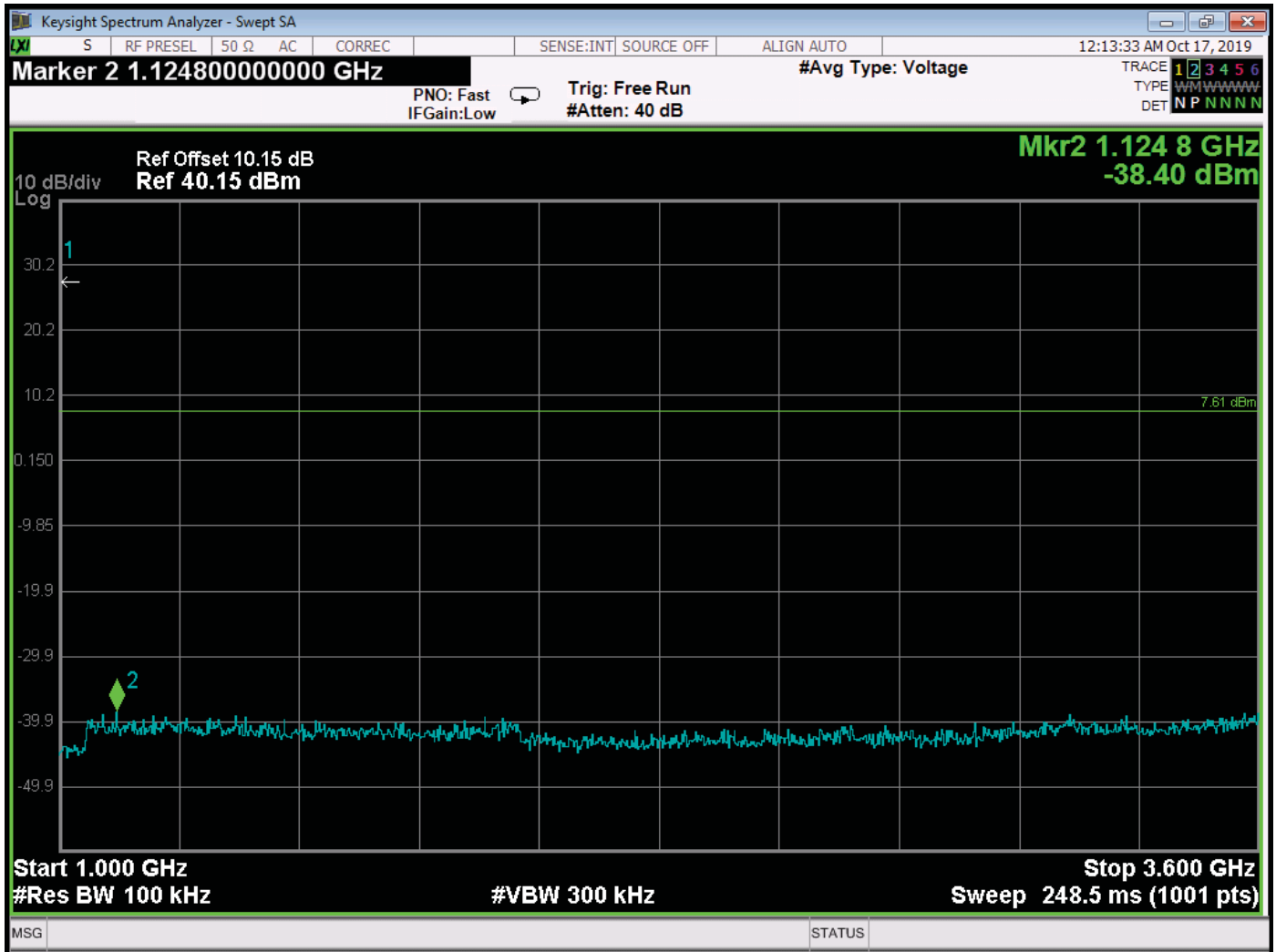
RF Antenna Conducted – Low Channel – 1000 MHz to 3600 MHz
