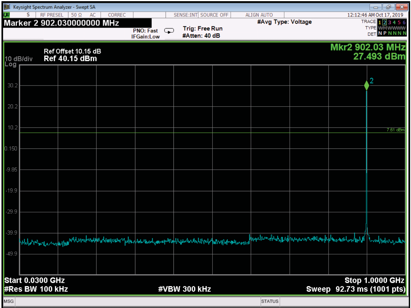
RF Antenna Conducted – Low Channel – 30 MHz to 1000 MHz
