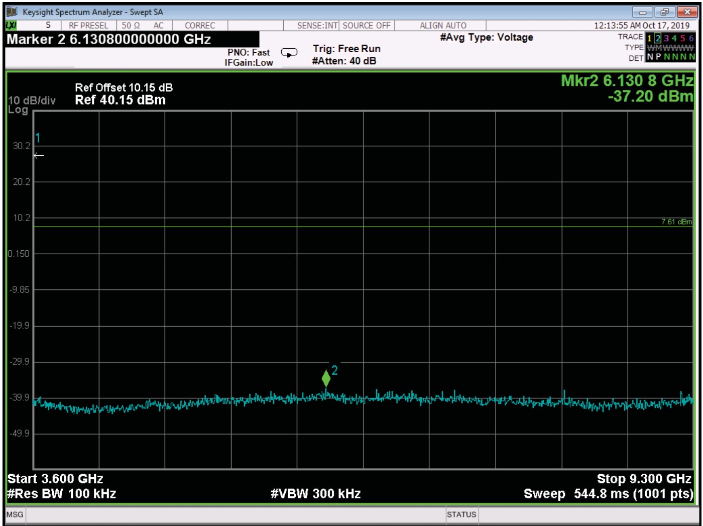
RF Antenna Conducted – Low Channel – 3600 MHz to 9300 MHz
