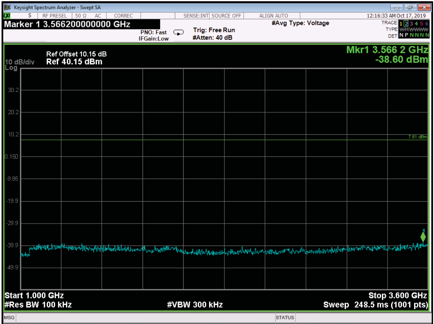
RF Antenna Conducted – Middle Channel – 1000 MHz to 3600 MHz
