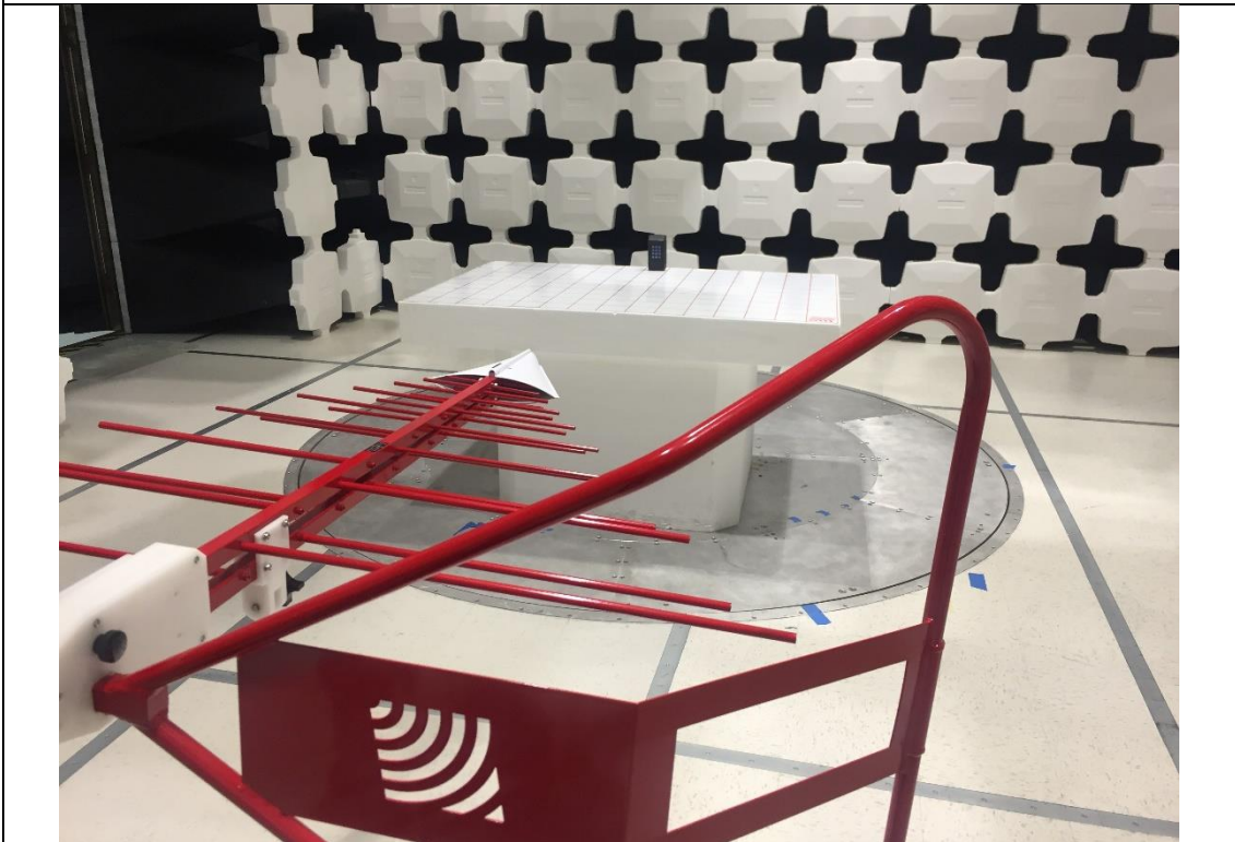
Radiated Emissions Below 1GHz setup – MMK200
