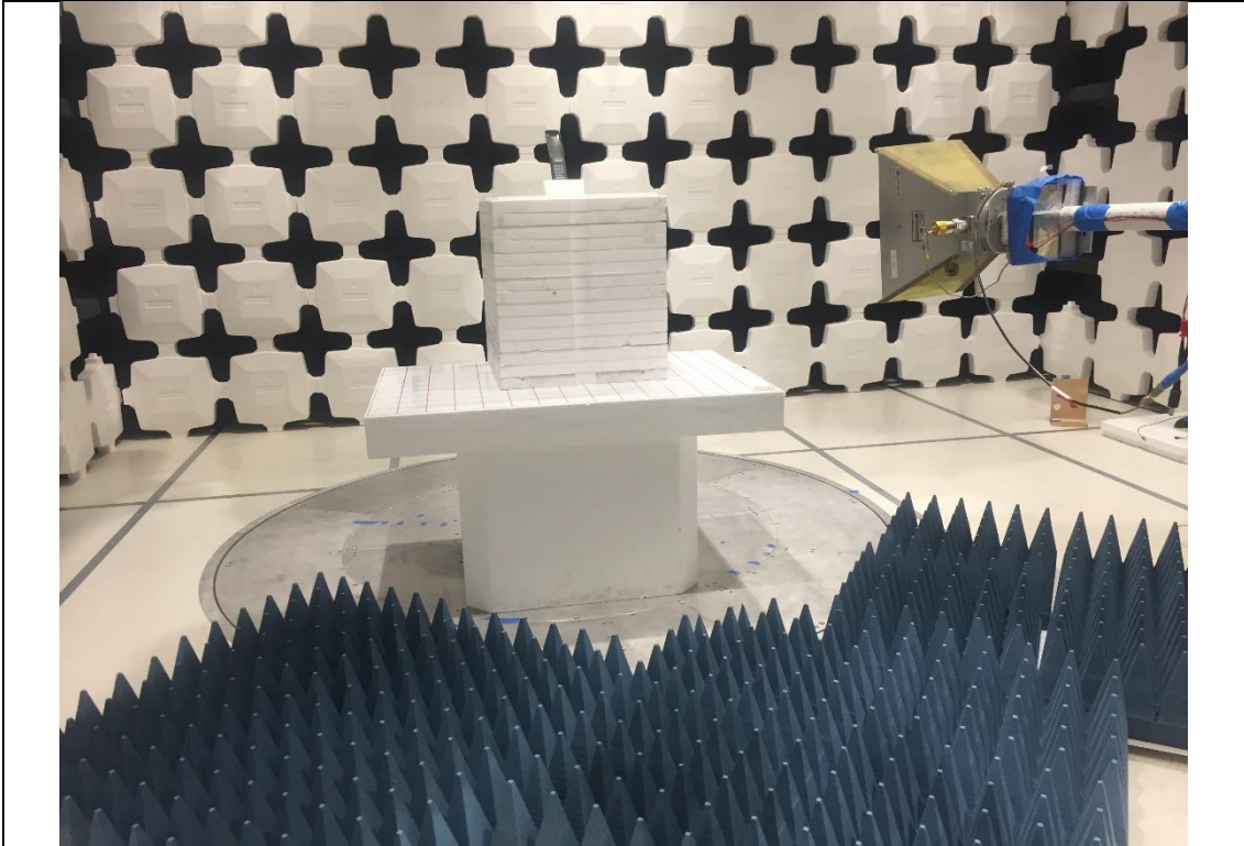
Radiated Emissions Above 1GHz setup – MMK100
