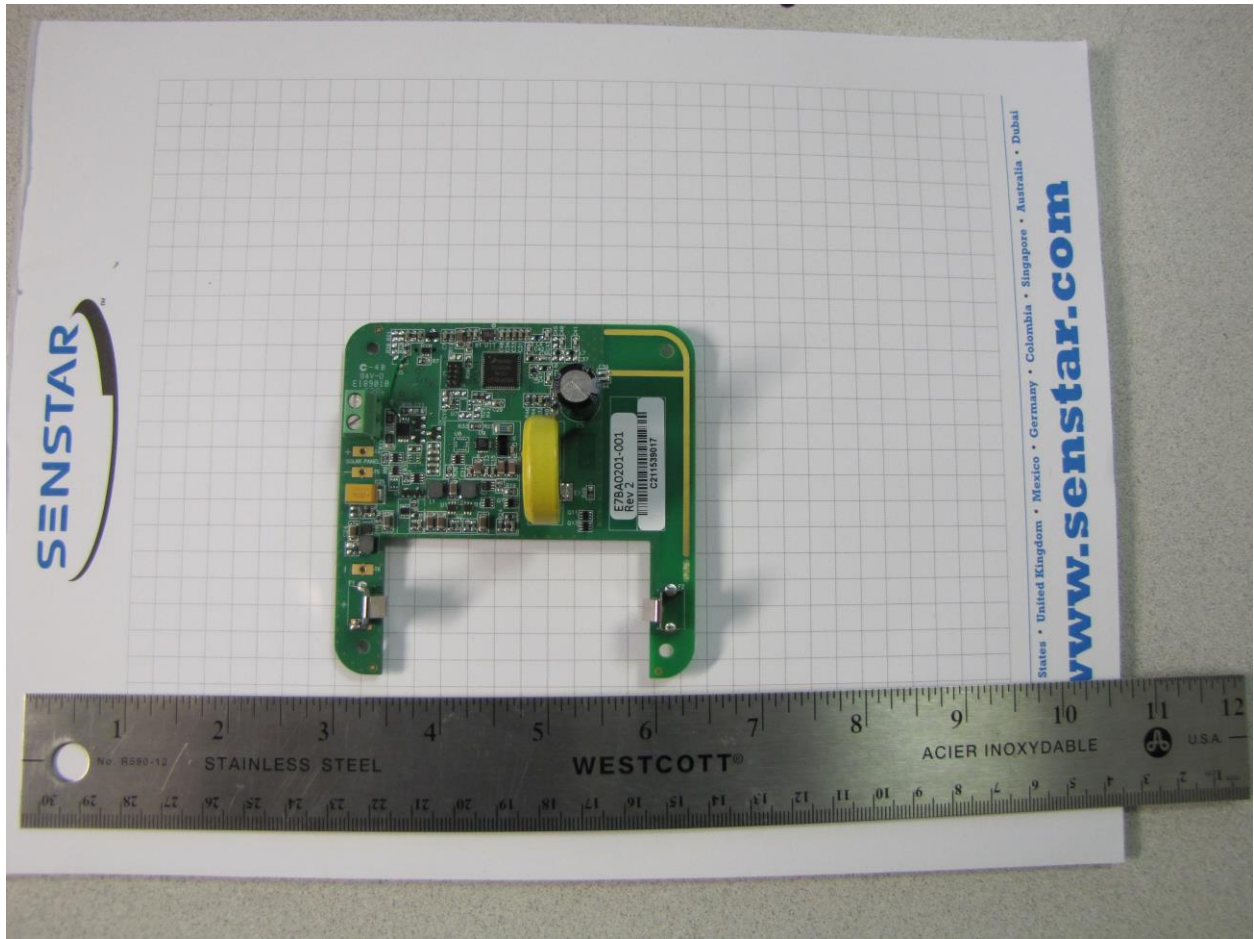
15T-E7EM0201 Printed Circuit Board Assembly (E7BA0201) Top View
