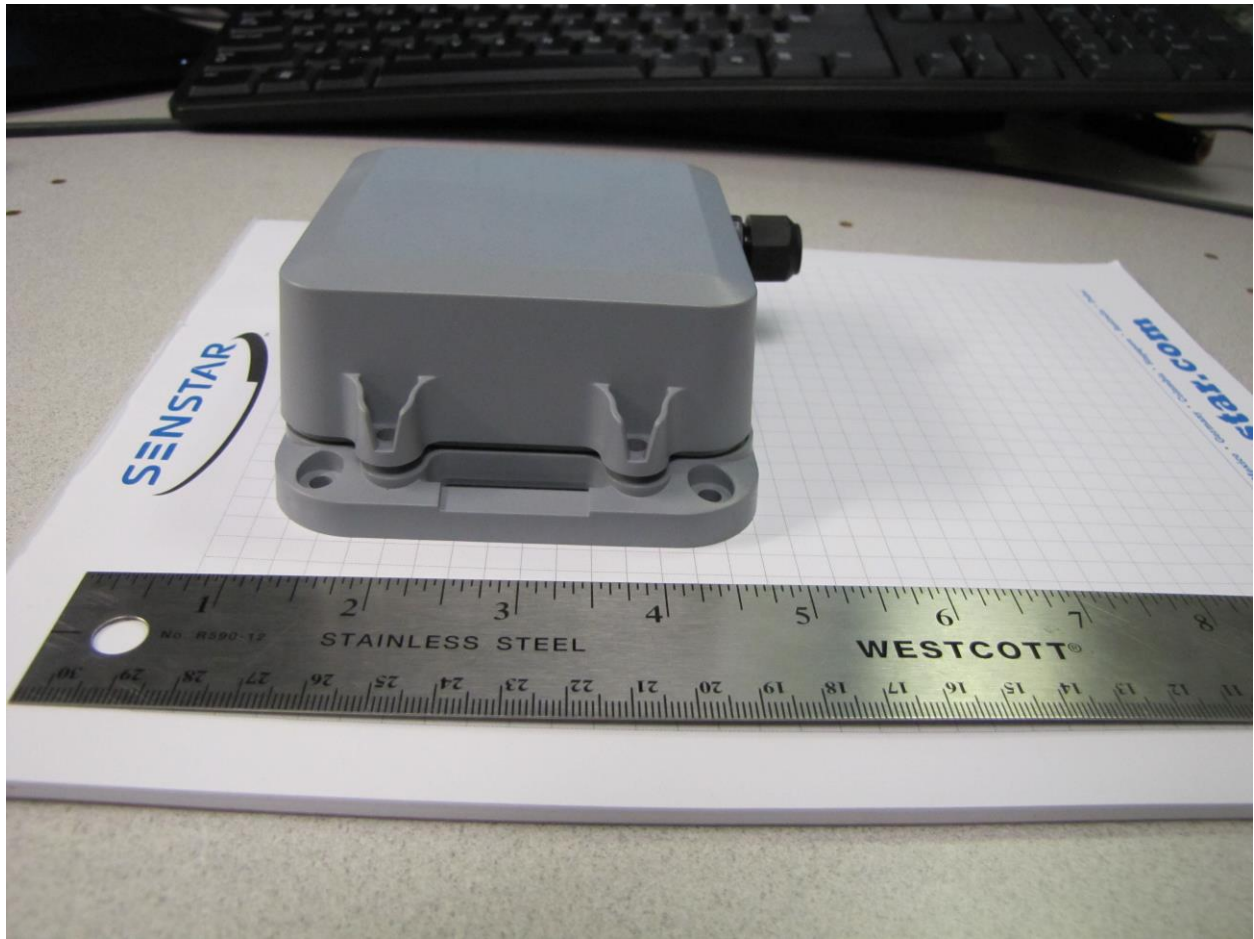
IST-E7EM0201 Left Side View
