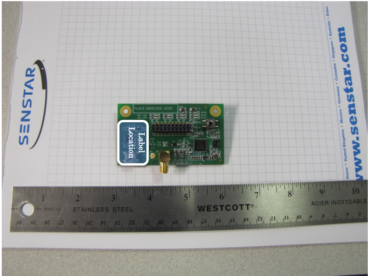
IST-E7BA0300 Printed Circuit Board Assembly with diagnostic USB & SMA connectors populated – Top View
