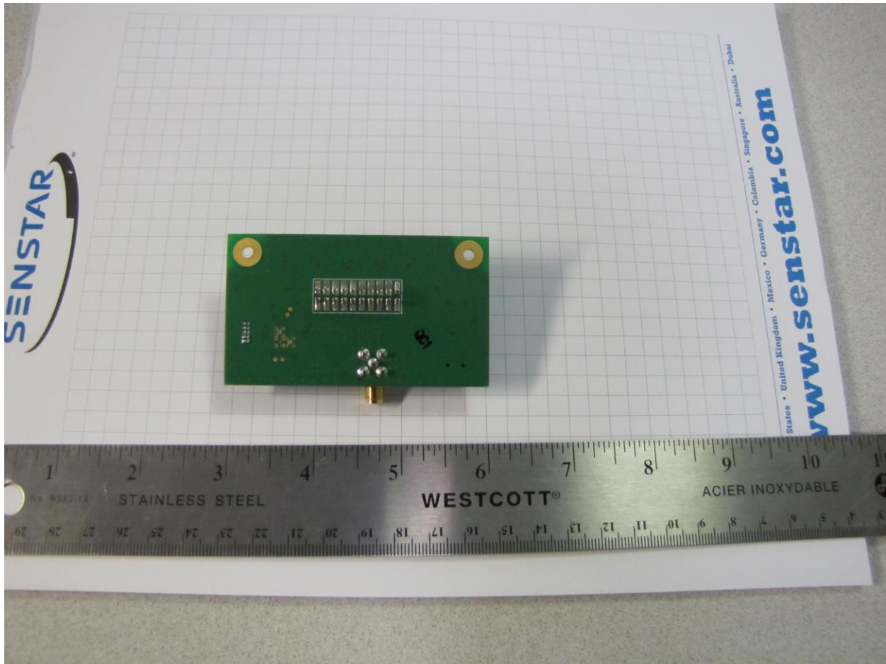
I5T-E7BA0300 Printed Circuit Board Assembly with diagnostic USB & SMA connectors populated – Bottom View
