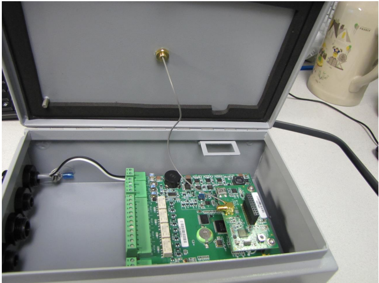
I5T-E7BA0300 Mounted in Host – Internal Side View
