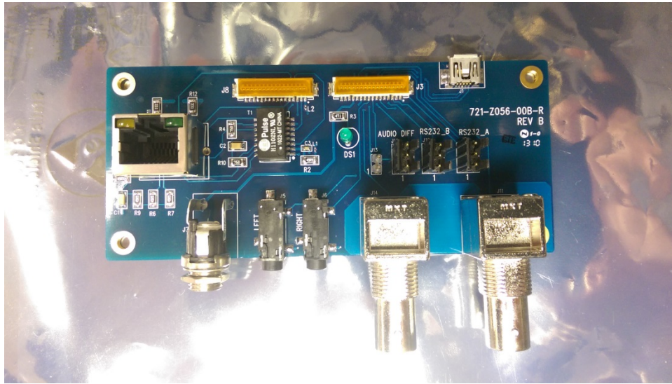
EUT Interface Board
