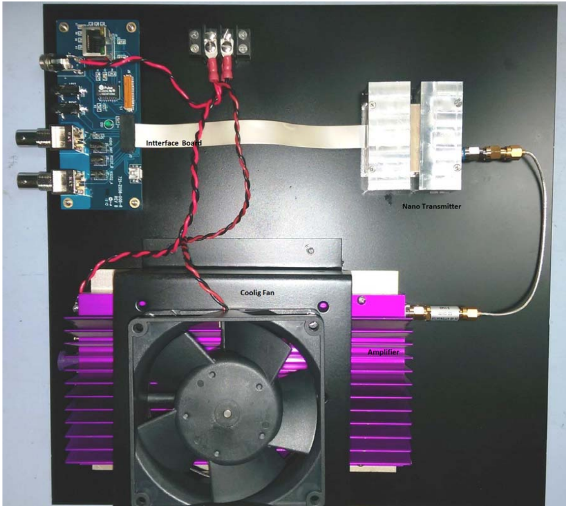
EUT Top View
