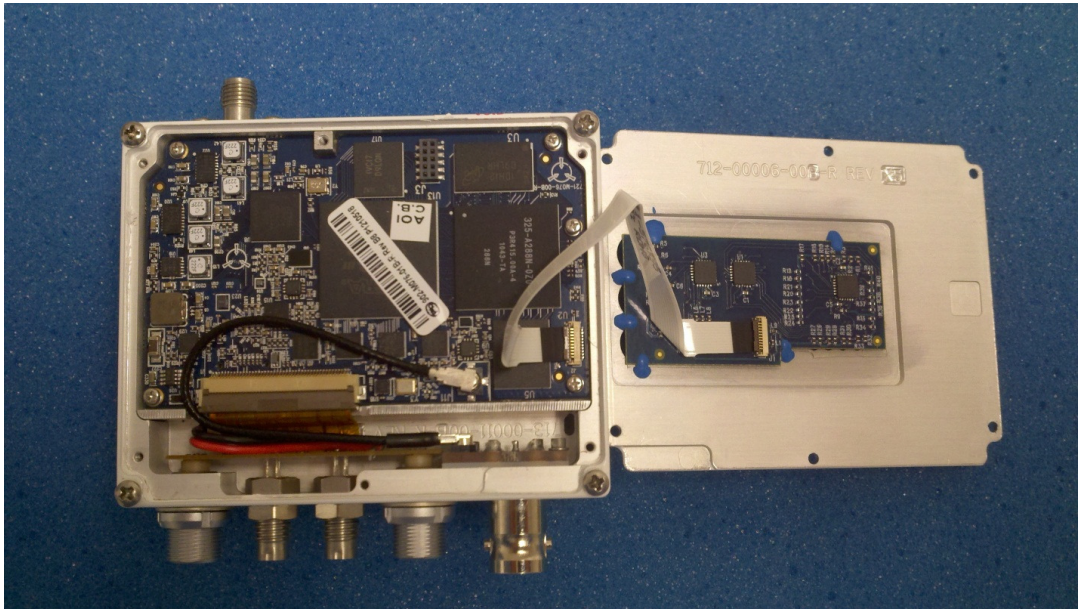
Photo 1 Top Opened
