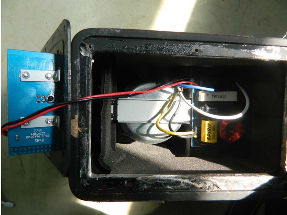
Inside View for Left Speaker
