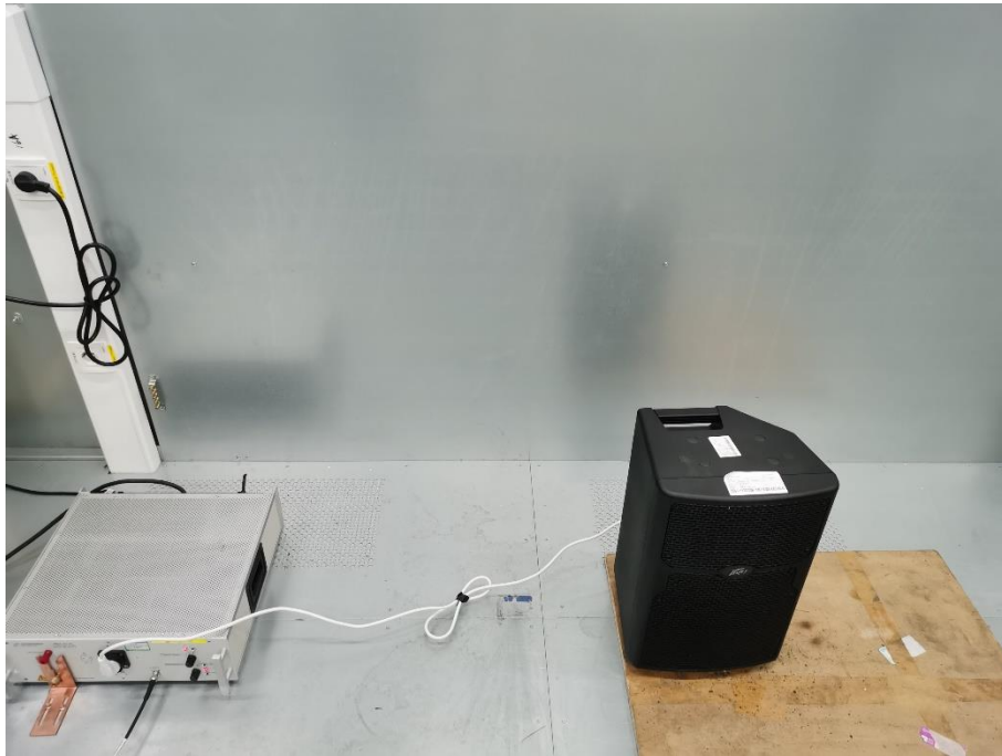
PVX p10 Conducted Emission
