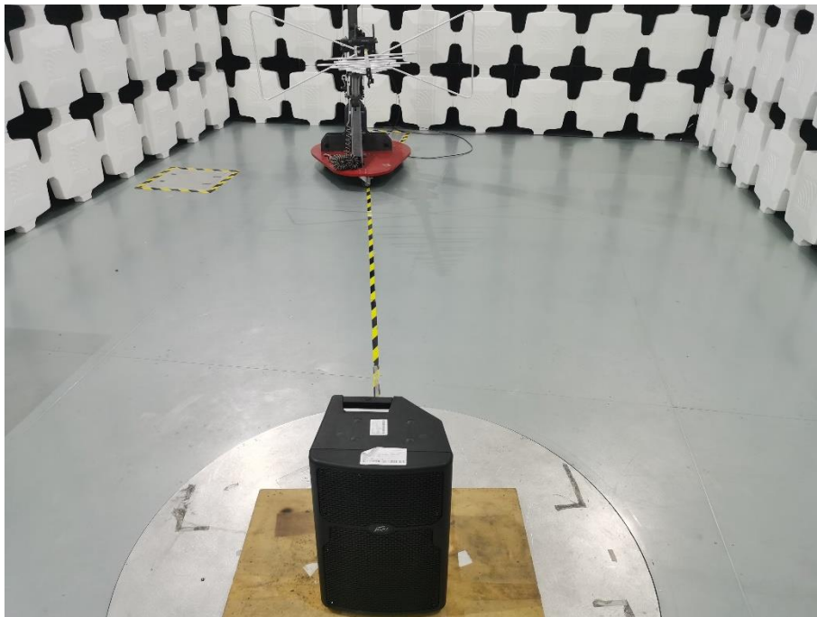
PVX p10 Radiated Emission test below 1GHz
