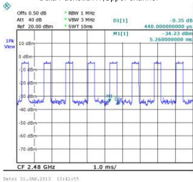
Data Packet:DH1,Upper channel
