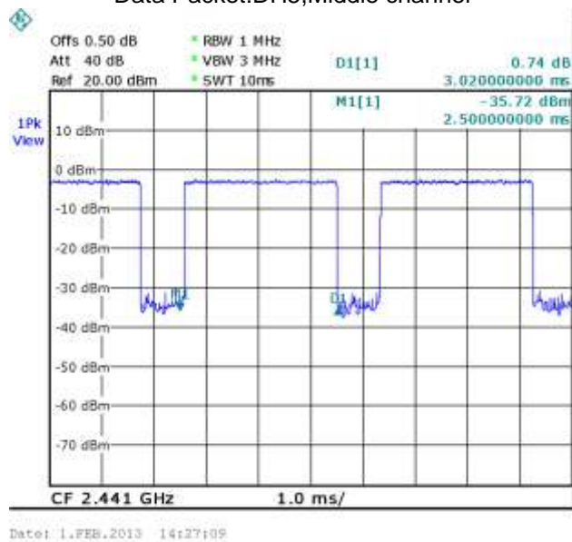
Data Packet:DH5,Middle channel
