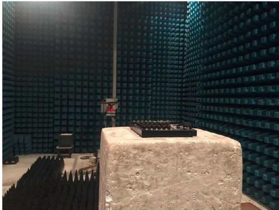
Description: Radiated Emission Test Setup for 1~18GHz
