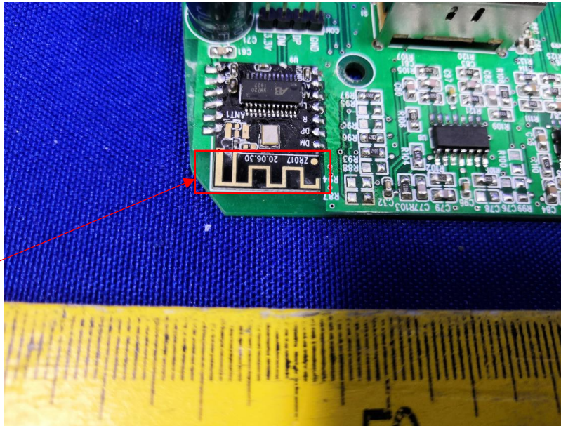
Bluetooth Antenna
