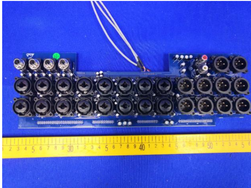
PCB-5 front view
