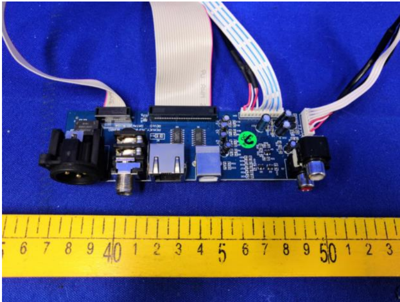
PCB-4 back view
