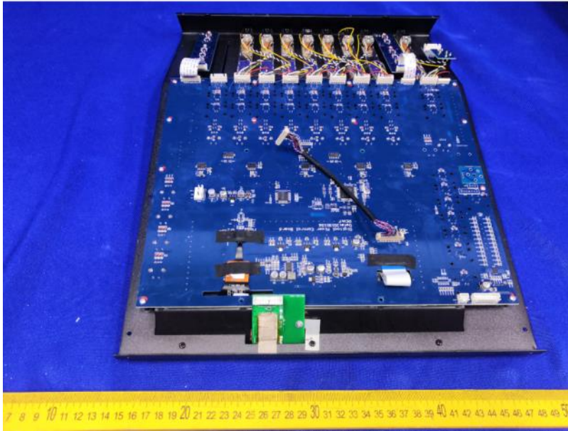
Key board front view
