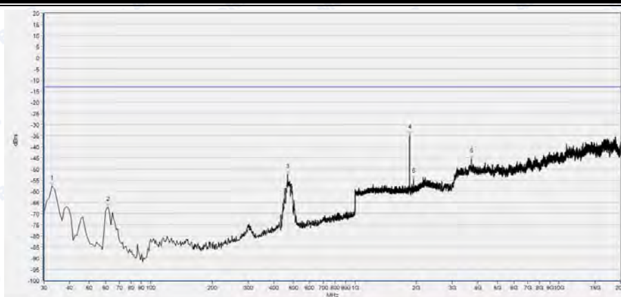
(Plot J1: HSDPA 1900MHz Channel = 9262, Test Antenna Horizontal)
