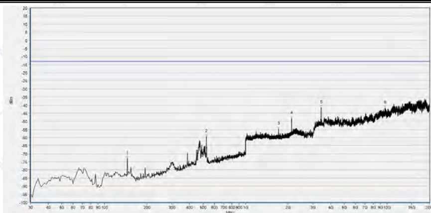
(Plot O1: HSPA+ 1700MHz Channel = 1312, Test Antenna Horizontal)
