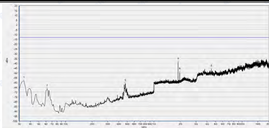
(Plot J3: HSDPA 1900MHz Channel = 9400, Test Antenna Horizontal)
