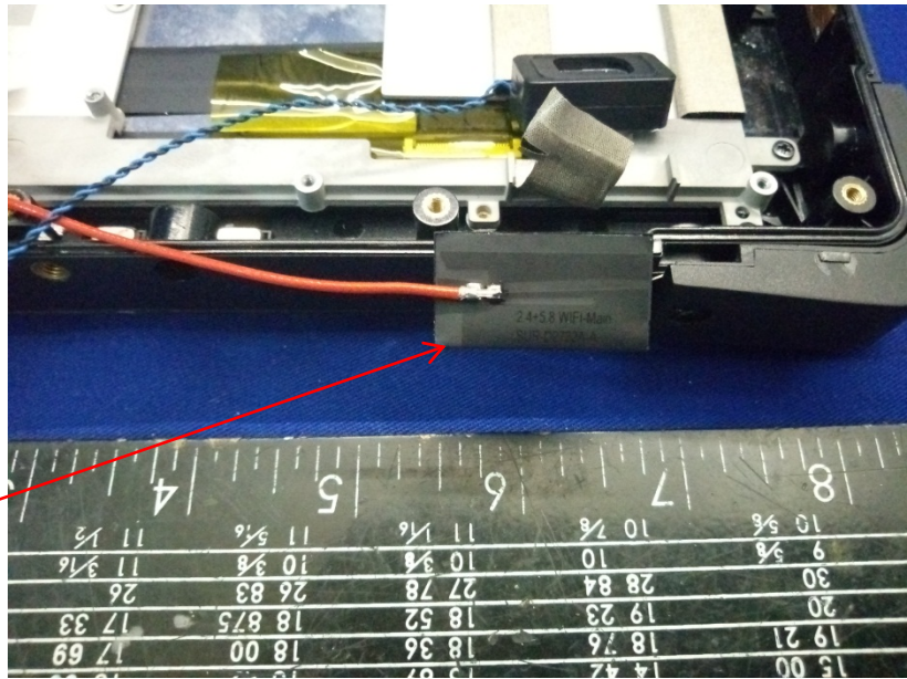
WiFi Main Antenna
