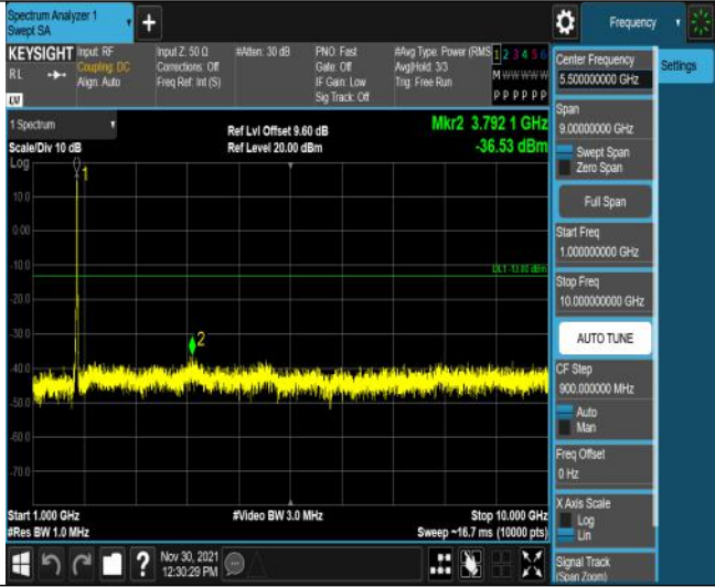
Band66-20MHz-16QAM-132572-100RB#0-Range2:1000~10000MHz
