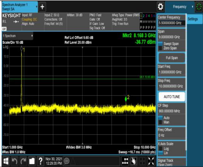
Band66-20MHz-16QAM-132322-100RB#0-Range2:1000~10000MHz
