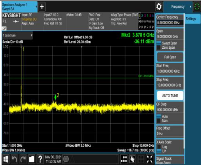
Band66-10MHz-16QAM-132322-50RB#0-Range2:1000~10000MHz
