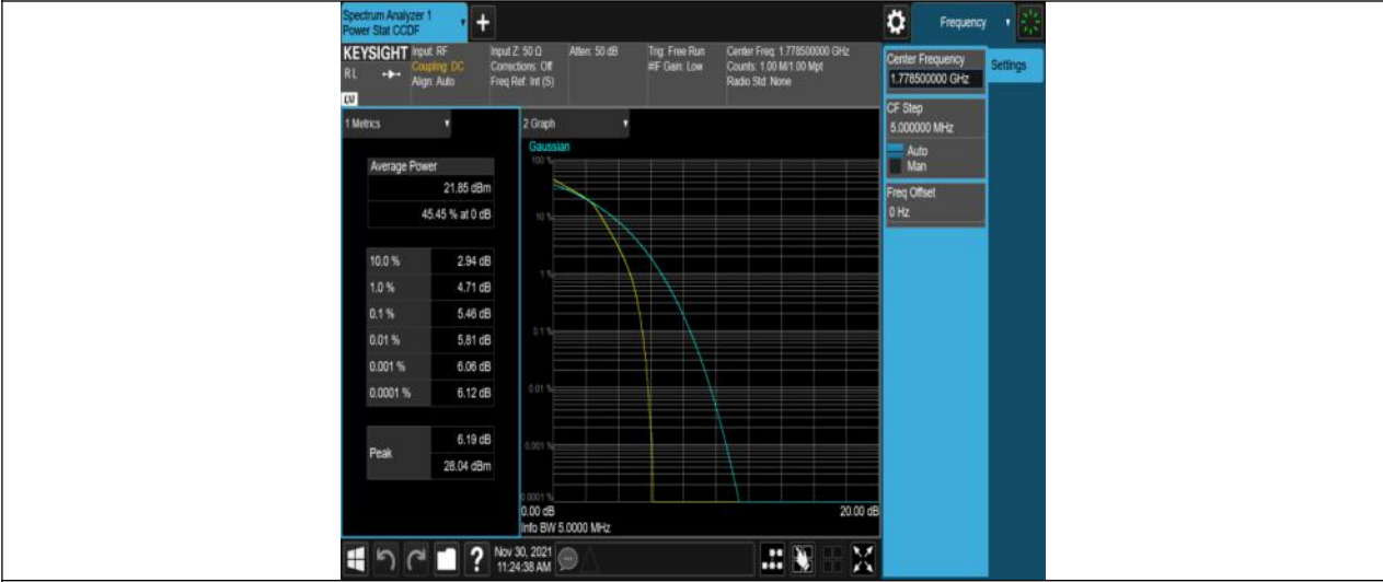
Band66-3MHz-16QAM-132657-15RB#0
