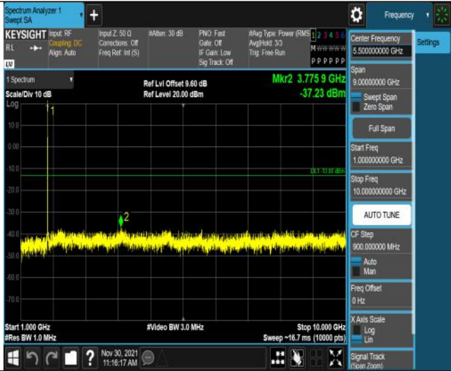
Band66-3MHz-16QAM-132322-15RB#0-Range2: 1000~10000MHz
