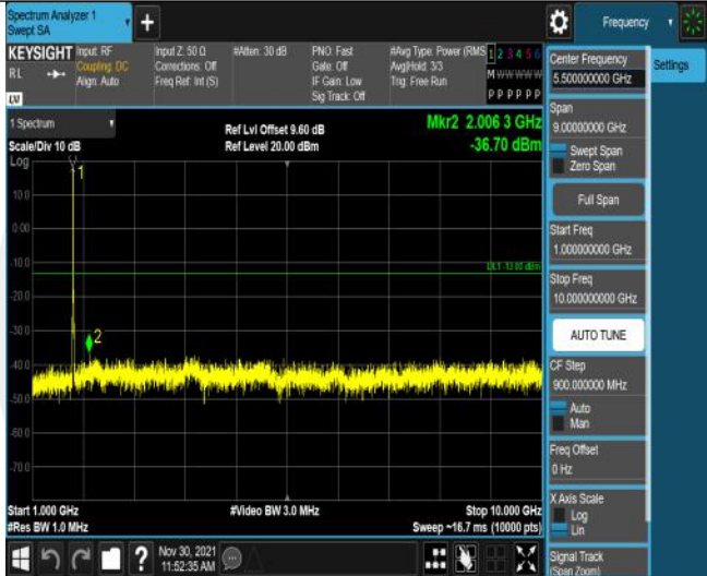
Band66-10MHz-16QAM-132022-50RB#0-Range2:1000~10000MHz
