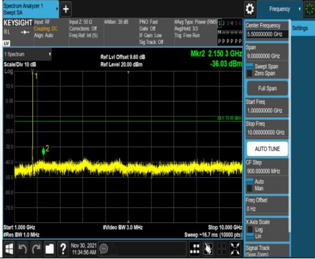
Band66-5MHz-16QAM-131997-25RB#0-Range2:1000~10000MHz
