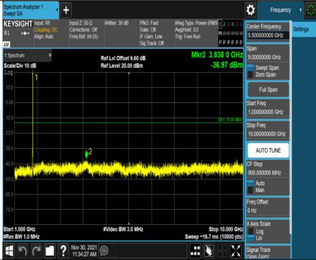
Band66-5MHz-QPSK-131997-25RB#0-Range2:1000~10000MHz
