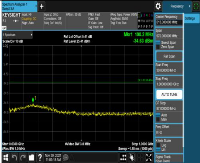
Band66-10MHz-16QAM-132322-50RB#0-Range1:30~1000MHz
