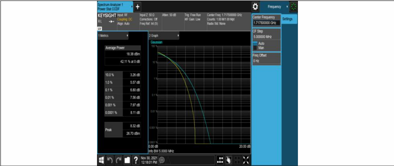
Band66-15MHz-16QAM-132047-75RB#0
