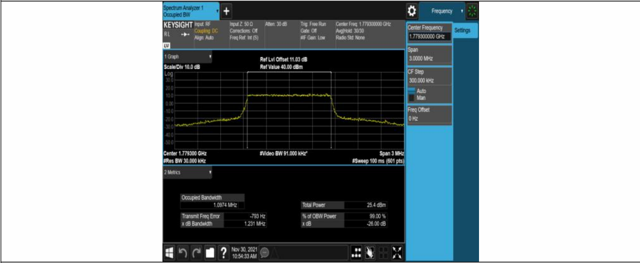
Band66-1.4MHz-QPSK-132665-6RB#0
