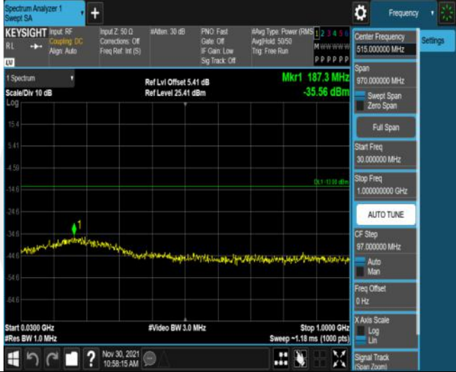
Band66-1.4MHz-QPSK-132665-6RB#0-Range1:30~1000MHz
