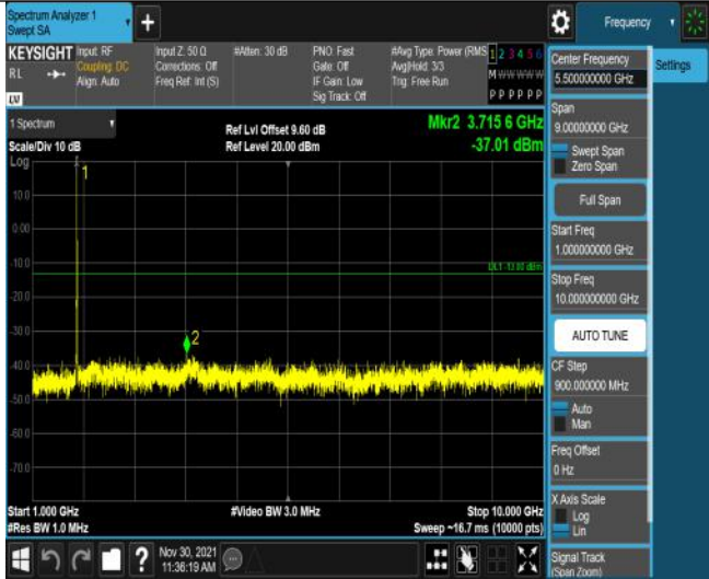
Band66-5MHz-QPSK-132647-25RB#0-Range2:1000~10000MHz
