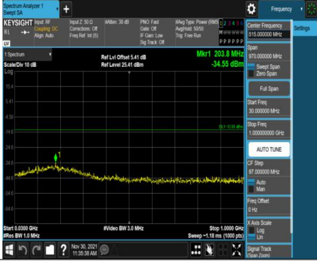
Band66-5MHz-16QAM-132322-25RB#0-Range1:30~1000MHz
