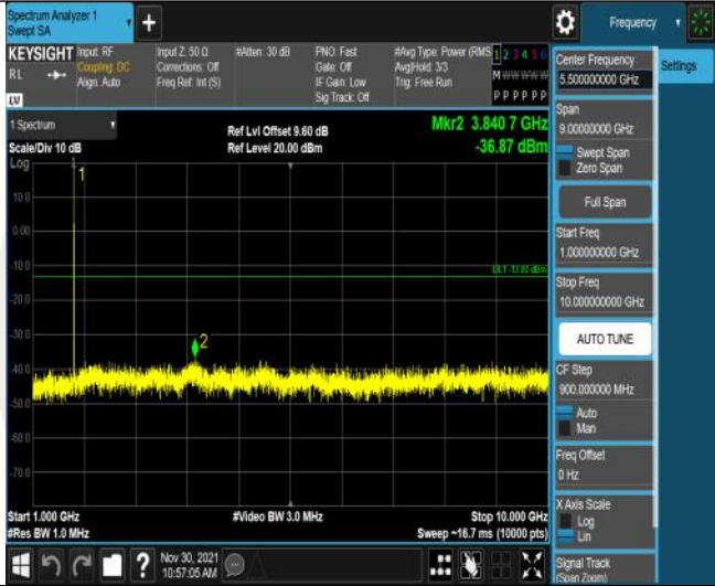
Band66-1.4MHz-16QAM-131979-6RB#0-Range2:1000~10000MHz
