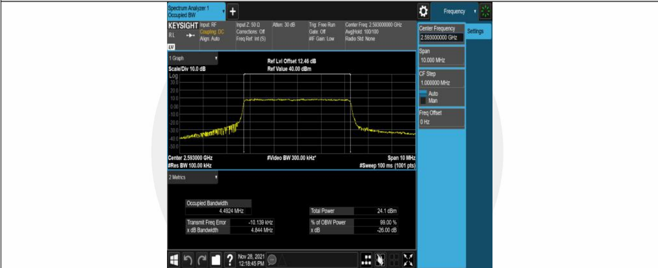
Band41-5MHz-16QAM-40620-25RB#0
