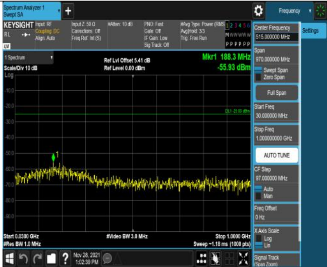
Band41-15MHz-QPSK-39725-75RB#0-Range1:30~1000MHz
