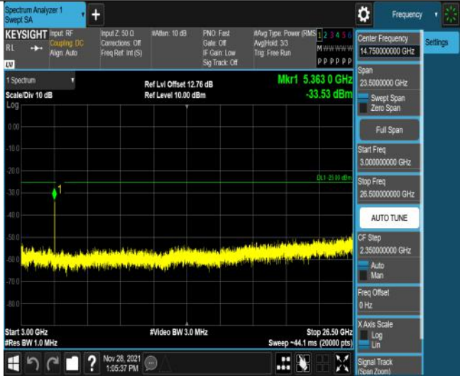
Band41-15MHz-QPSK-41515-75RB#0-Range3:3000~26500MHz
