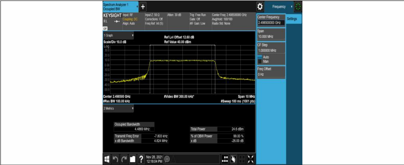
Band41-5MHz-16QAM-39675-25RB#0
