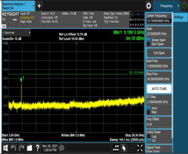
Band4 1-20MHz-16QAM-40620-100RB#0-Range3:3000~26500MHz
