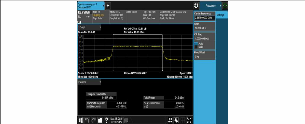
Band41-5MHz-16QAM-41565-25RB#0
