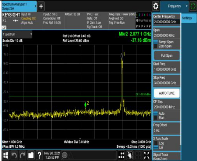
Band4 1-20MHz-16QAM-40620-100RB#0-Range2:1000~3000MHz
