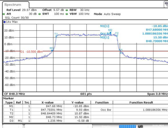
Band26-1.4MHz-QPSK-27033-6RB#0
