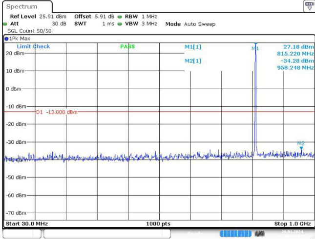
Band26-1.4MHz-QPSK-26697-1RB#0-Range1:30~1000MHz
