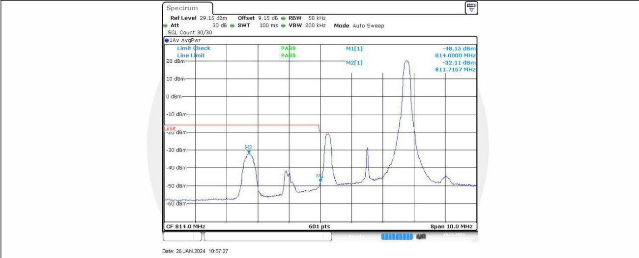
Band26-3MHz-QPSK-26705-15RB#0
