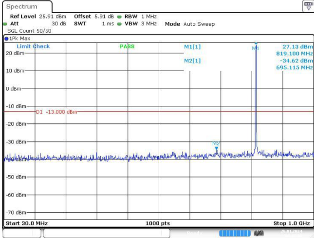
Band26-1.4MHz-QPSK-26740-1RB#0-Range1:30~1000MHz
