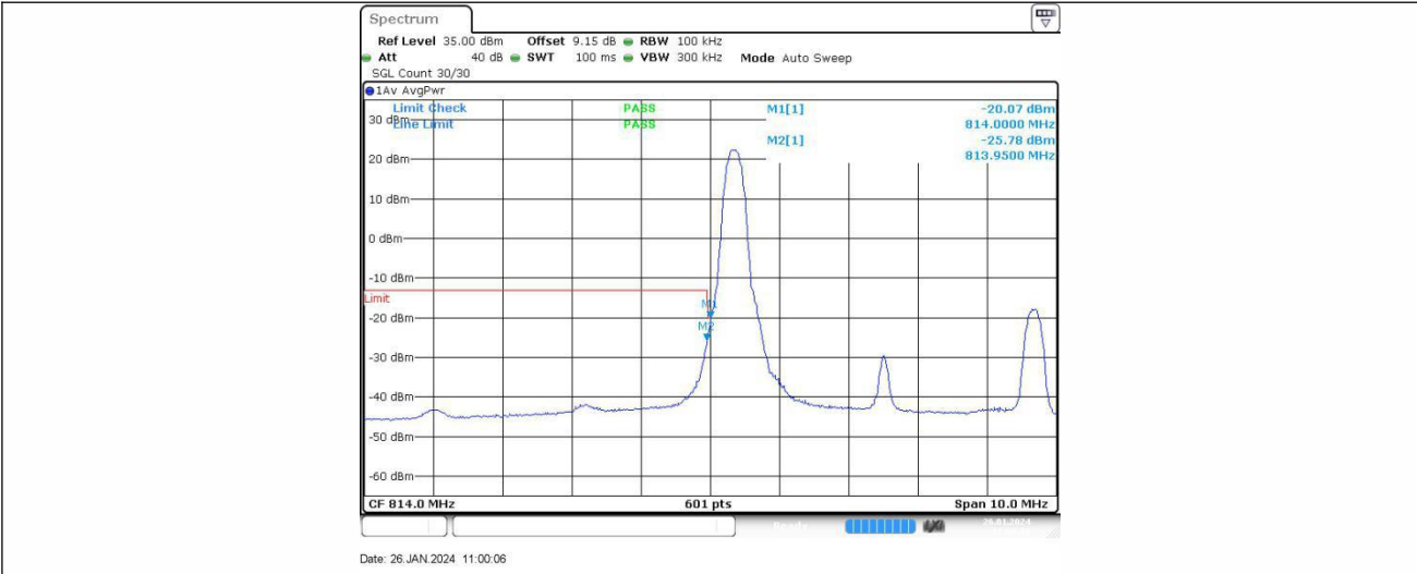
Band26-5MHz-QPSK-26715-1RB#24
