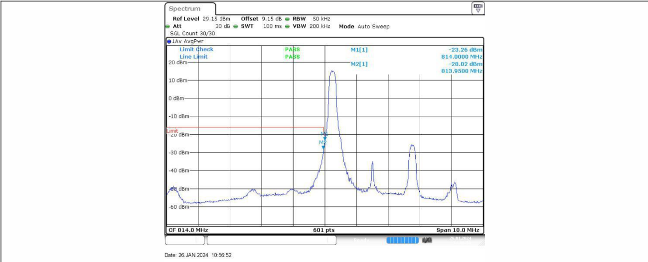
Band26-3MHz-QPSK-26705-1RB#14
