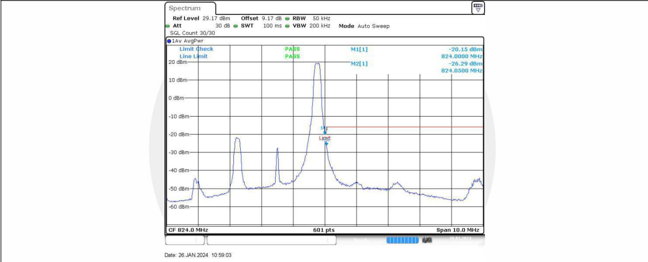
Band26-3MHz-16QAM-26775-15RB#0
