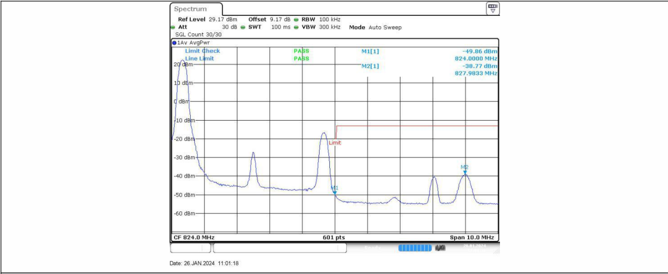
Band26-5MHz-16QAM-26765-1RB#24
