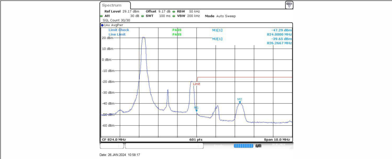
Band26-3MHz-16QAM-26775-1RB#14
