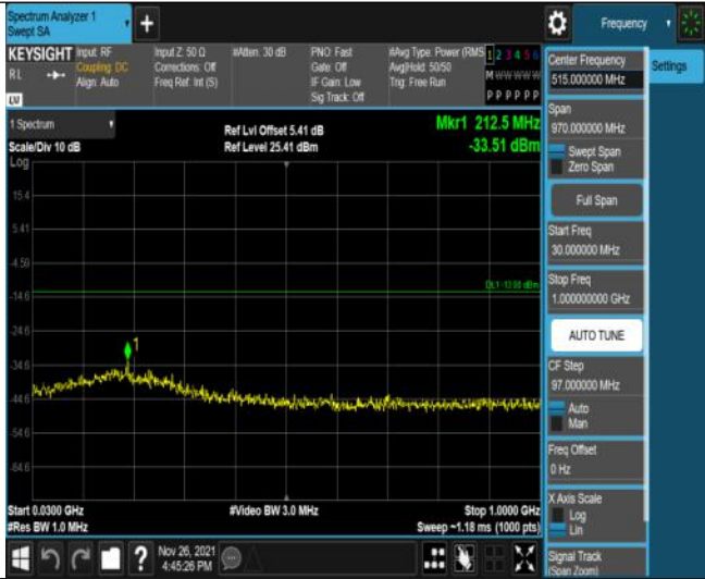
Band25-5MHz-16QAM-26365-25RB#0-Range1:30~1000MHz
