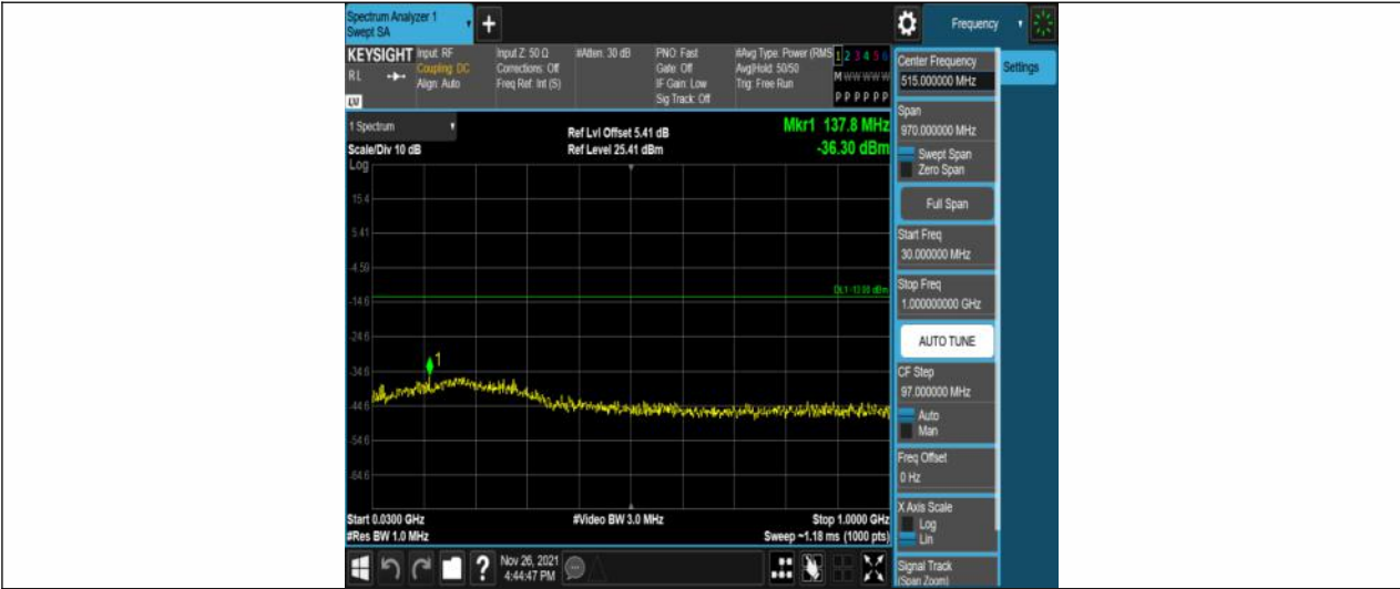
Band25-5MHz-QPSK-26365-25RB#0-Range1:30~1000MHz
