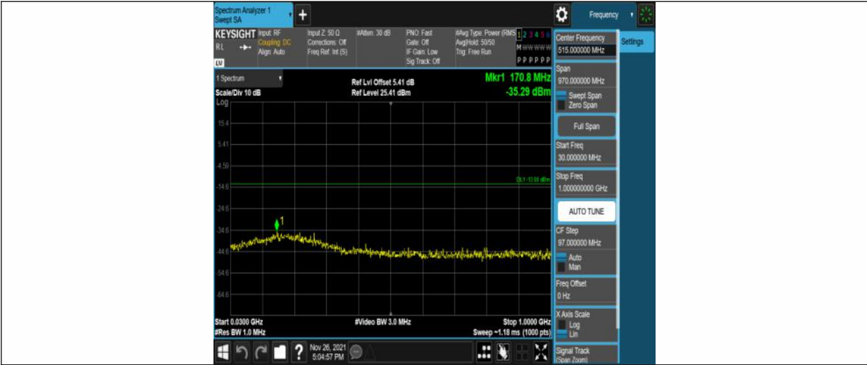
Band25-10MHz-QPSK-26090-50RB#0-Range1:30~1000MHz
