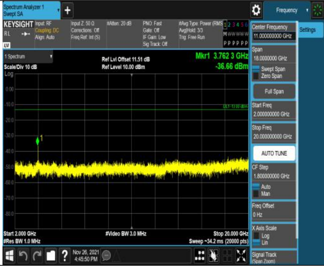
Band25-5MHz-16QAM-26365-25RB#0-Range3:2000~20000MHz
