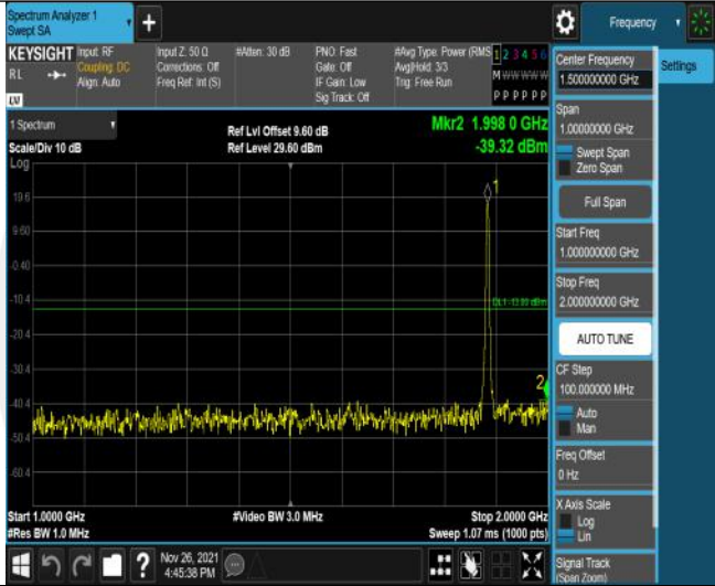
Band25-5MHz-16QAM-26365-25RB#0-Range2:1000~2000MHz
