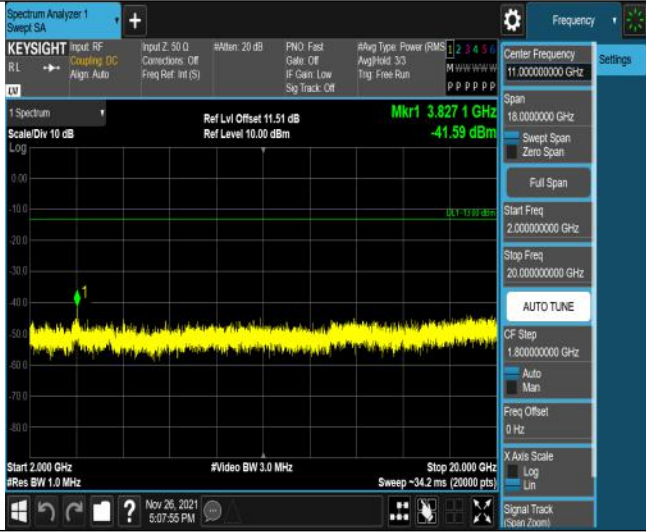
Band25-10MHz-QPSK-26640-50RB#0-Range3:2000~20000MHz
