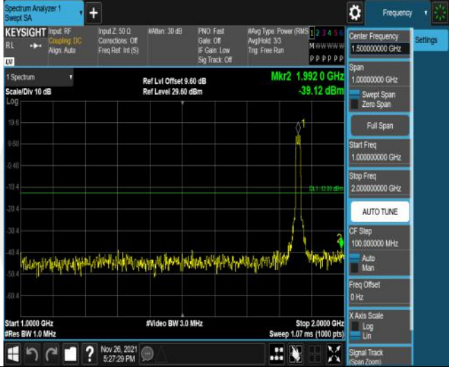
Band25-15MHz-16QAM-26115-75RB#0-Range2:1000~2000MHz
