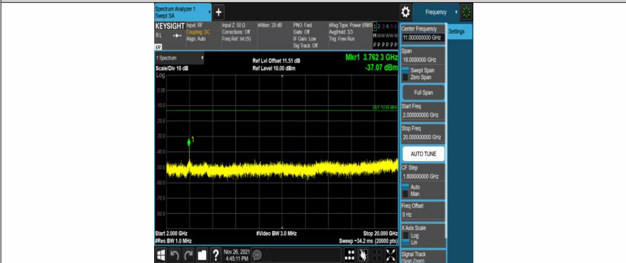
Band25-5MHz-QPSK-26365-25RB#0-Range3:2000~20000MHz
