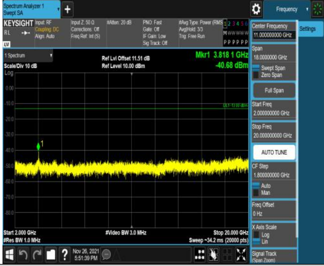
Band25-20MHz-QPSK-26590-100RB#0-Range3:2000~20000MHz
