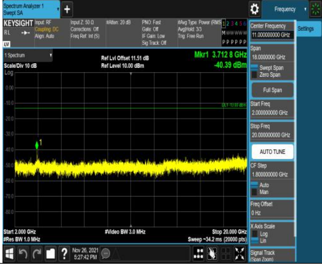
Band25-15MHz-16QAM-26115-75RB#0-Range3:2000~20000MHz
