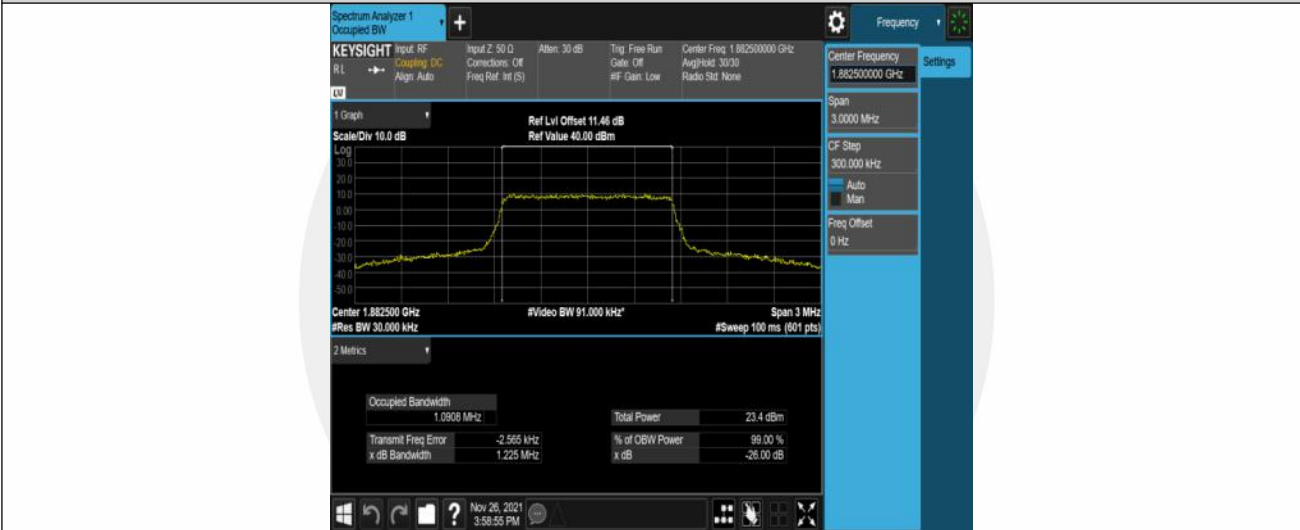
Band25-1.4MHz-16QAM-26365-6RB#0
