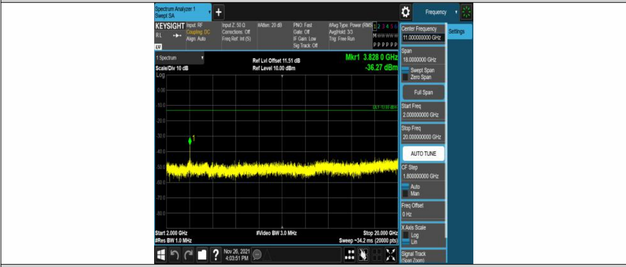
Band25-1.4MHz-QPSK-26683-6RB#0-Range3:2000~20000MHz
