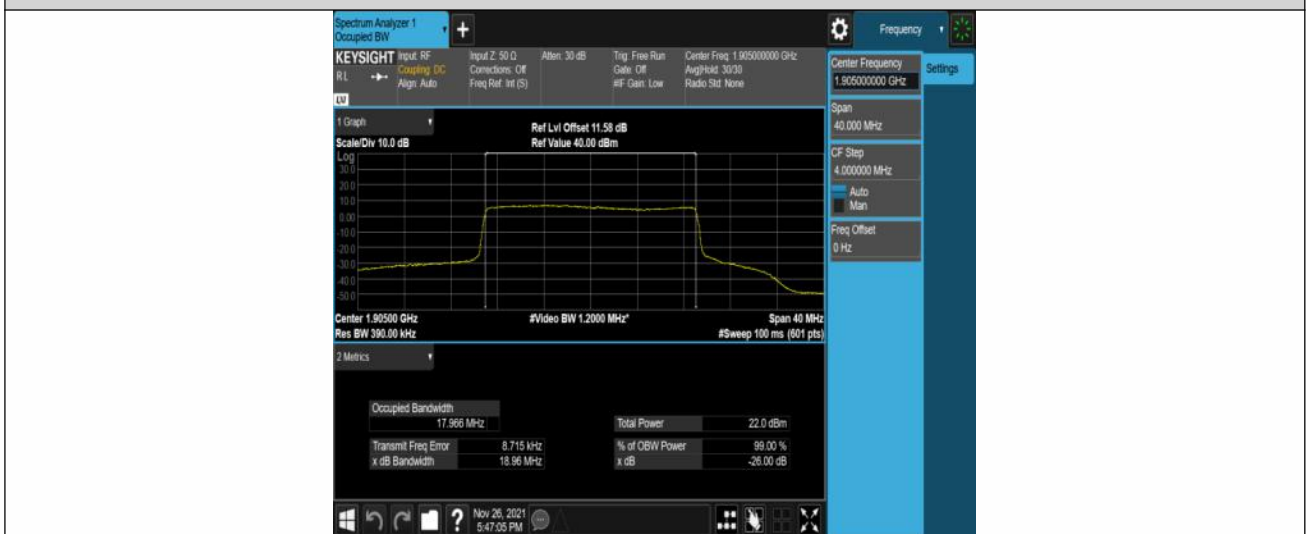
Band25-20MHz-16QAM-26590-100RB#0
