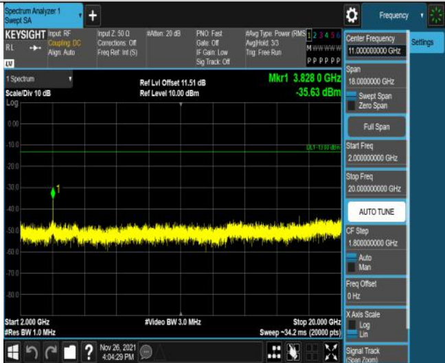
Band25-1.4MHz-16QAM-26683-6RB#0-Range3:2000~20000MHz
