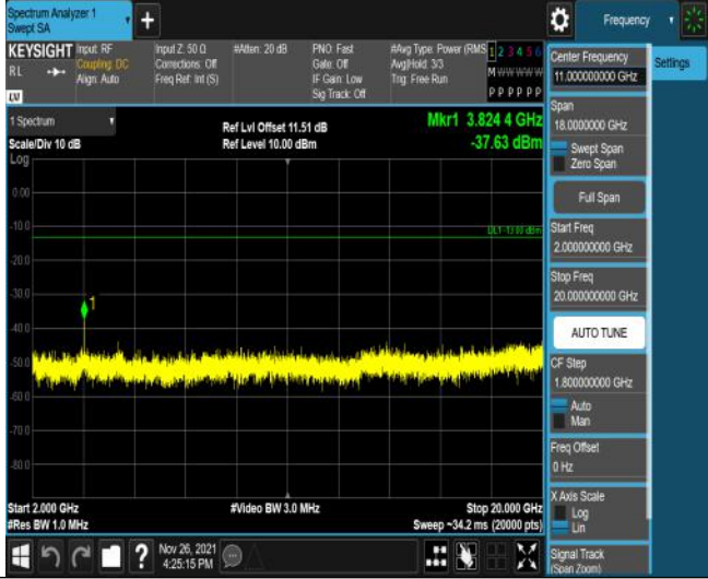
Band25-3MHz-16QAM-26675-1RB#0-Range3:2000~20000MHz
