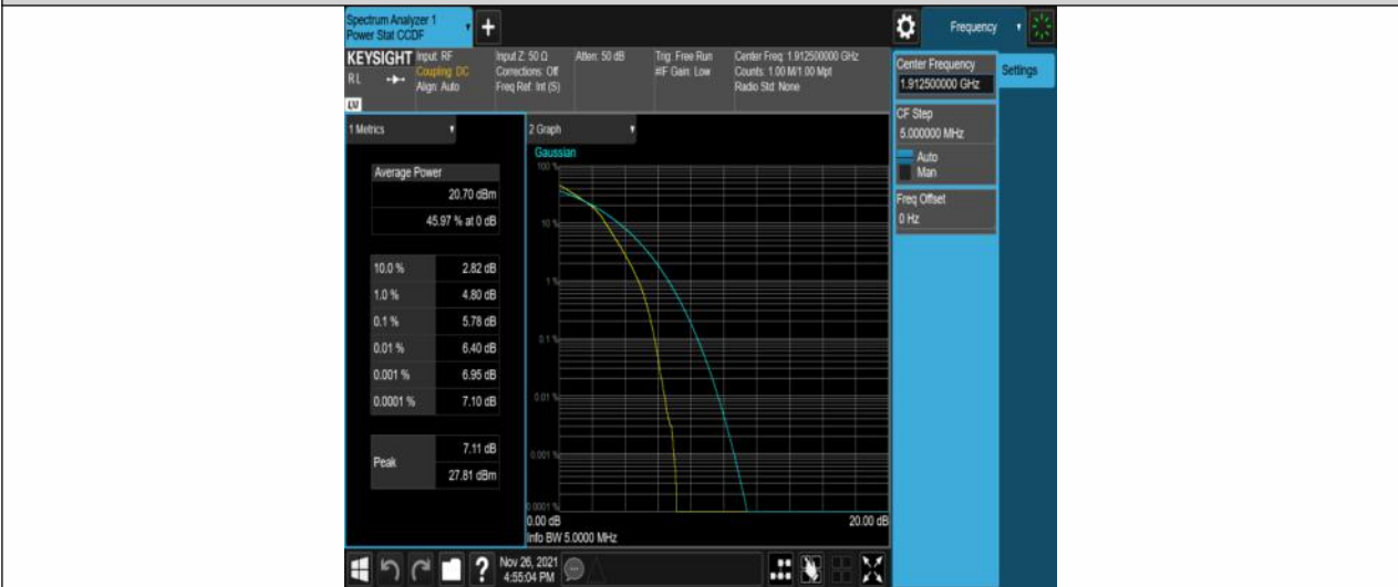
Band25-5MHz-16QAM-26665-25RB#0
