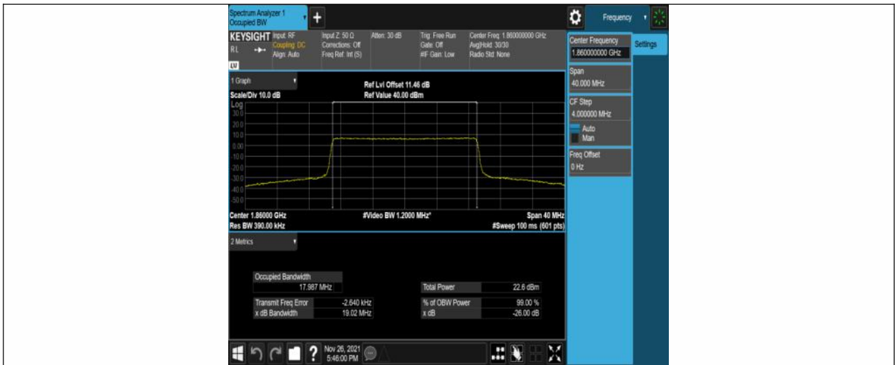
Band25-20MHz-QPSK-26140-100RB#0
