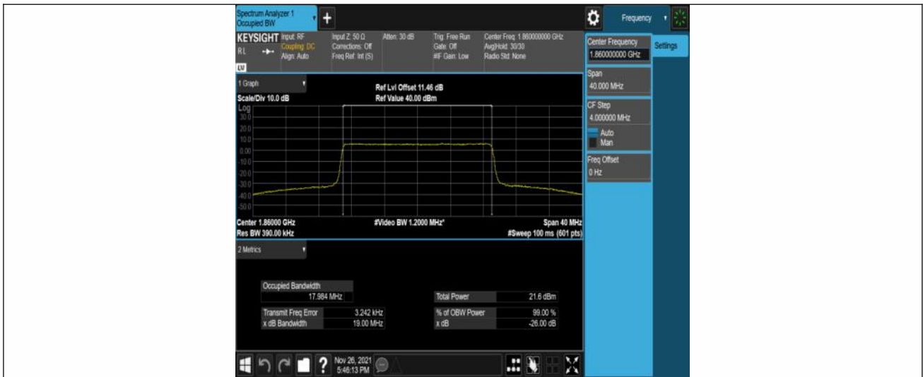
Band25-20MHz-16QAM-26140-100RB#0
