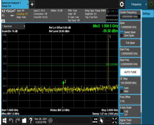
Band25-3MHz-16QAM-26675-1RB#0-Range2:1000~2000MHz
