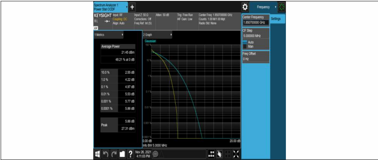
Band25-1.4MHz-QPSK-26047-6RB#0
