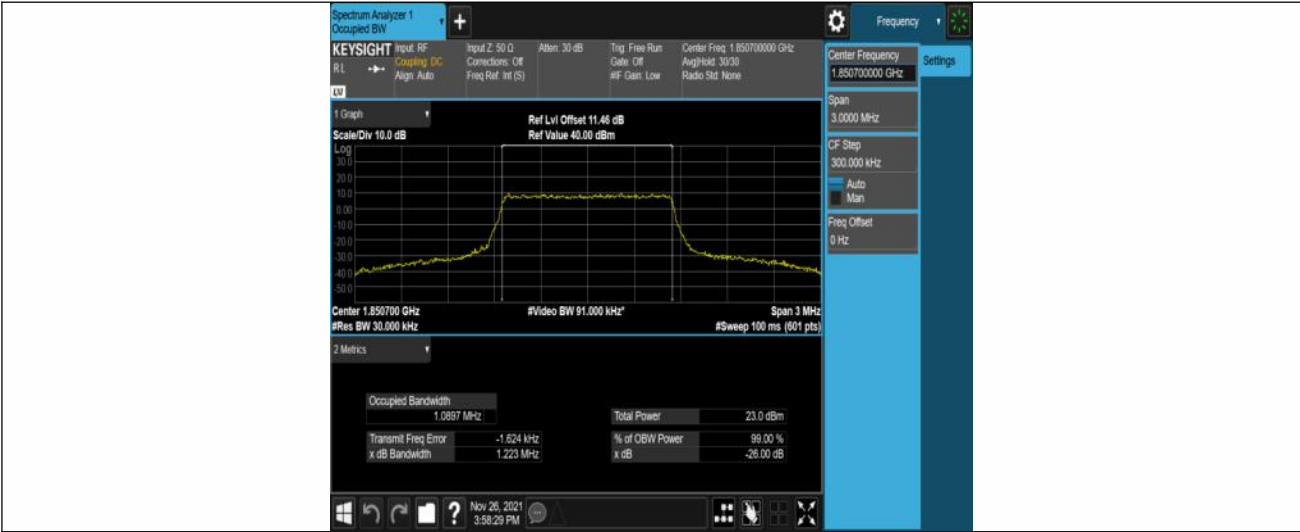
Band25-1.4MHz-16QAM-26047-6RB#0
