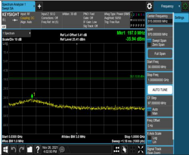
Band25-1.4MHz-16QAM-26365-6RB#0-Range1:30~1000MHz
