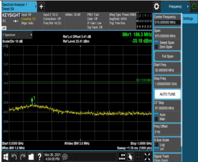
Band25-1.4MHz-16QAM-26683-6RB#0-Range1:30~1000MHz
