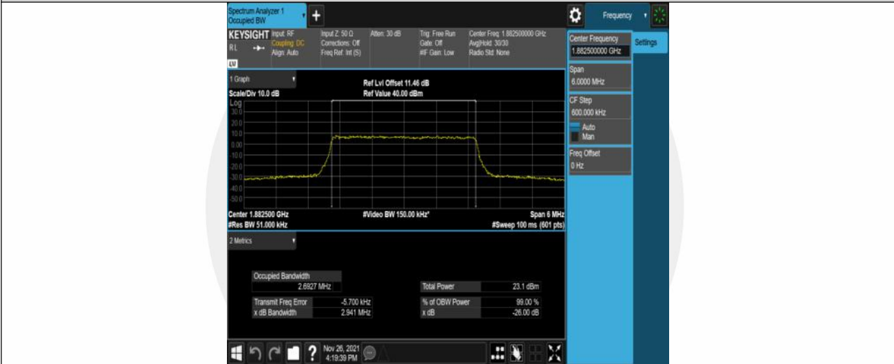
Band25-3MHz-16QAM-26365-15RB#0
