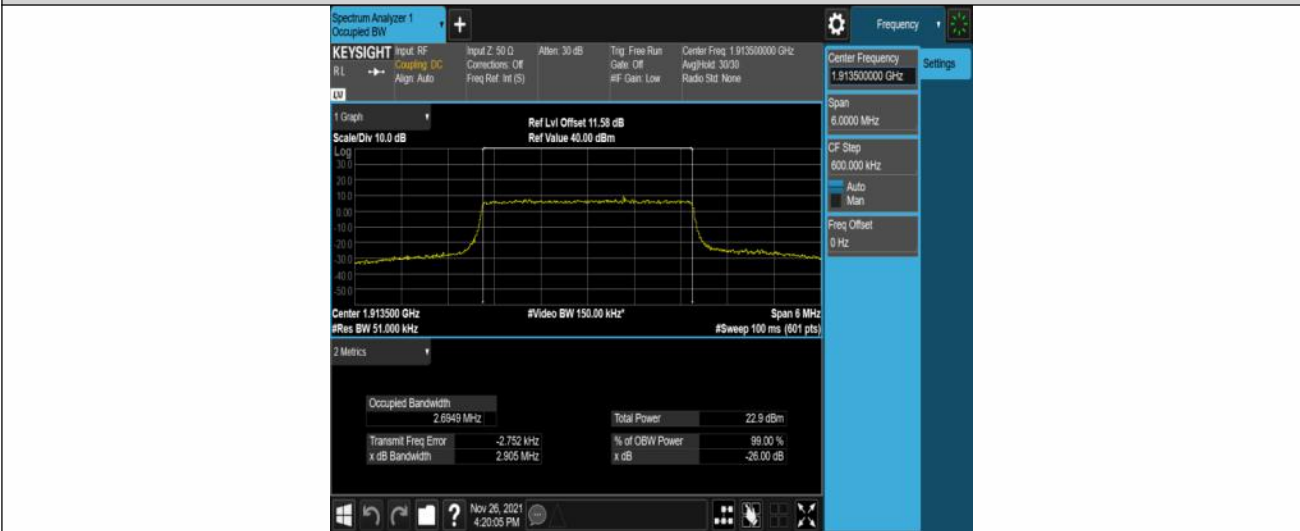
Band25-3MHz-16QAM-26675-15RB#0
