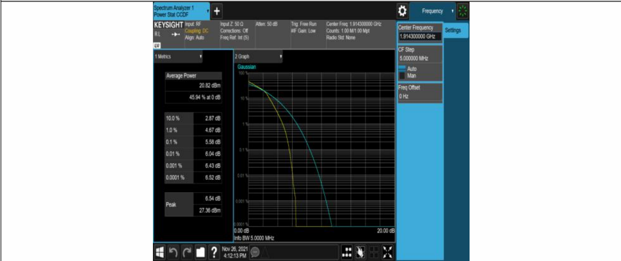
Band25-1.4MHz-16QAM-26683-6RB#0
