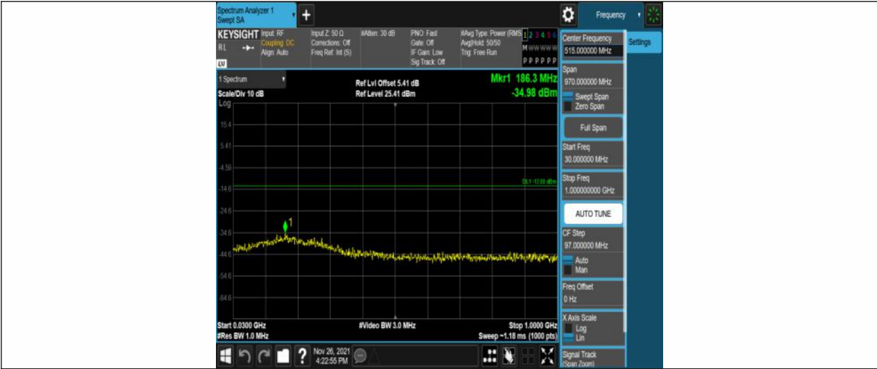
Band25-3MHz-QPSK-26365-1RB#0-Range1:30~1000MHz
