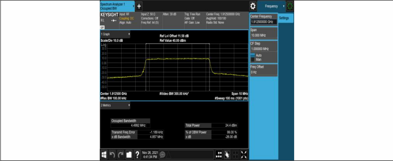
Band25-5MHz-QPSK-26665-25RB#0
