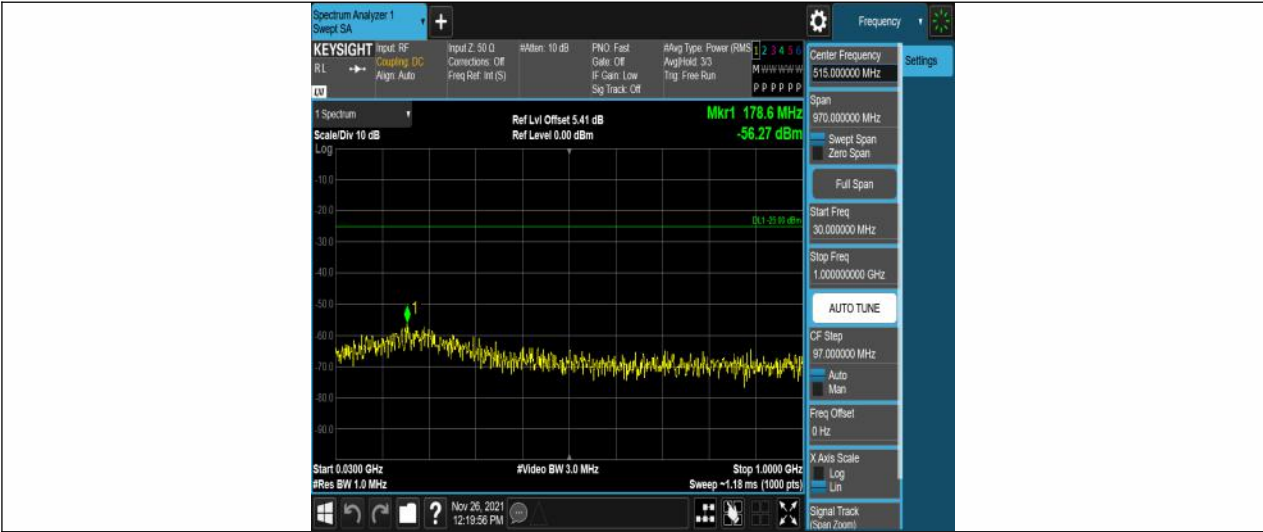
Band7-5MHz-QPSK-21100-25RB#0-Range1:30~1000MHz
