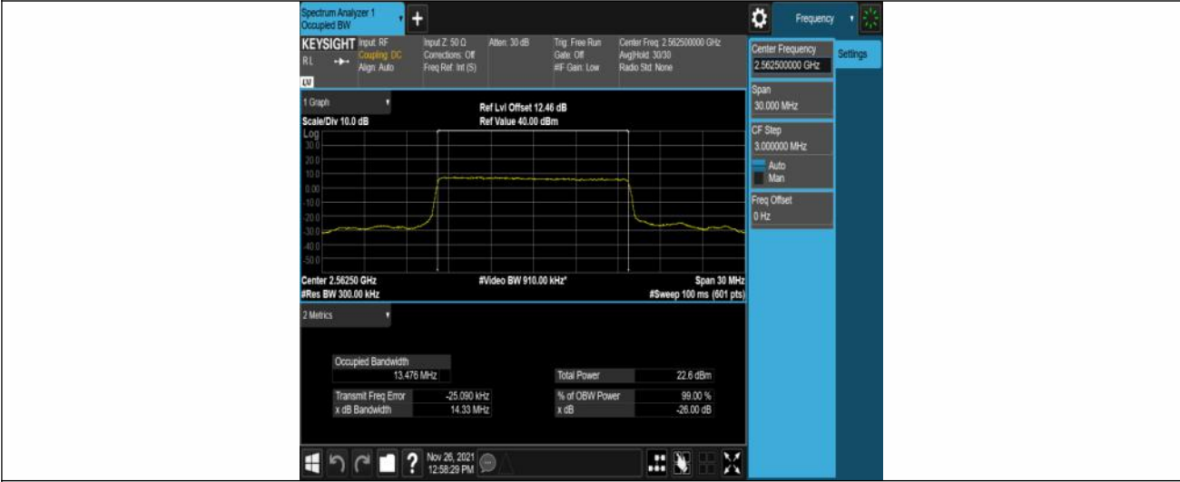
Band7-15MHz-QPSK-21375-75RB#0
