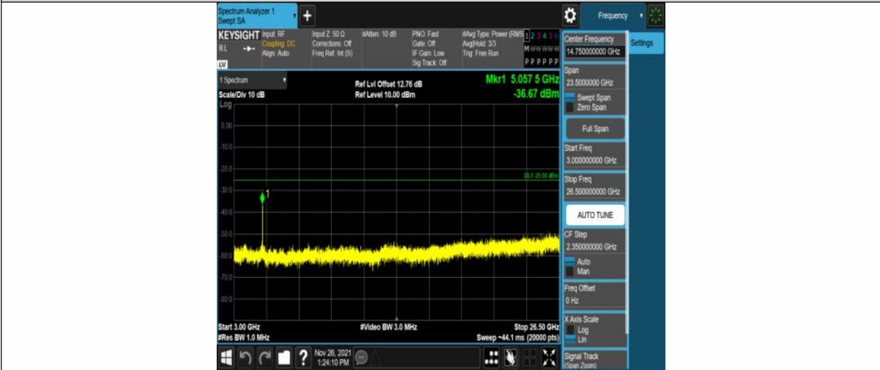
Band7-20MHz-16QAM-21100-100RB#0-Range3:3000~26500MHz
