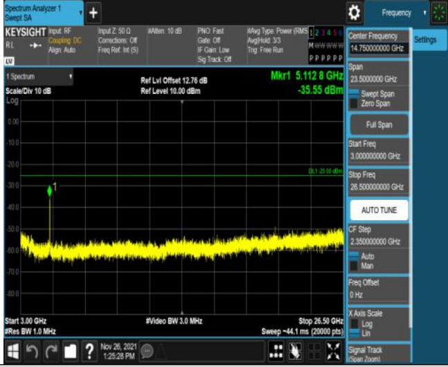
Band7-20MHz-16QAM-21350-100RB#0-Range3:3000~26500MHz
