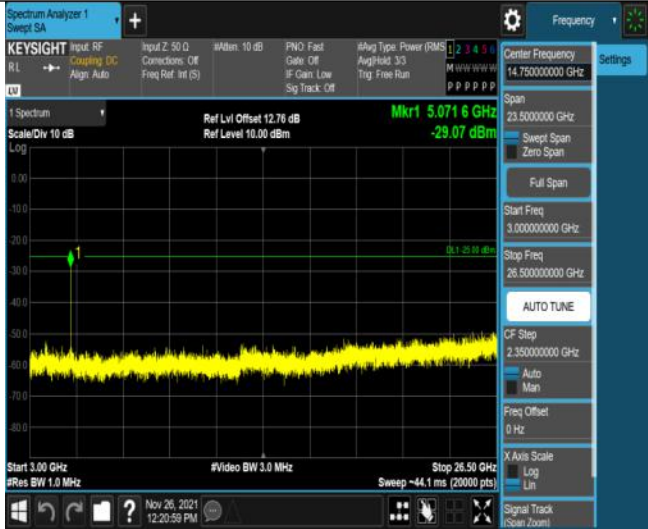
Band7-5MHz-16QAM-21100-25RB#0-Range3:3000~26500MHz
