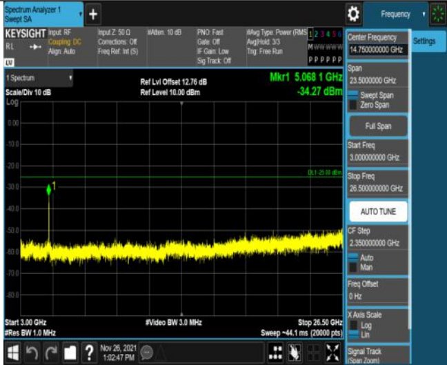
Band7-15MHz-16QAM-21100-75RB#0-Range3:3000~26500MHz
