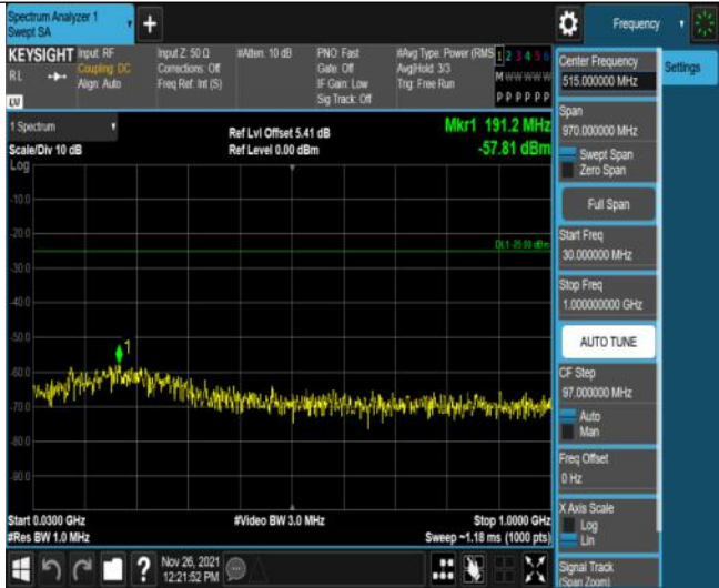
Band7-5MHz-16QAM-21425-25RB#0-Range1:30~1000MHz
