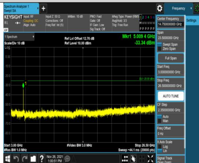
Band7-15MHz-QPSK-20825-75RB#0-Range3:3000~26500MHz
