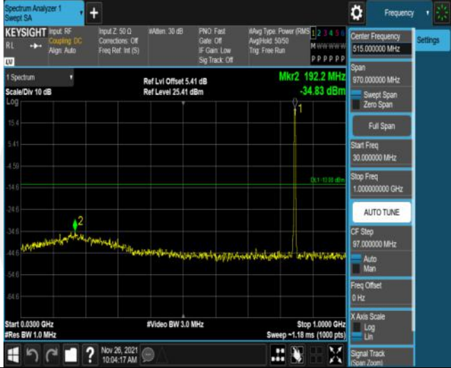
Band5-1.4MHz-QPSK-20643-6RB#0-Range1:30~1000MHz
