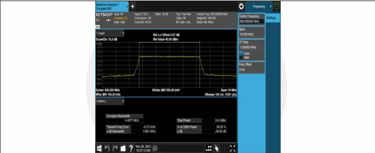
Band5-5MHz-QPSK-20525-25RB#0
