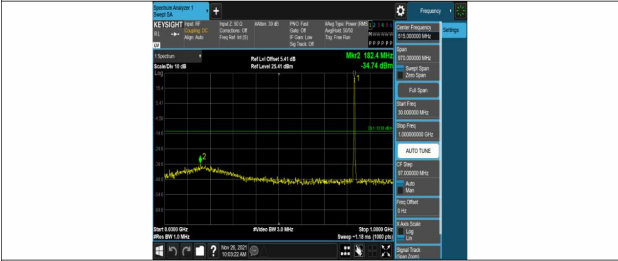
Band5-1.4MHz-QPSK-20525-6RB#0-Range1:30~1000MHz
