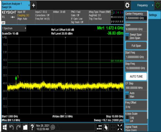
Band5-3MHz-16QAM-20525-15RB#0-Range2: 1000~10000MHz
