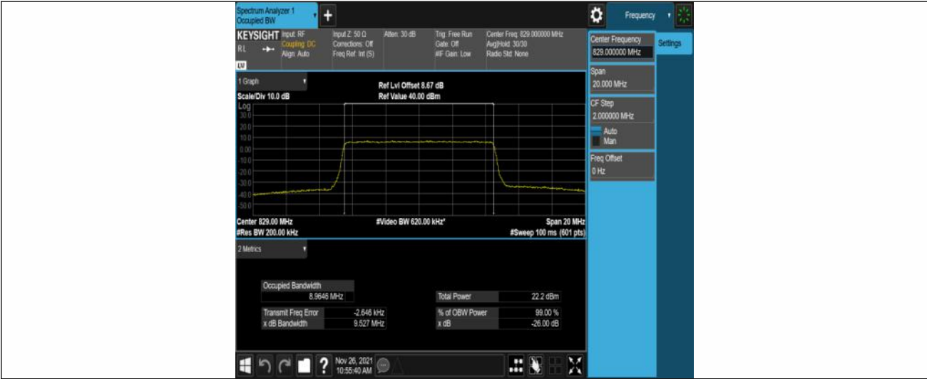
Band5-10MHz-16QAM-20450-50RB#0
