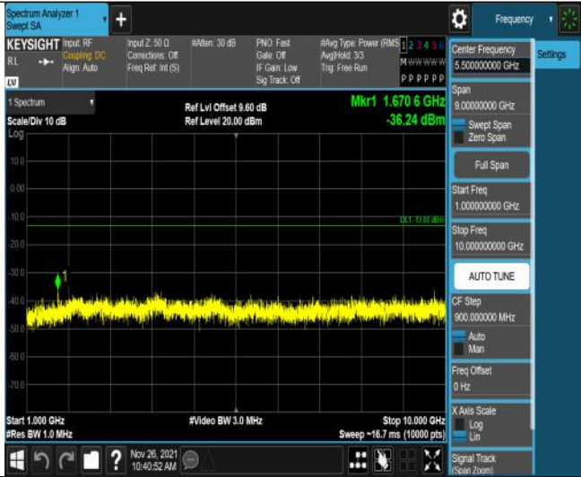
Band5-5MHz-QPSK-20525-25RB#0-Range2:1000~10000MHz
