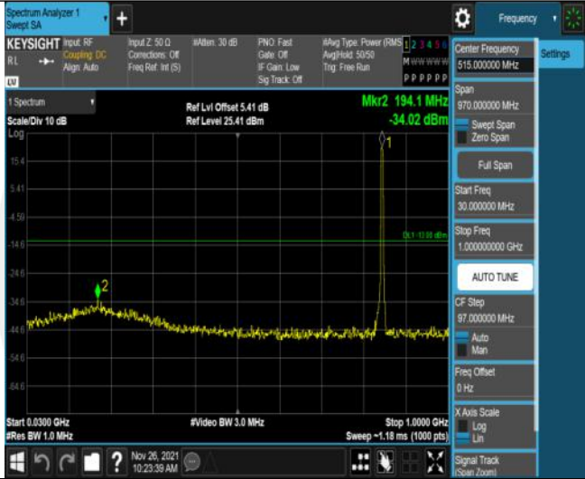
Band5-3MHz-16QAM-20635-15RB#0-Range1:30~1000MHz
