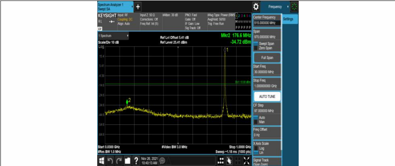
Band5-5MHz-16QAM-20425-25RB#0-Range1:30~1000MHz
