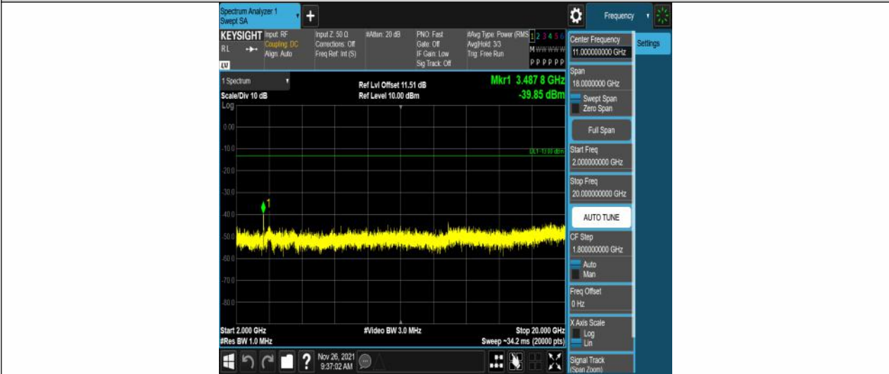
Band4-20MHz-QPSK-20300-100RB#0-Range3:2000~20000MHz
