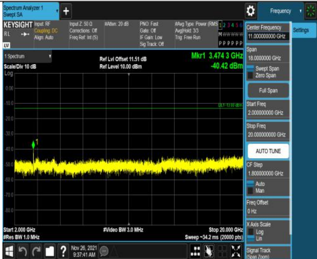
Band4-20MHz-16QAM-20300-100RB#0-Range3:2000~20000MHz
