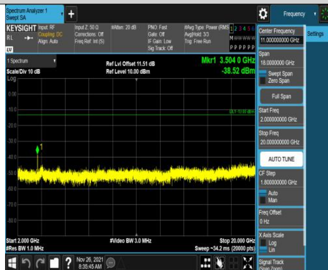
Band4-5MHz-QPSK-20375-25RB#0-Range3:2000~20000MHz
