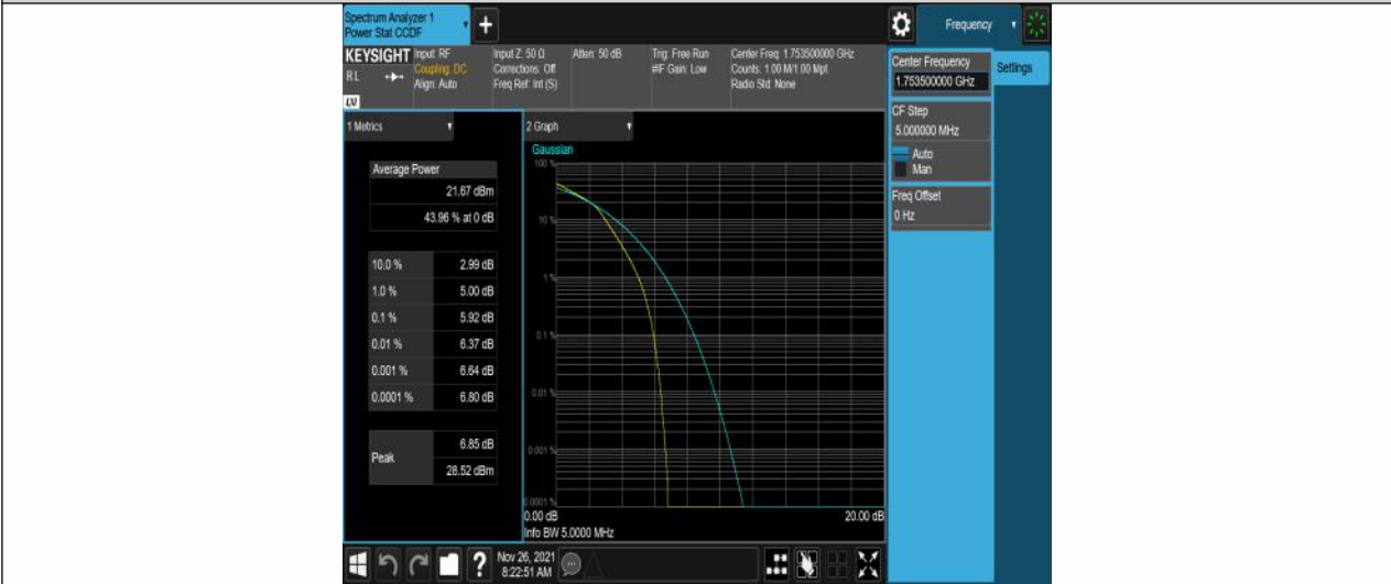
Band4-3MHz-16QAM-20385-15RB#0
