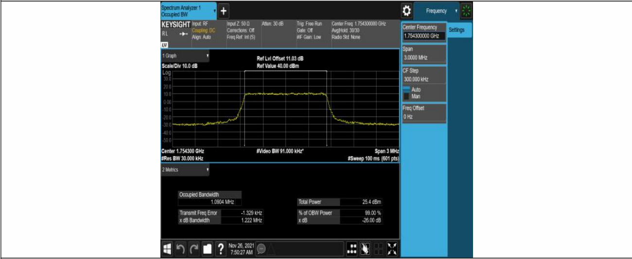
Band4-1.4MHz-QPSK-20393-6RB#0
