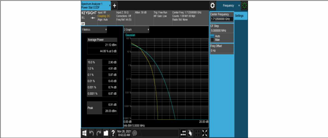
Band4-5MHz-16QAM-19975-25RB#0
