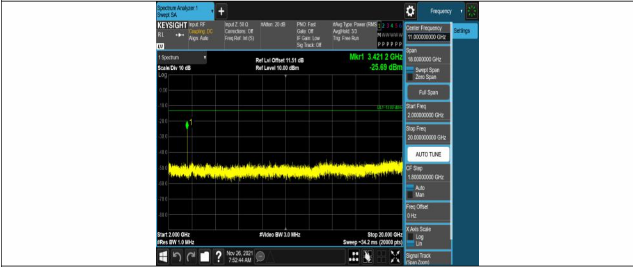
Band4-1.4MHz-QPSK-19957-6RB#0-Range3:2000~20000MHz
