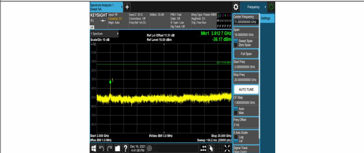
Band2-5MHz-QPSK-19175-25RB#0-Range3:2000~20000MHz
