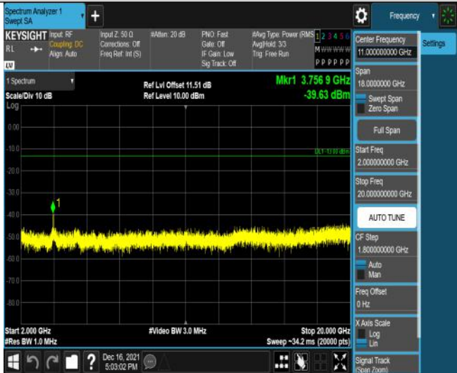
Band2-20MHz-16QAM-18900-100RB#0-Range3:2000~20000MHz
