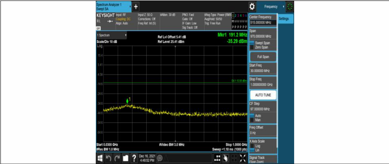
Band2-10MHz-16QAM-19150-50RB#0-Range1:30~1000MHz
