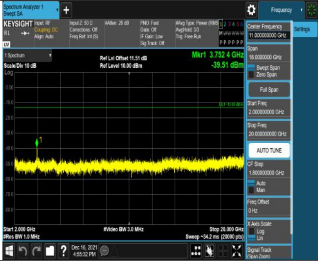
Band2-15MHz-16QAM-18900-75RB#0-Range3:2000~20000MHz
