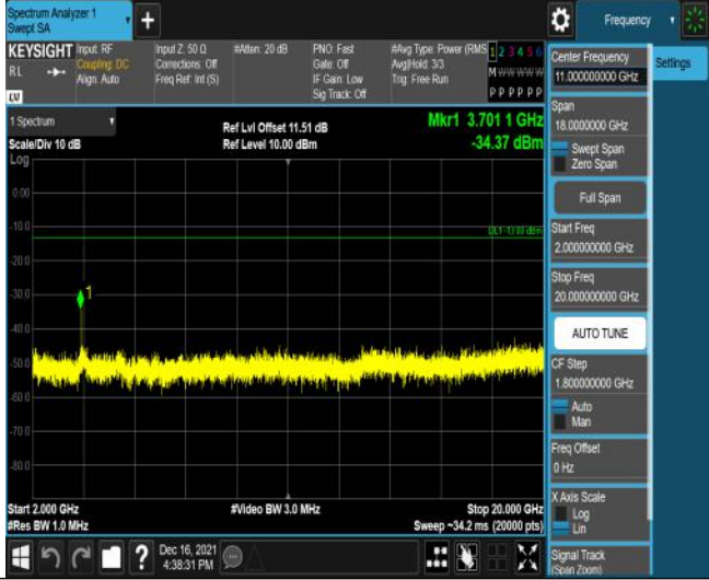
Band2-5MHz-QPSK-18625-25RB#0-Range3:2000~20000MHz
