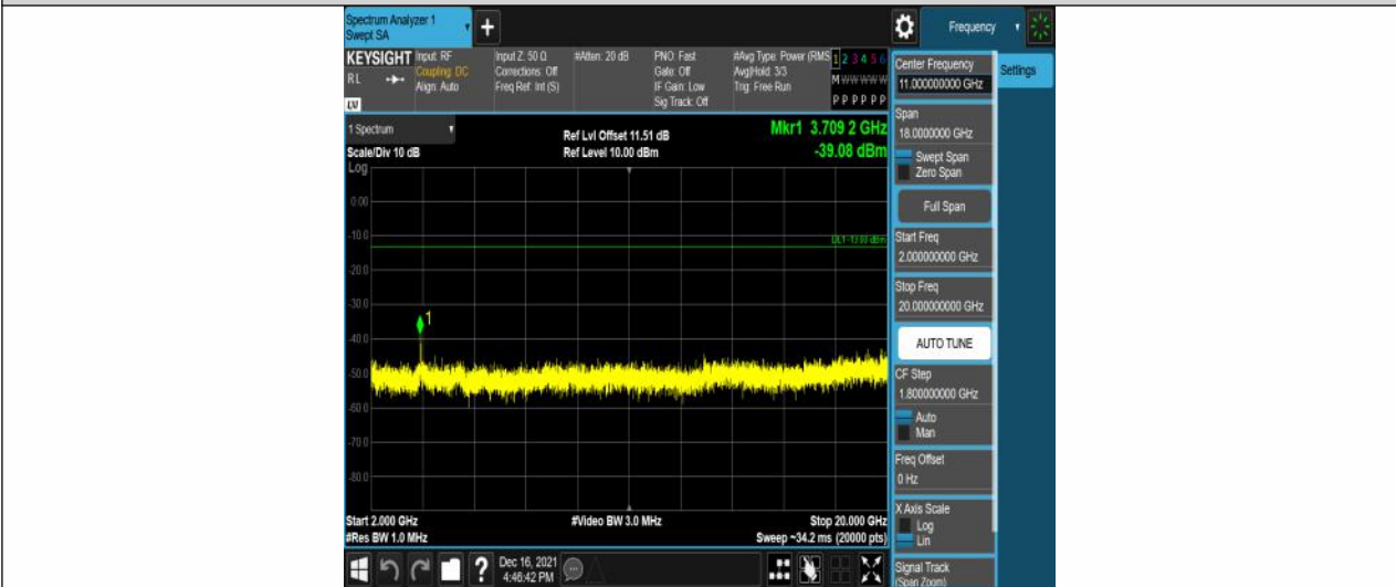
Band2-10MHz-16QAM-18650-50RB#0-Range3:2000~20000MHz
