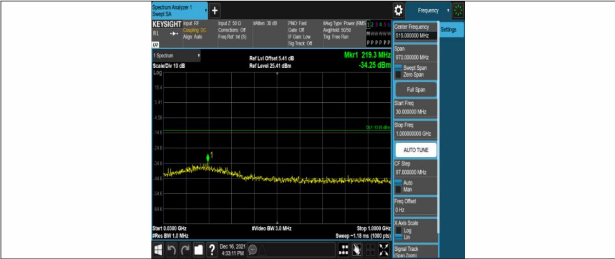
Band2-3MHz-16QAM-19185-15RB#0-Range1:30~1000MHz
