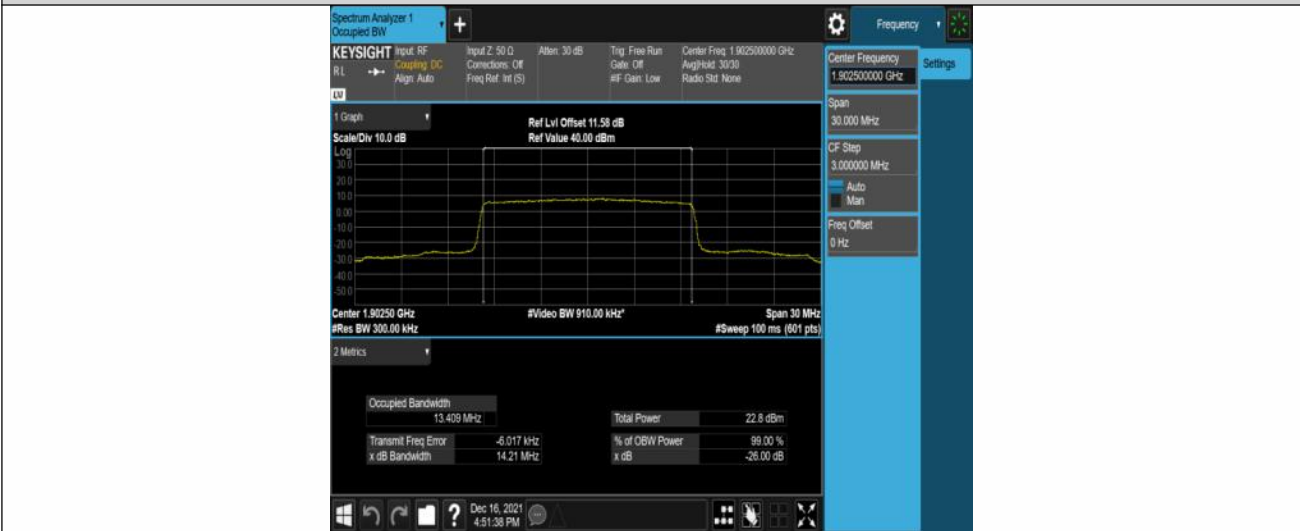
Band2-15MHz-16QAM-19125-75RB#0
