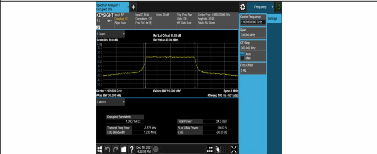
Band2-1.4MHz-16QAM-19193-6RB#0
