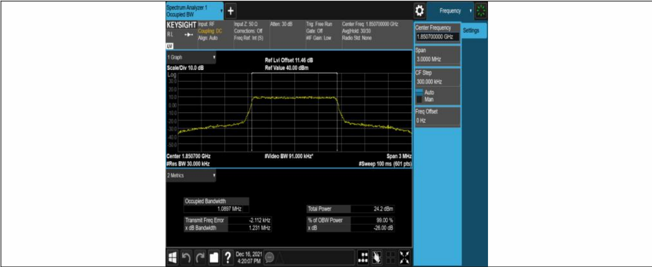
Band2-1.4MHz-16QAM-18507-6RB#0
