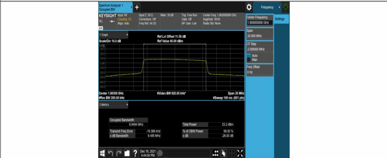
Band2-10MHz-16QAM-19150-50RB#0
