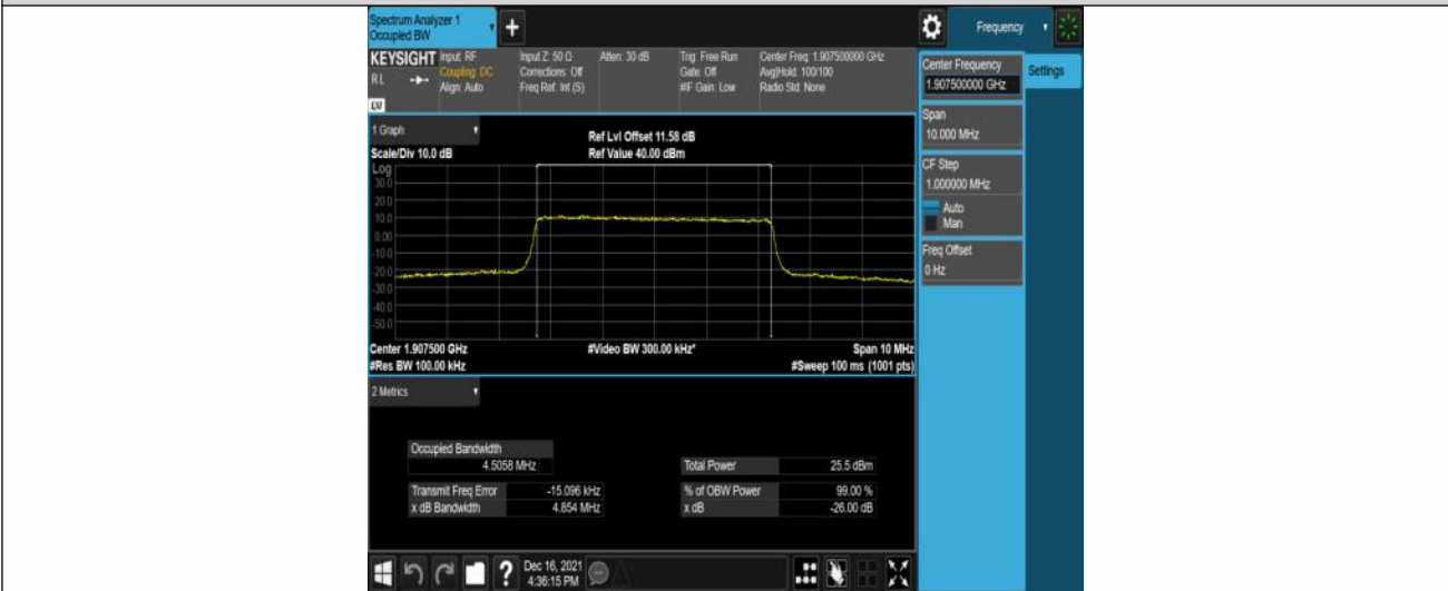
Band2-5MHz-QPSK-19175-25RB#0
