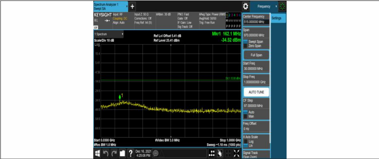
Band2-1.4MHz-QPSK-19193-6RB#0-Range1:30~1000MHz
