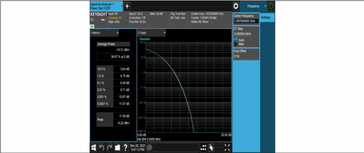
Band2-15MHz-QPSK-18675-75RB#0
