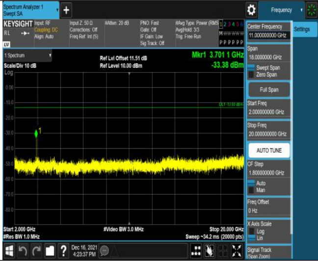
Band2-1.4MHz-16QAM-18607-6RB#0-Range3:2000~20000MHz
