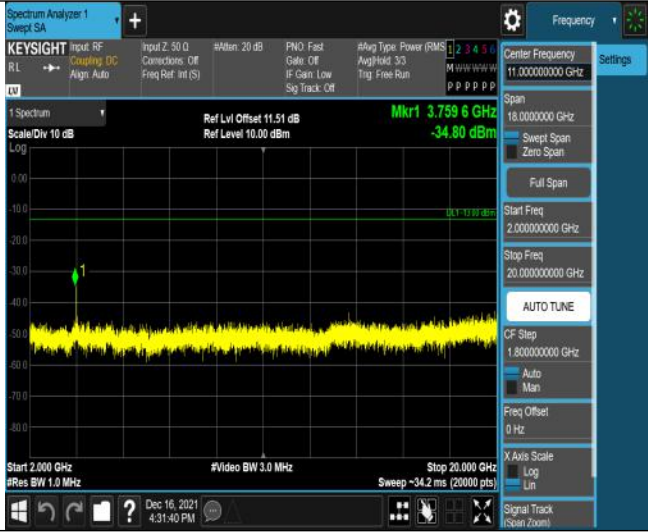
Band2-3MHz-QPSK-18900-15RB#0-Range3:2000~20000MHz
