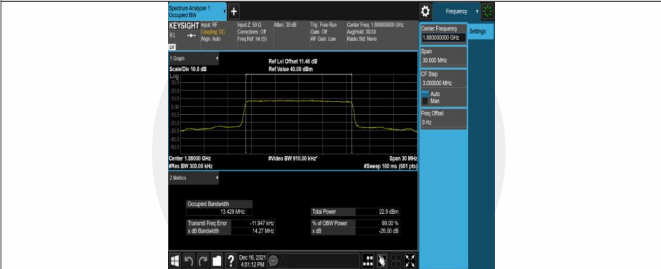
Band2-15MHz-16QAM-18900-75RB#0
