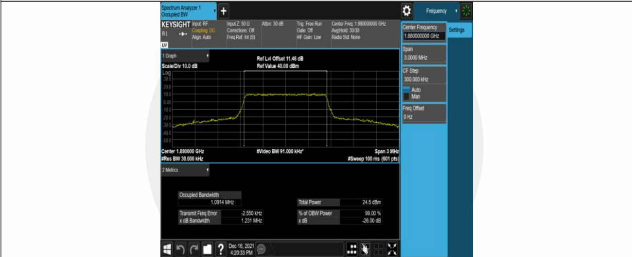
Band2-1.4MHz-16QAM-18900-6RB#0
