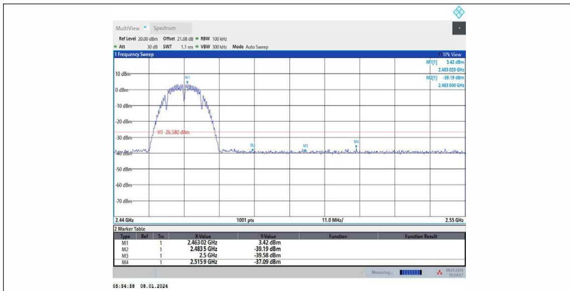
11B_Ant2_High_2462
