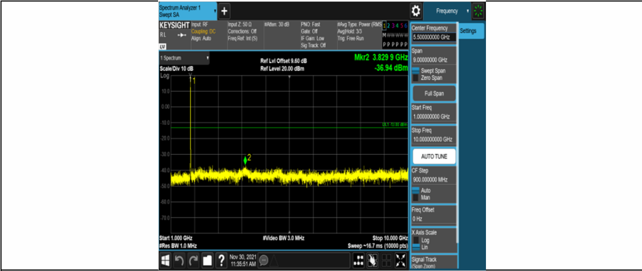
Band66-5MHz-16QAM-132322-25RB#0-Range2:1000~10000MHz
