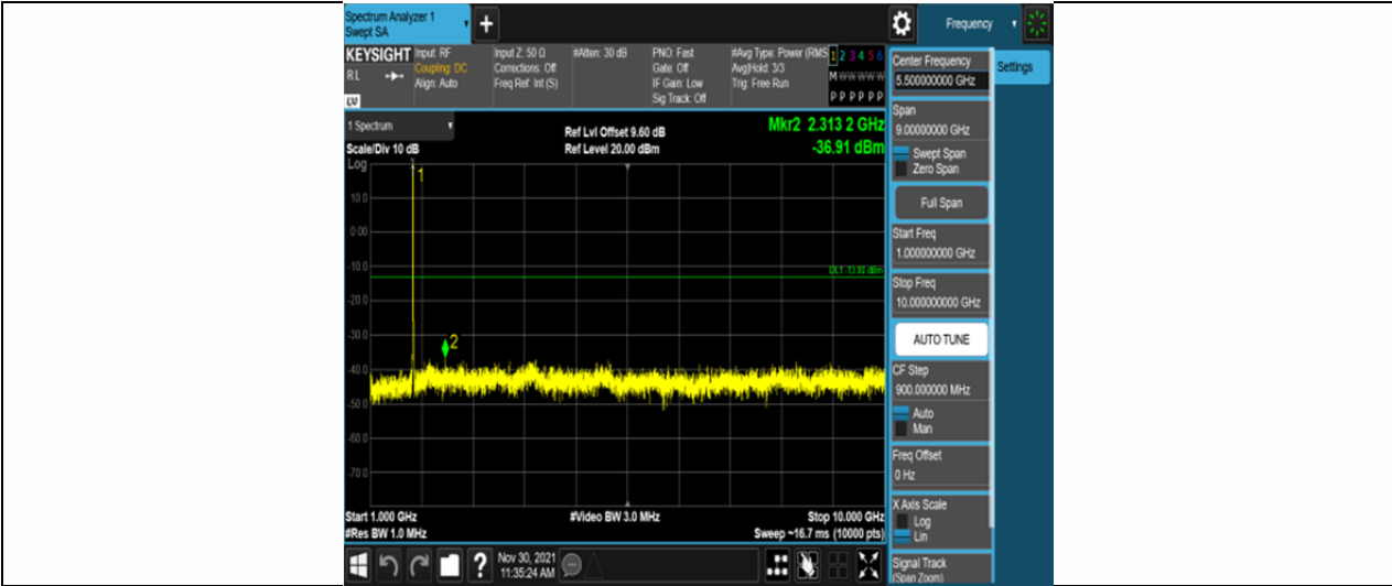
Band66-5MHz-QPSK-132322-25RB#0-Range2:1000~10000MHz
