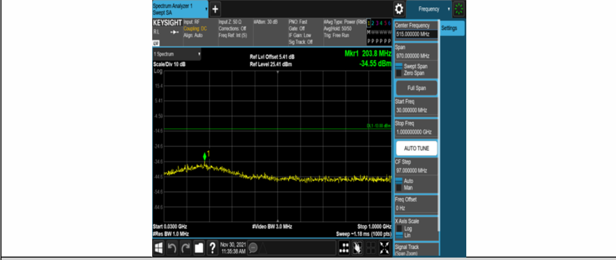
Band66-5MHz-16QAM-132322-25RB#0-Range1:30~1000MHz
