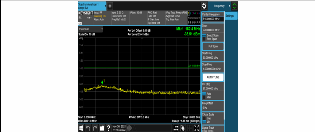
Band66-3MHz-QPSK-132322-15RB#0-Range1:30~1000MHz
