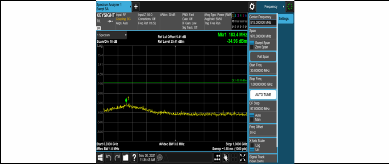
Band66-5MHz-16QAM-131997-25RB#0-Range1:30~1000MHz
