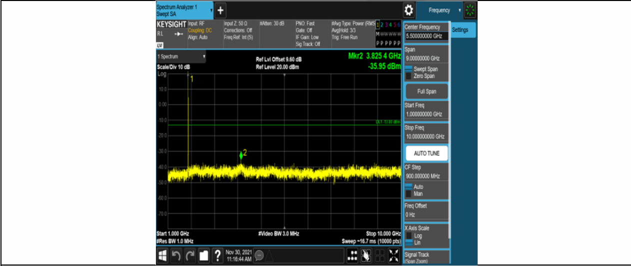
Band66-3MHz-QPSK-132657-15RB#0-Range2:1000~10000MHz
