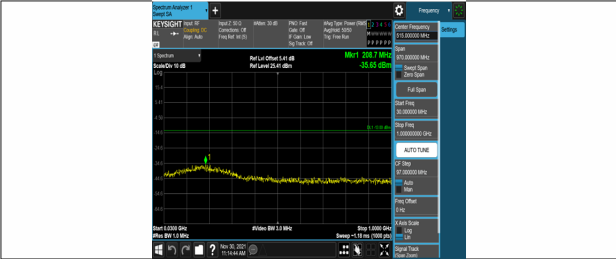
Band66-3MHz-QPSK-131987-15RB#0-Range1:30~1000MHz
