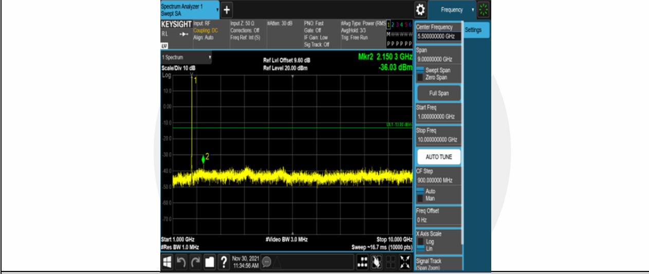
Band66-5MHz-16QAM-131997-25RB#0-Range2:1000~10000MHz
