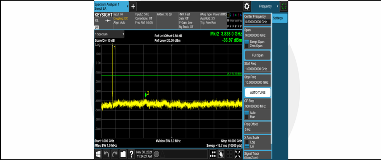
Band66-5MHz-QPSK-131997-25RB#0-Range2:1000~10000MHz
