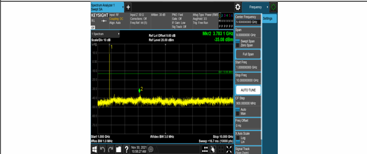
Band66-1.4MHz-QPSK-132665-6RB#0-Range2:1000~10000MHz
