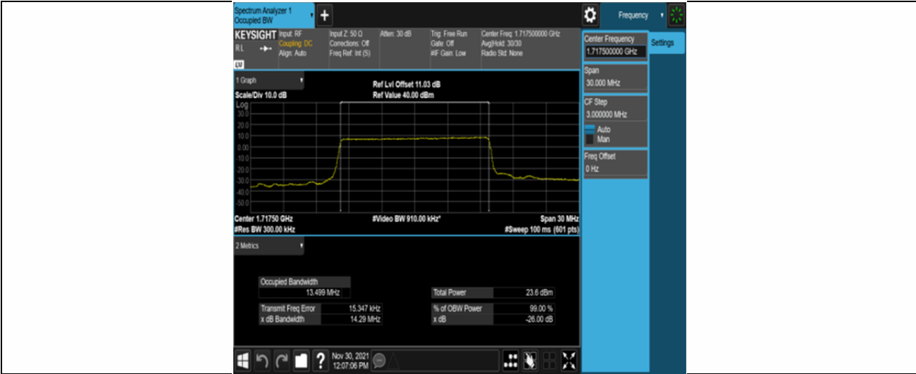
Band66-15MHz-QPSK-132047-75RB#0
