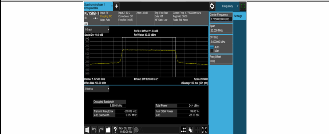
Band66-10MHz-QPSK-132622-50RB#0
