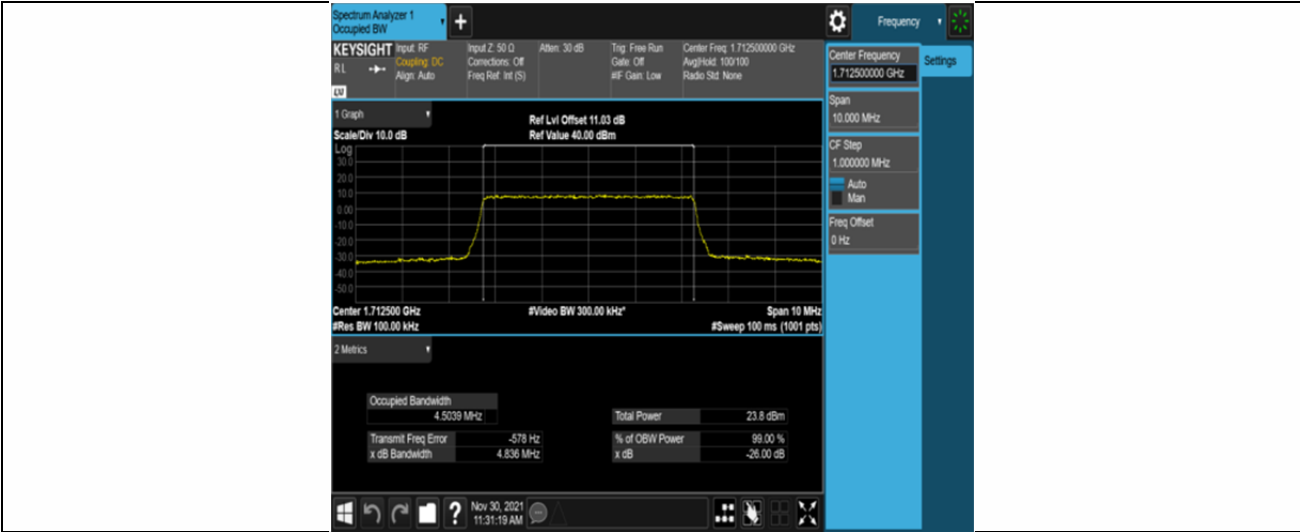
Band66-5MHz-16QAM-131997-25RB#0
