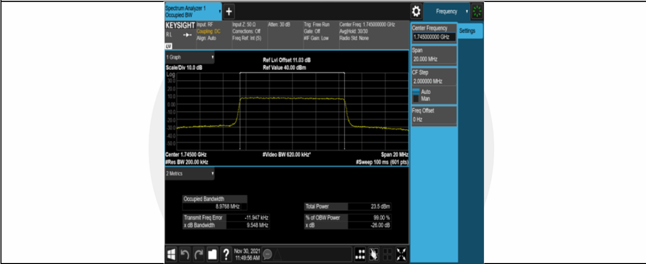
Band66-10MHz-16QAM-132322-50RB#0
