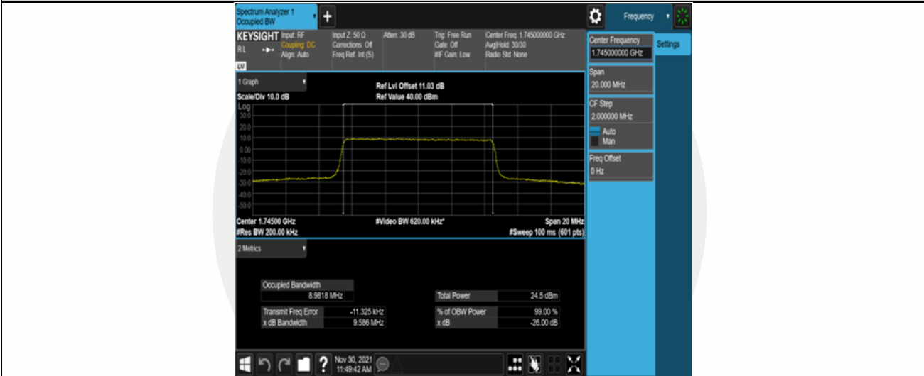
Band66-10MHz-QPSK-132322-50RB#0
