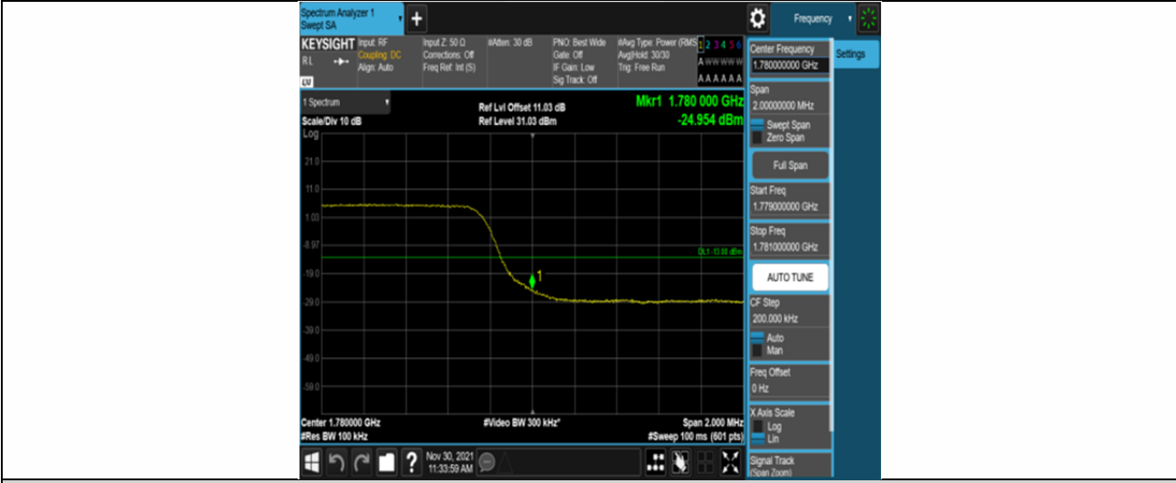
Band66-5MHz-16QAM-132647-25RB#0
