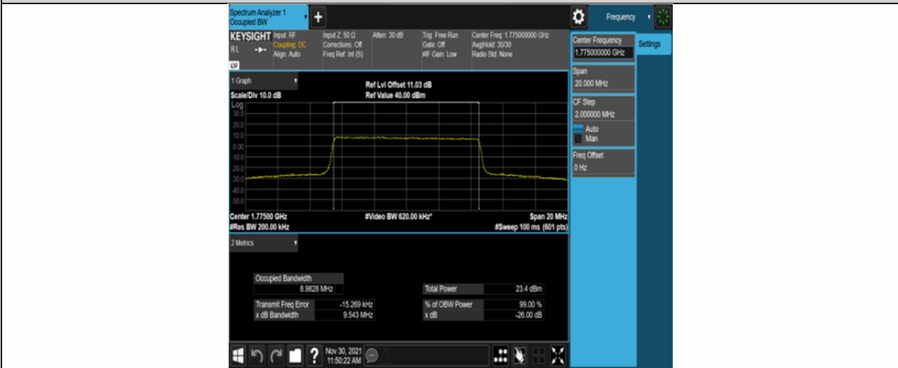
Band66-10MHz-16QAM-132622-50RB#0
