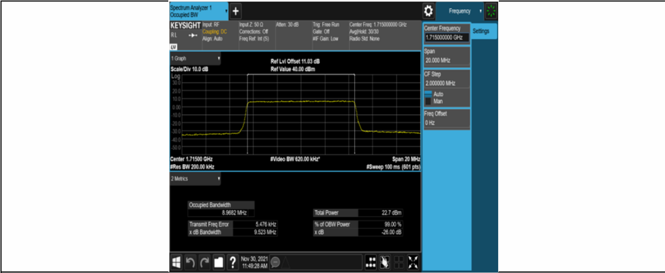
Band66-10MHz-16QAM-132022-50RB#0
