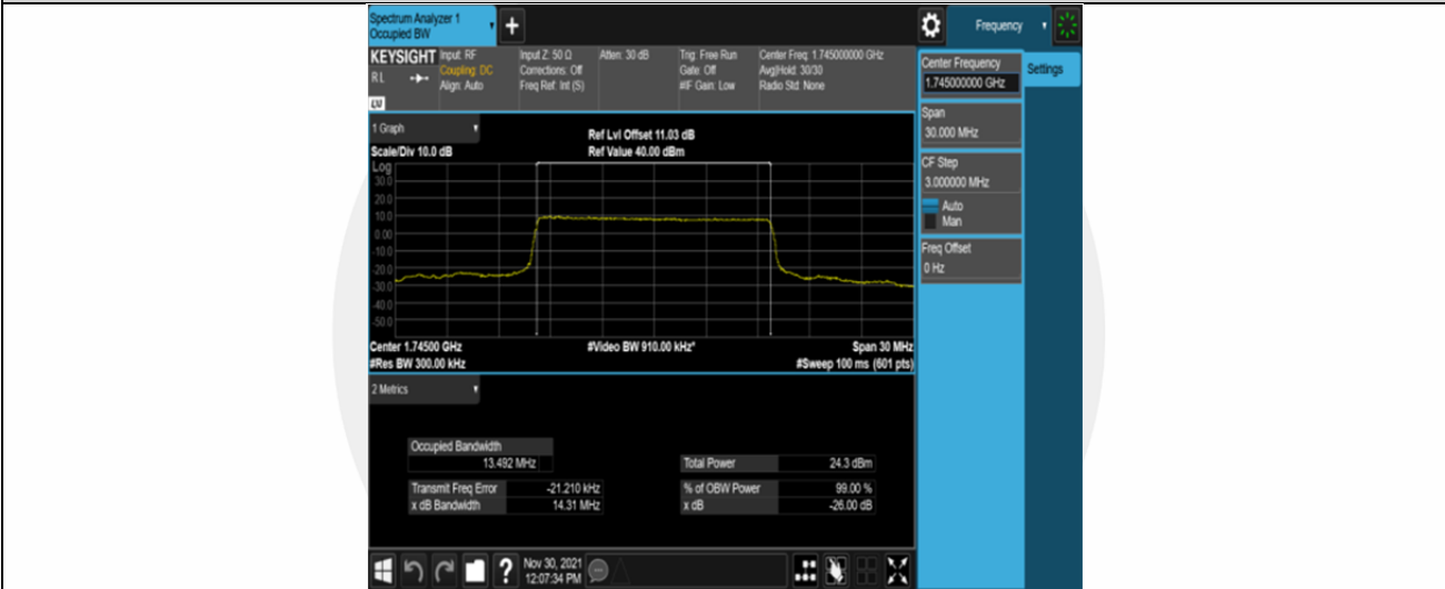
Band66-15MHz-QPSK-132322-75RB#0
