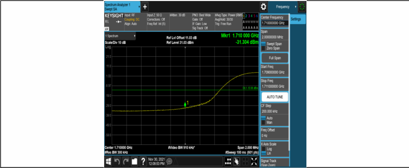
Band66-15MHz-16QAM-132047-75RB#0
