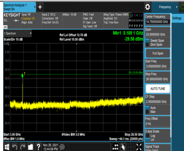
Band41-10MHz-16QAM-40620-50RB#0-Range3:3000~26500MHz
