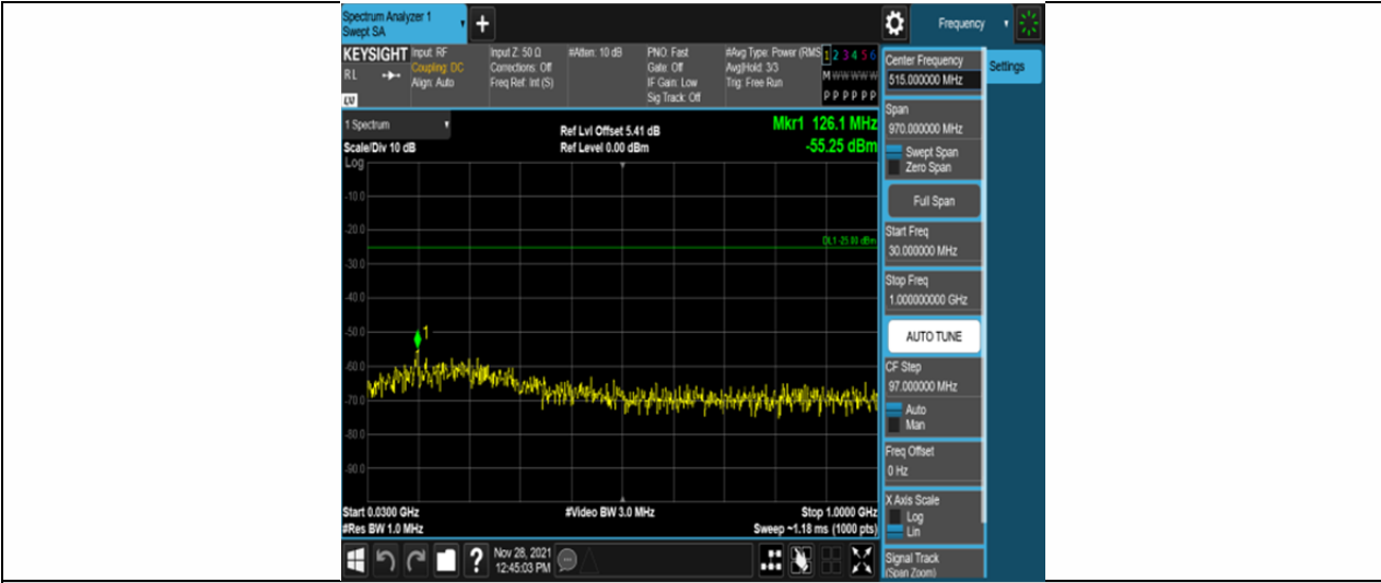
Band41-10MHz-16QAM-41540-50RB#0-Range1:30~1000MHz
