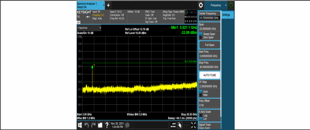
Band41-20MHz-QPSK-39750-100RB#0-Range3:3000~26500MHz
