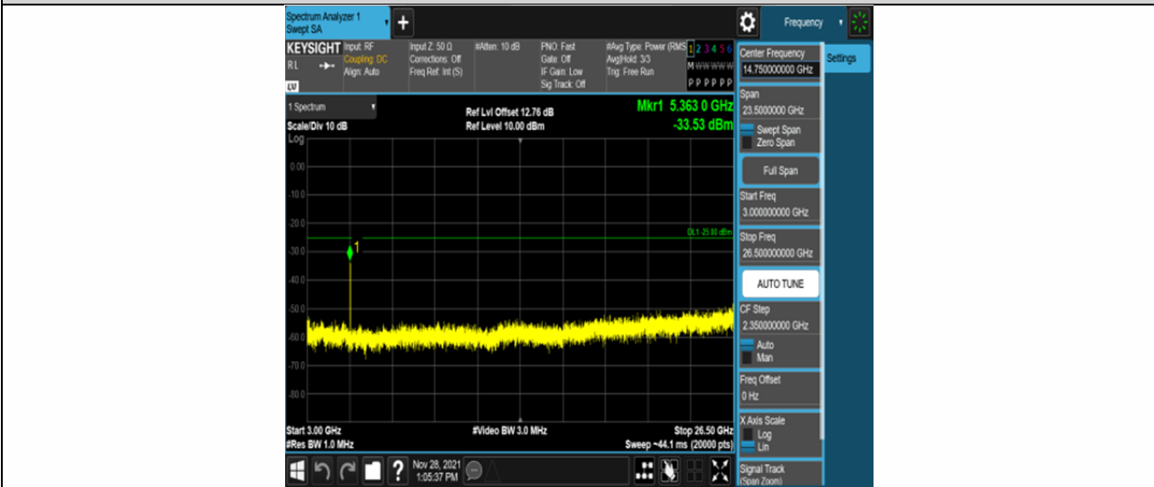
Band41-15MHz-QPSK-41515-75RB#0-Range3:3000~26500MHz
