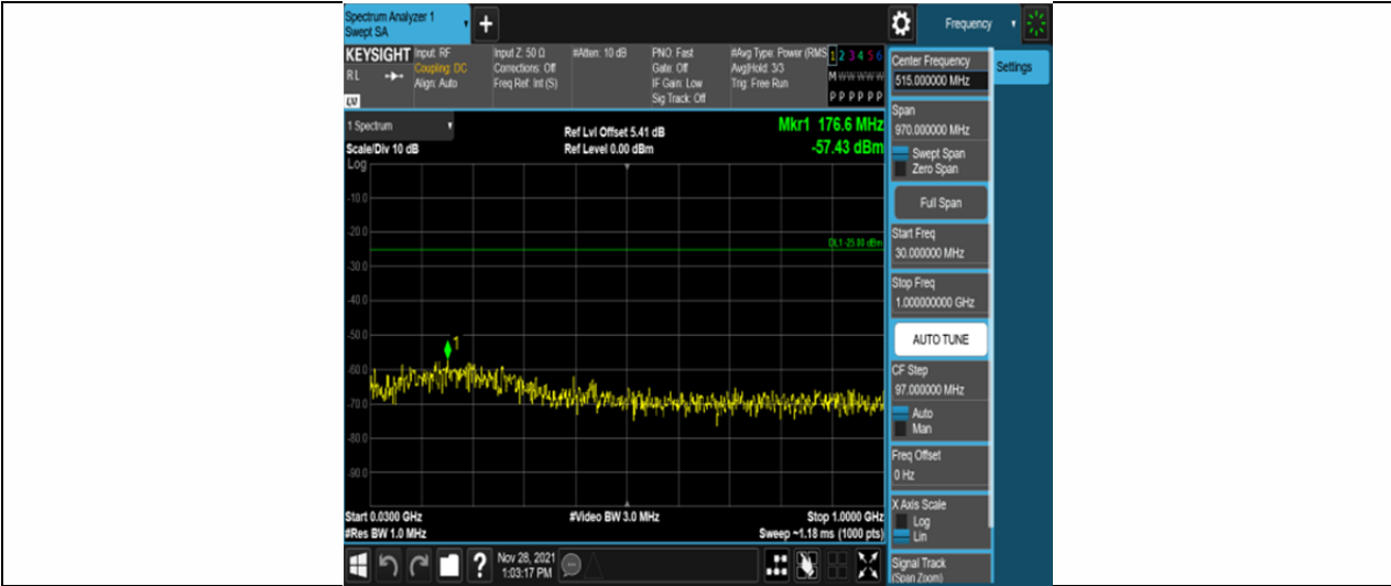
Band41-15MHz-16QAM-39725-75RB#0-Range1:30~1000MHz
