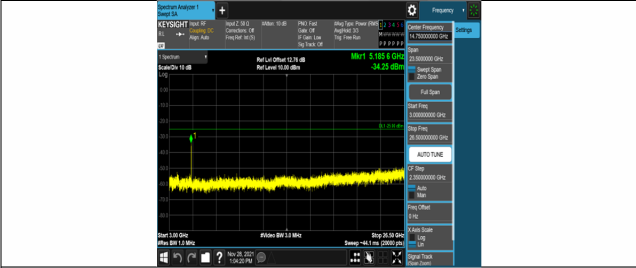
Band41-15MHz-QPSK-40620-75RB#0-Range3:3000~26500MHz
