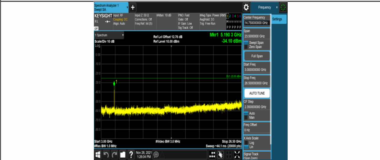
Band41-20MHz-16QAM-40620-100RB#0-Range3:3000~26500MHz
