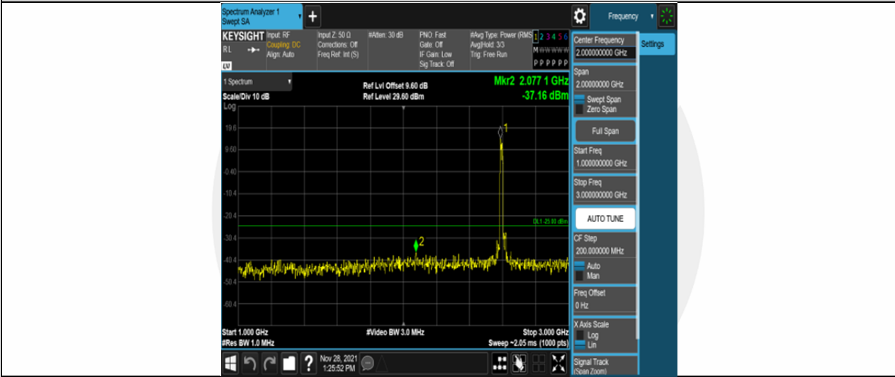
Band41-20MHz-16QAM-40620-100RB#0-Range2:1000~3000MHz
