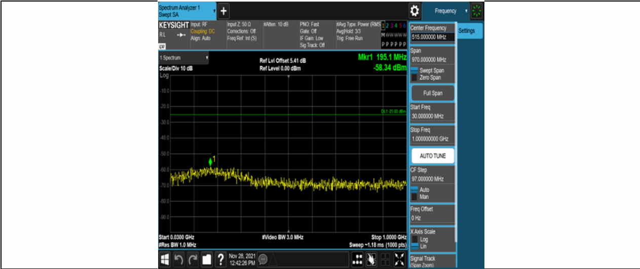
Band41-10MHz-16QAM-39700-50RB#0-Range1:30~1000MHz
