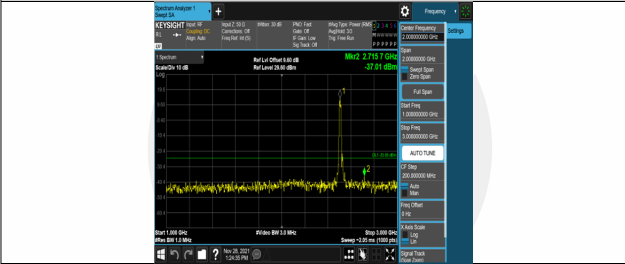
Band41-20MHz-16QAM-39750-100RB#0-Range2:1000~3000MHz
