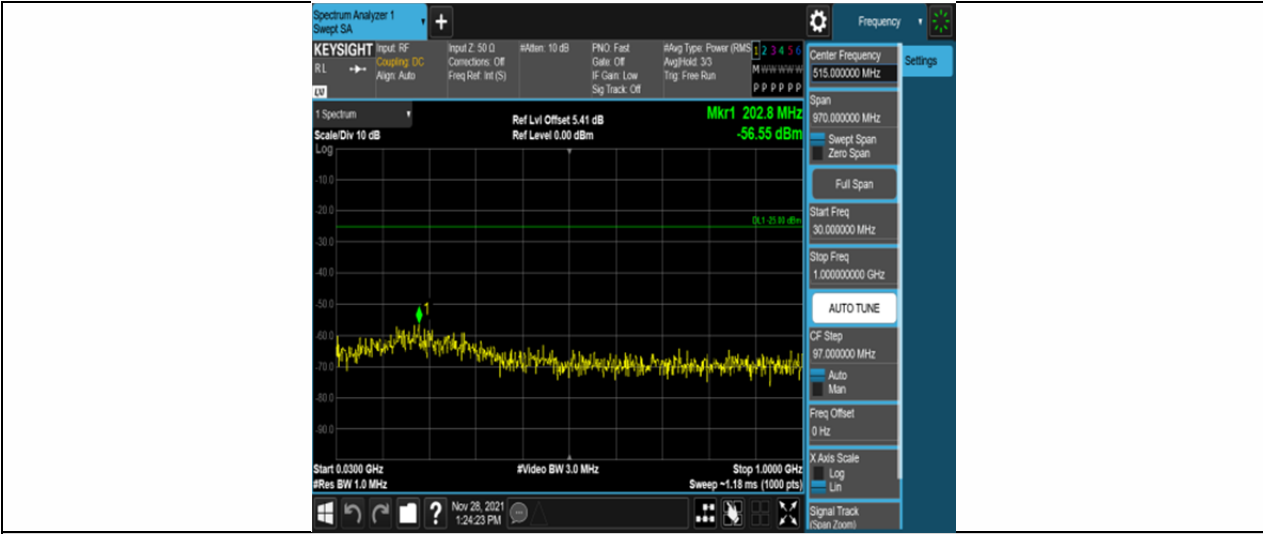
Band41-20MHz-16QAM-39750-100RB#0-Range1:30~1000MHz
