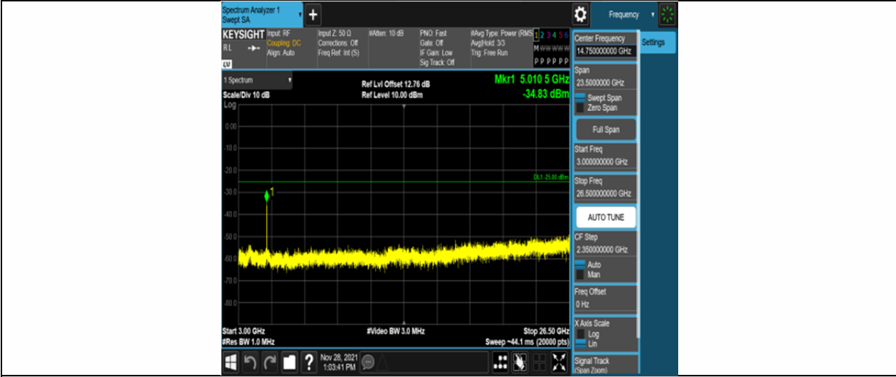
Band41-15MHz-16QAM-39725-75RB#0-Range3:3000~26500MHz
