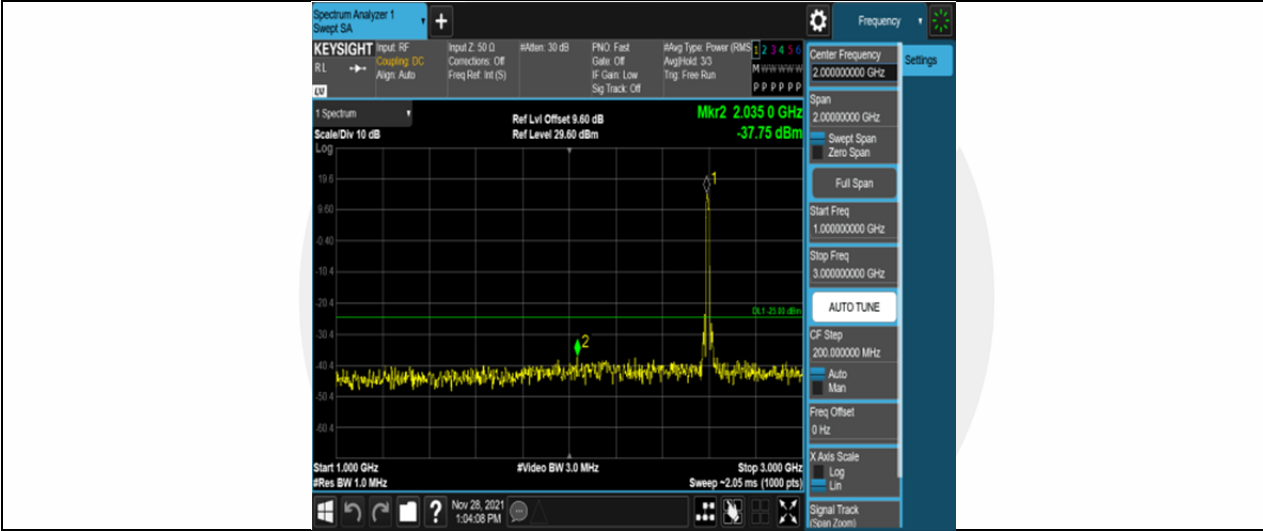
Band41-15MHz-QPSK-40620-75RB#0-Range2:1000~3000MHz
