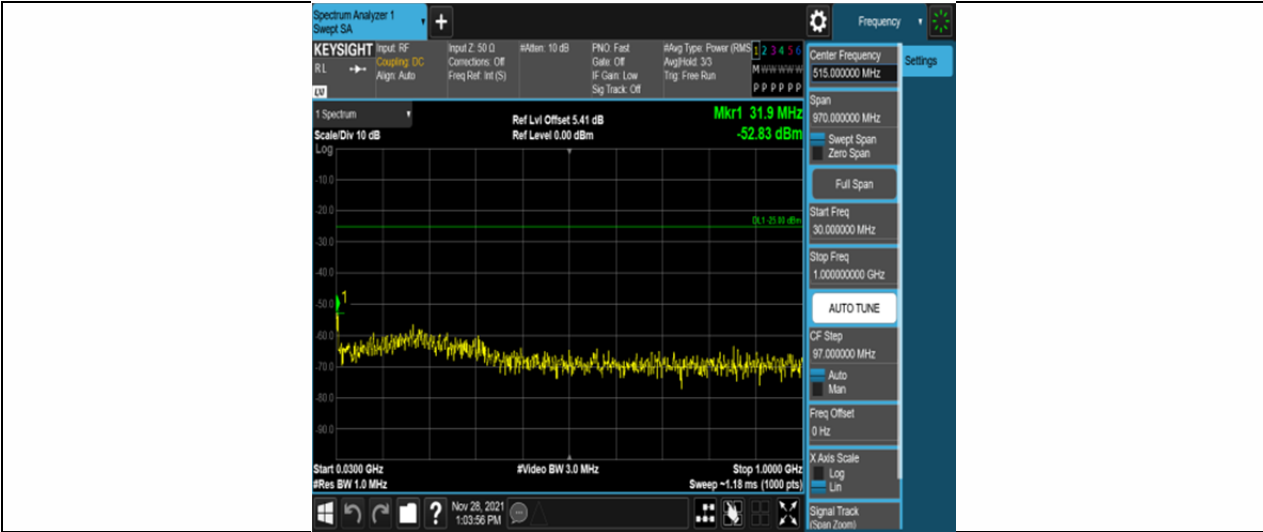
Band41-15MHz-QPSK-40620-75RB#0-Range1:30~1000MHz
