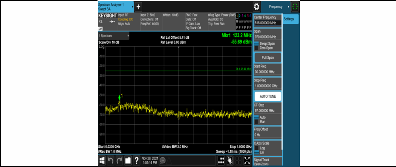
Band41-15MHz-QPSK-41515-75RB#0-Range1:30~1000MHz
