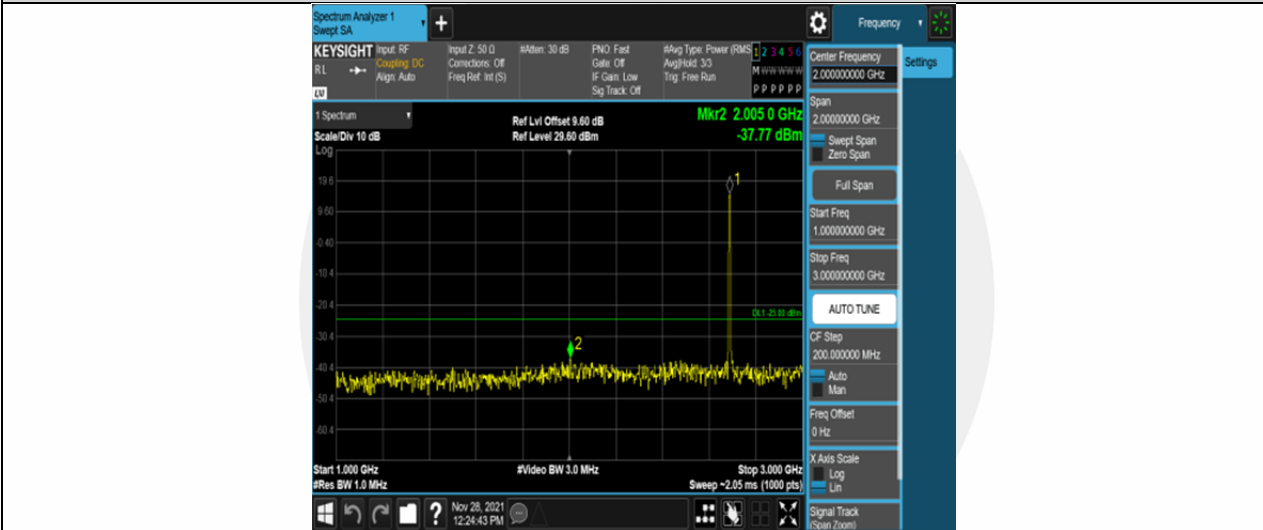
Band41-5MHz-16QAM-41565-25RB#0-Range2:1000~3000MHz
