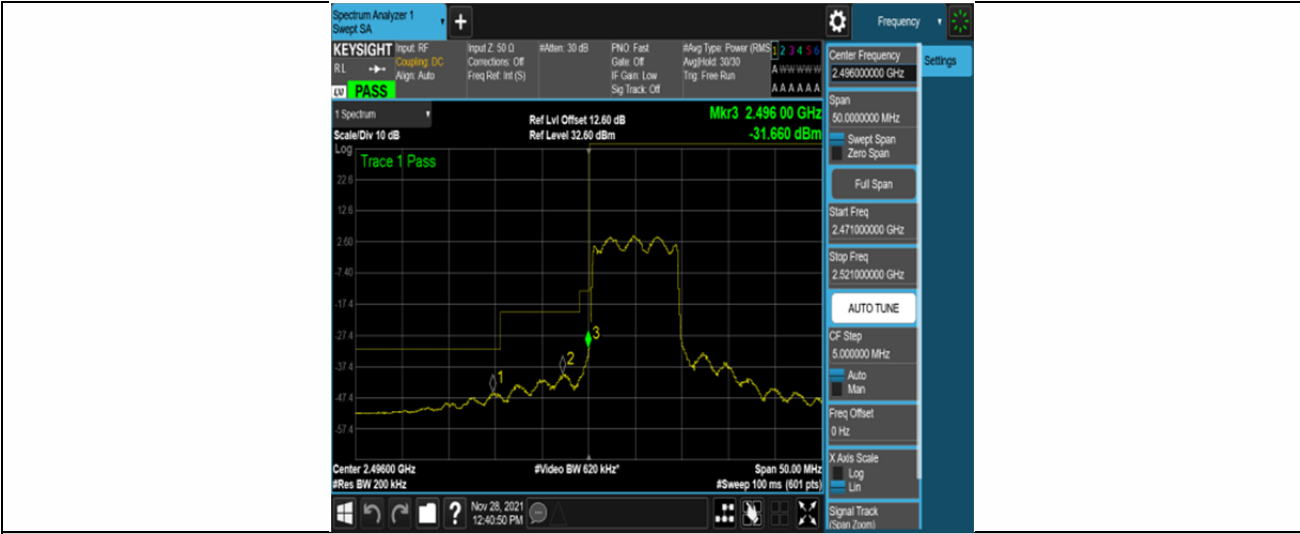
Band41-10MHz-16QAM-39700-50RB#0
