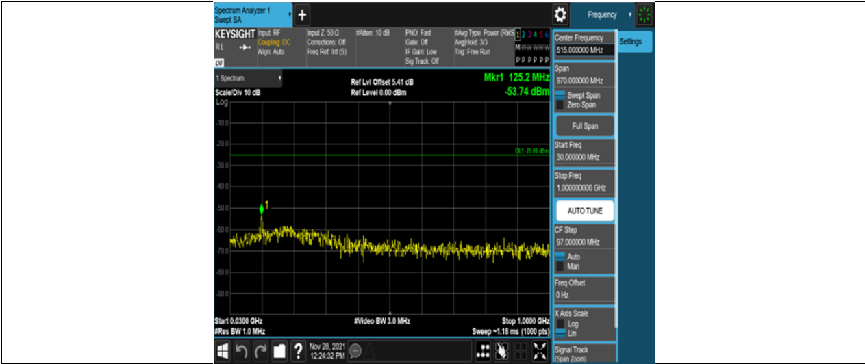
Band41-5MHz-16QAM-41565-25RB#0-Range1:30~1000MHz
