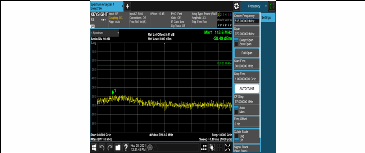
Band41-5MHz-16QAM-39675-25RB#0-Range1:30~1000MHz
