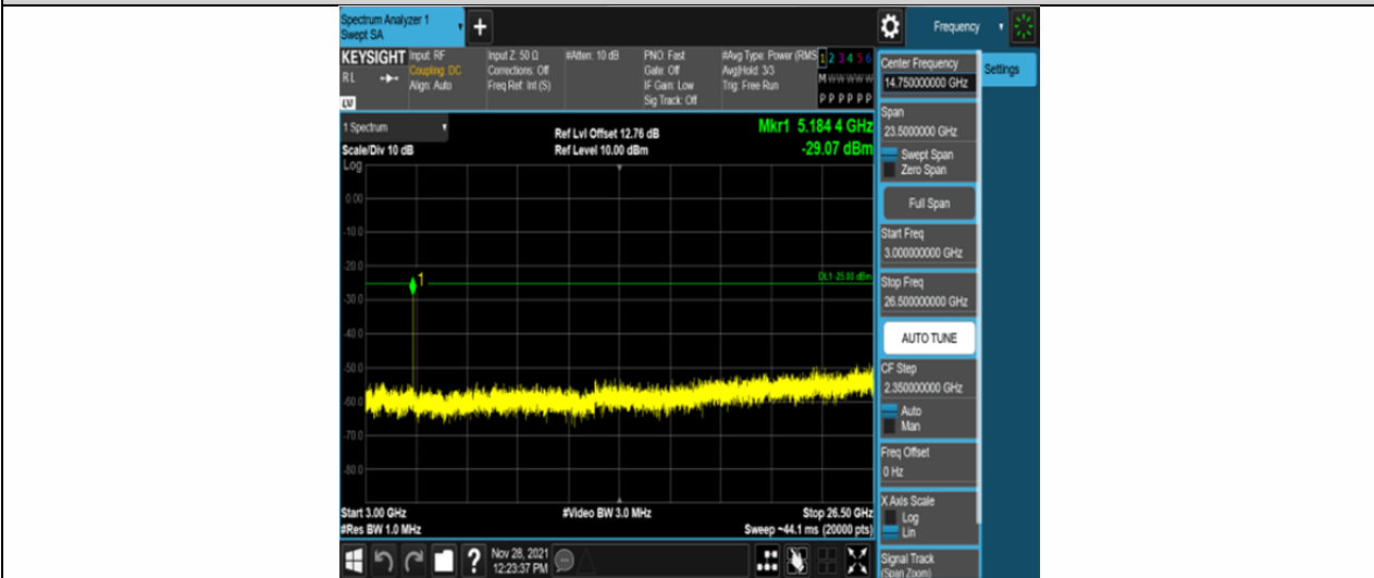
Band41-5MHz-16QAM-40620-25RB#0-Range3:3000~26500MHz
