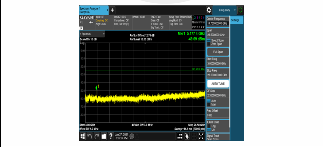
Band41-5MHz-16QAM-39675-25RB#0-Range3:3000~26500MHz
