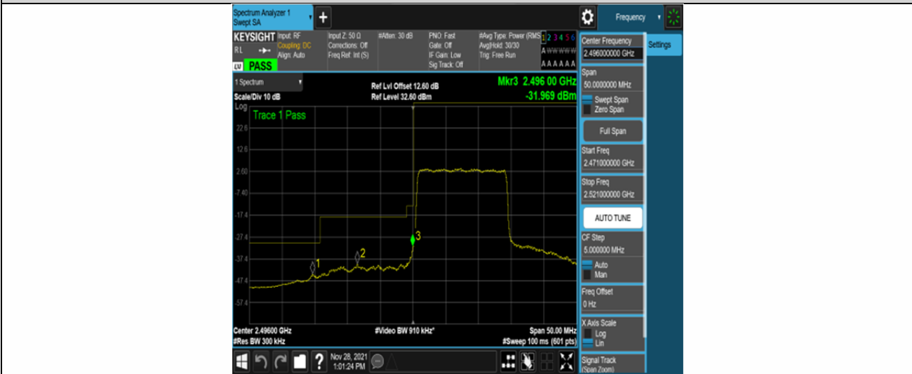
Band41-15MHz-QPSK-39725-75RB#0
