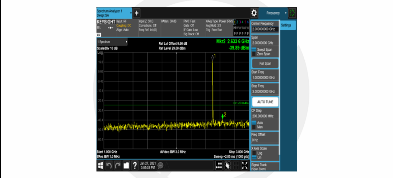
Band41-5MHz-16QAM-39675-25RB#0-Range2:1000~3000MHz
