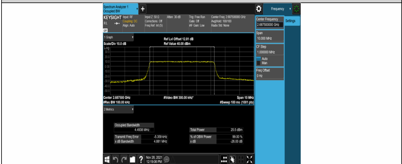
Band41-5MHz-QPSK-41565-25RB#0
