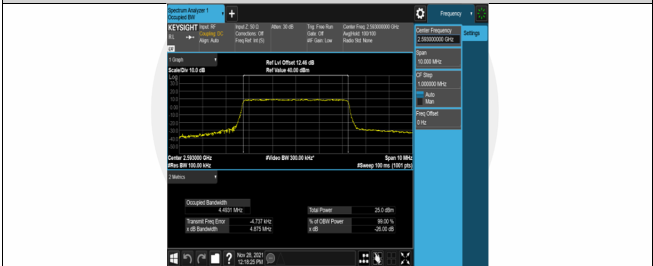
Band41-5MHz-QPSK-40620-25RB#0
