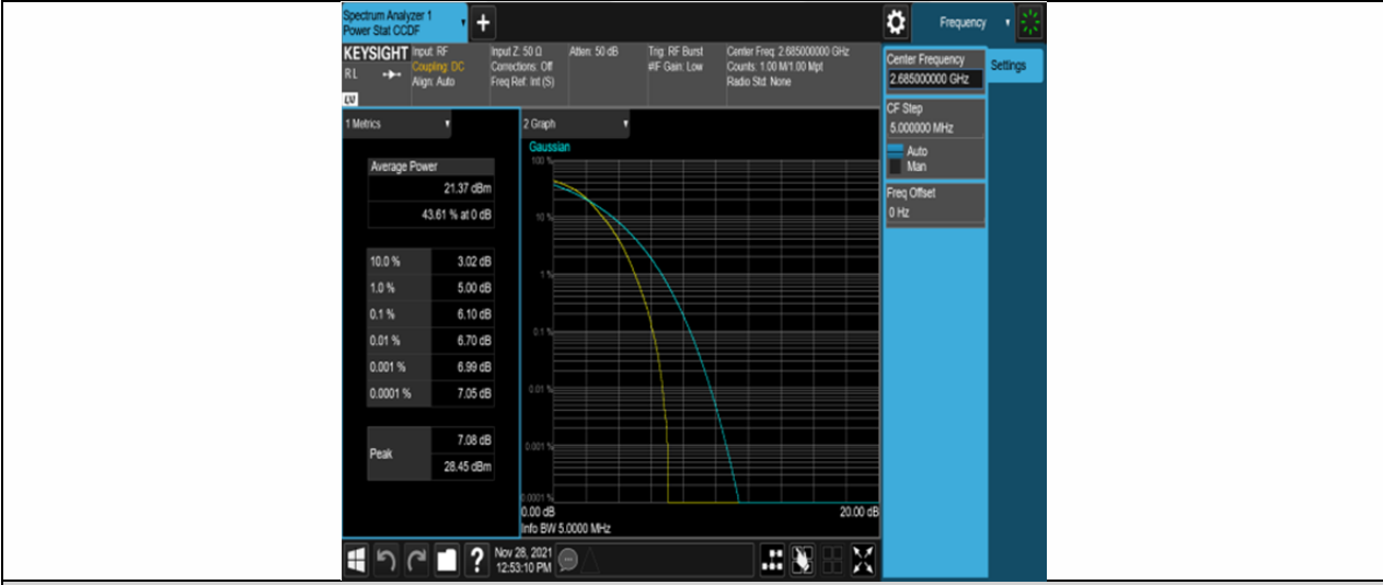
Band41-10MHz-16QAM-41540-50RB#0
