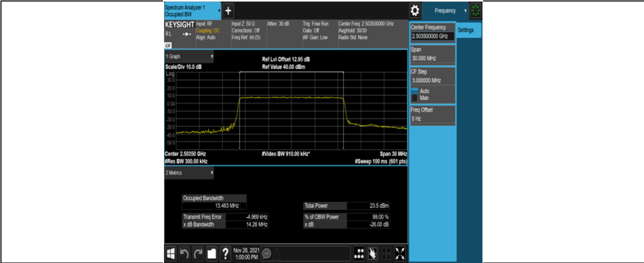
Band41-15MHz-16QAM-39725-75RB#0
