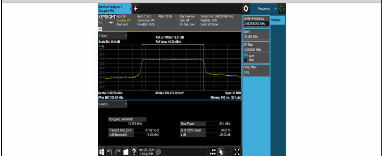
Band41-15MHz-QPSK-41515-75RB#0
