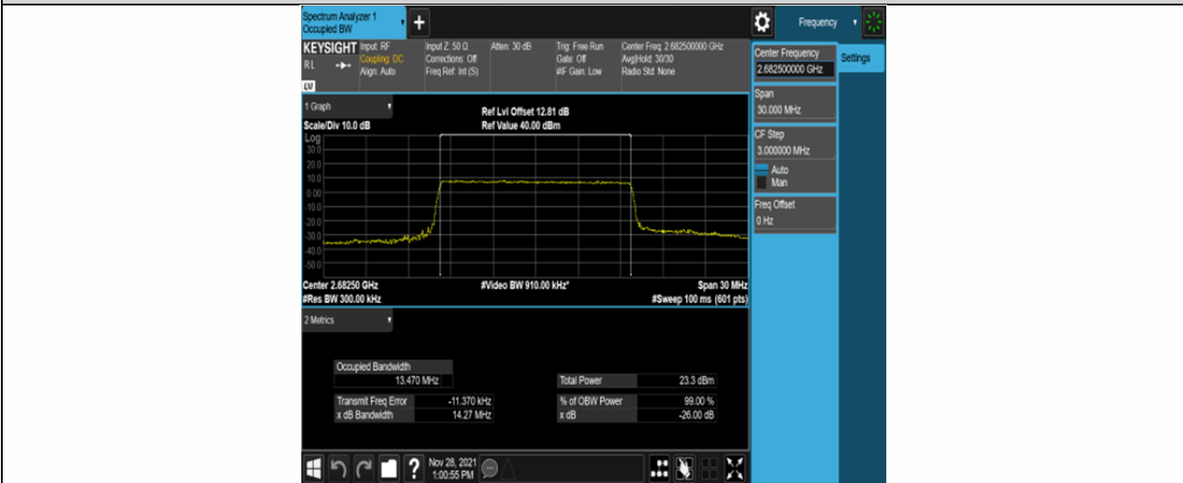
Band41-15MHz-16QAM-41515-75RB#0
