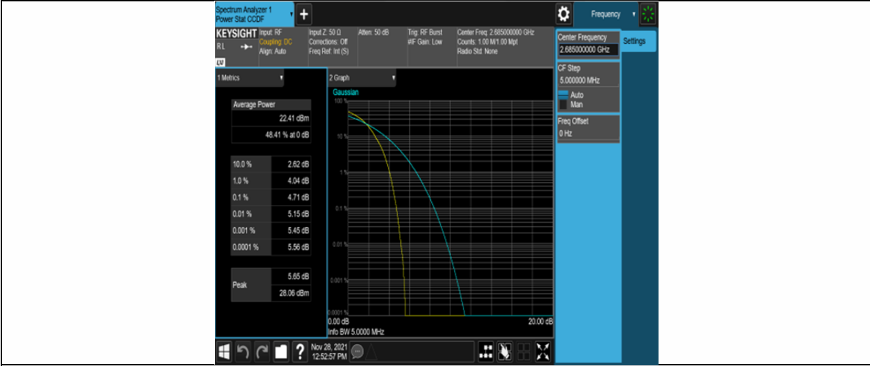
Band41-10MHz-QPSK-41540-50RB#0
