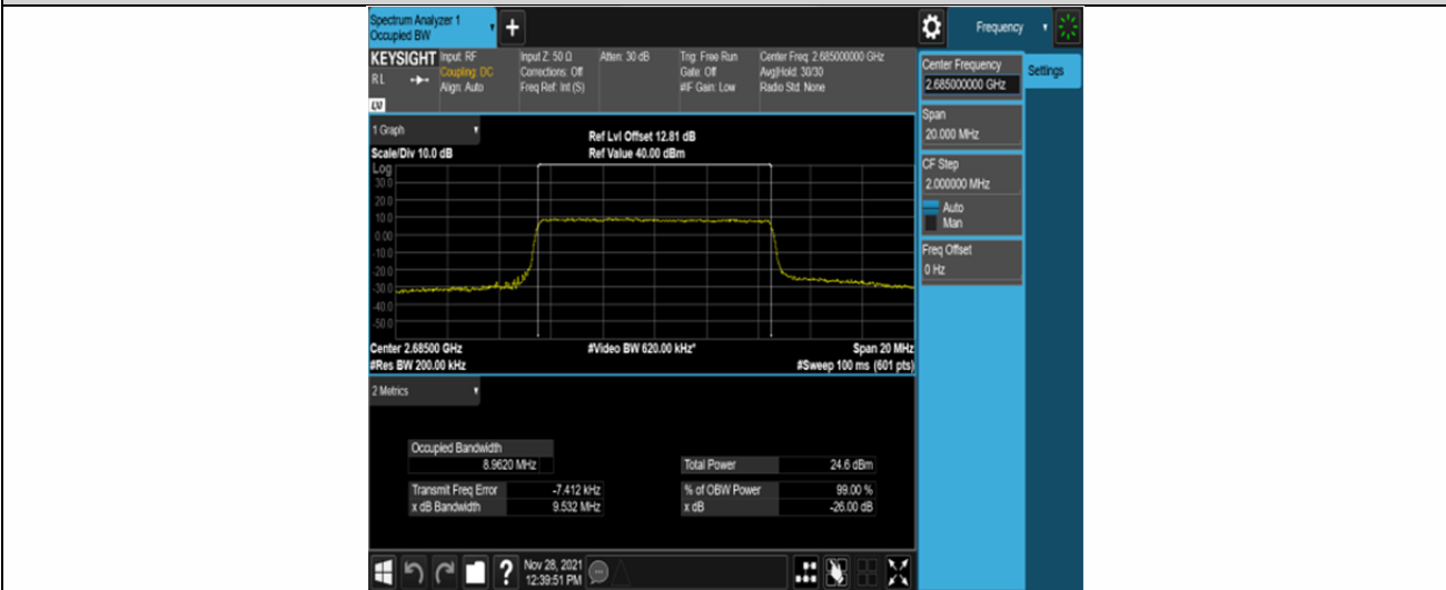
Band41-10MHz-QPSK-41540-50RB#0
