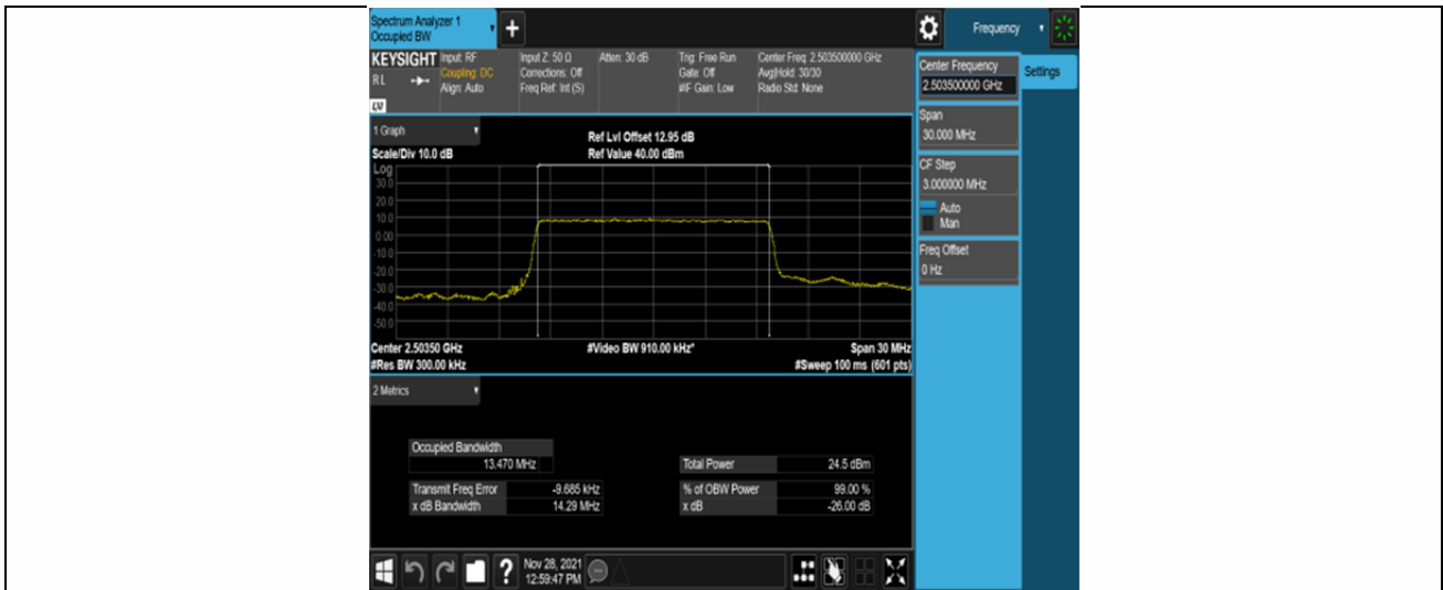
Band41-15MHz-QPSK-39725-75RB#0
