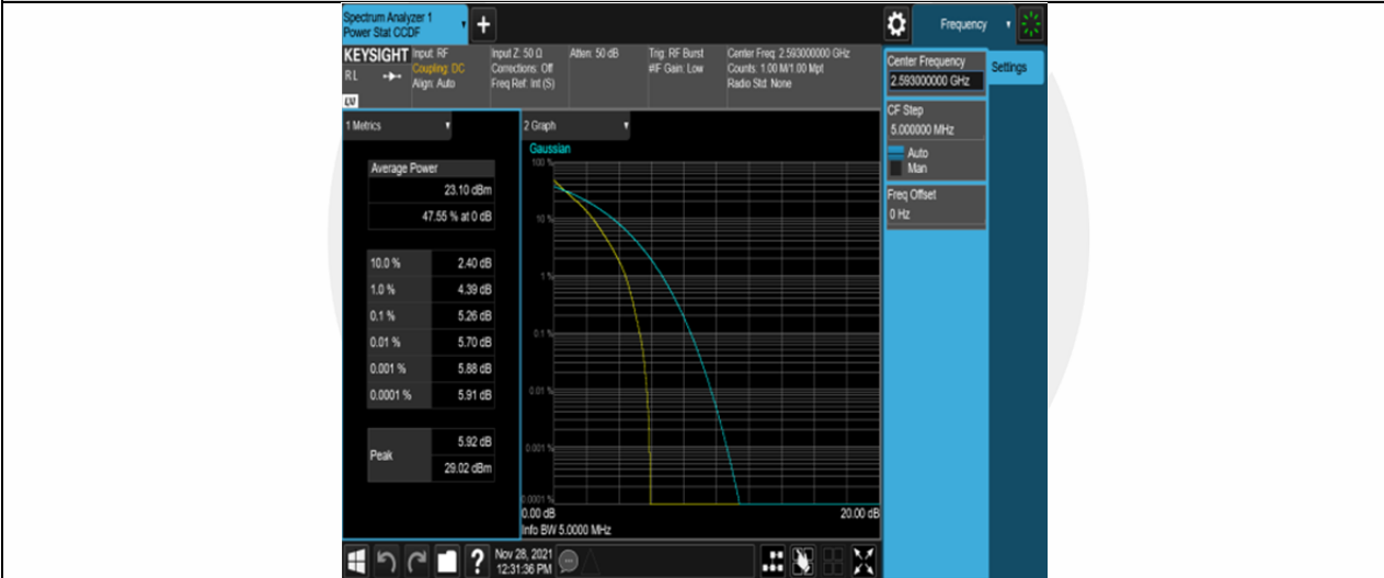
Band41-5MHz-QPSK-40620-25RB#0
