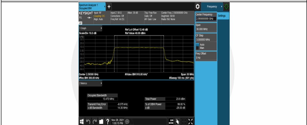
Band41-15MHz-QPSK-40620-75RB#0
