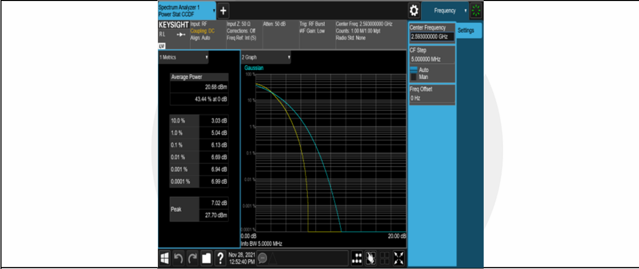
Band41-10MHz-16QAM-40620-50RB#0
