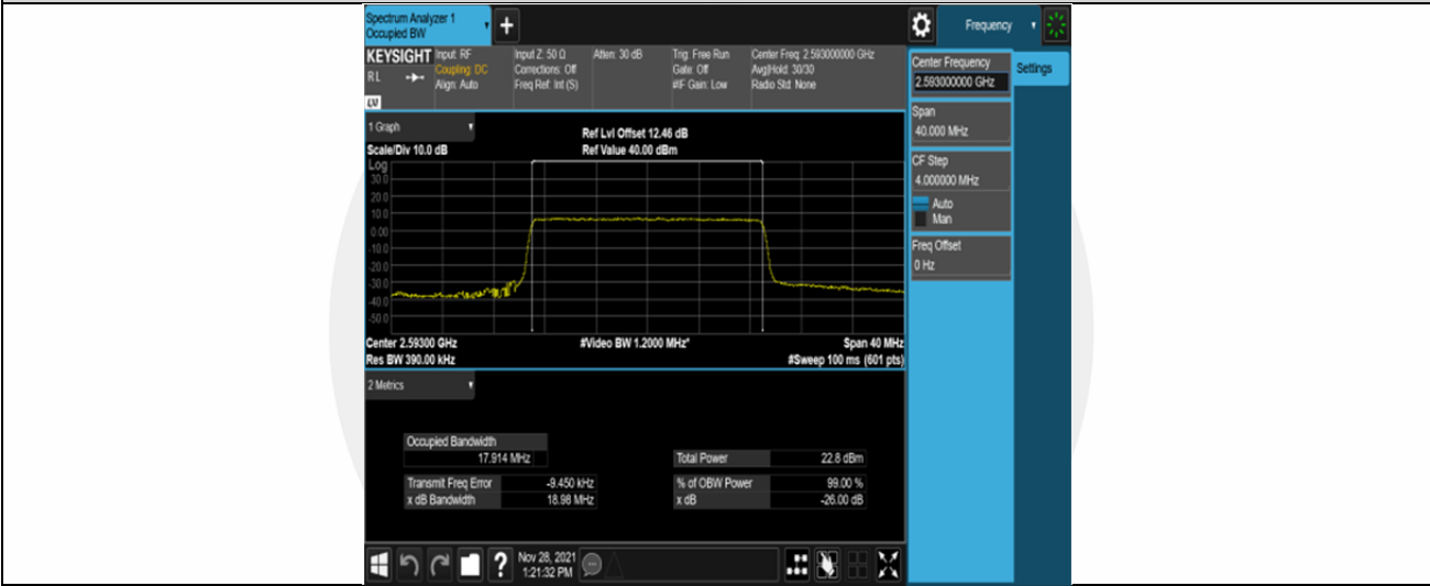
Band41-20MHz-16QAM-40620-100RB#0
