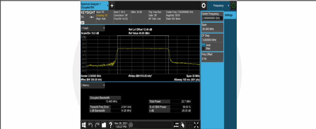
Band41-15MHz-16QAM-40620-75RB#0
