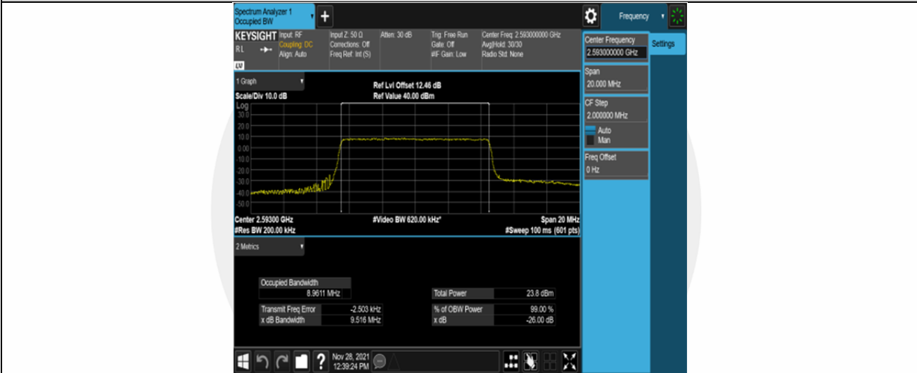
Band41-10MHz-QPSK-40620-50RB#0
