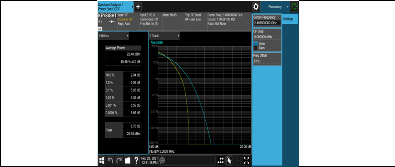
Band41-5MHz-16QAM-39675-25RB#0
