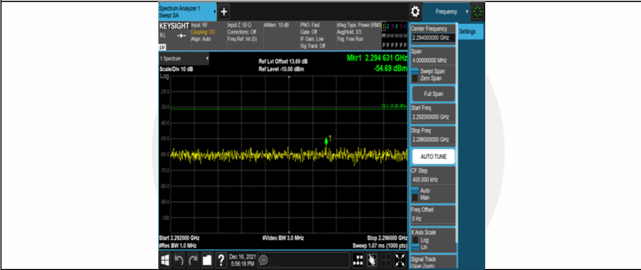
Band30-10MHz-16QAM-27710-50RB#0-Range4:2292~2296MHz
