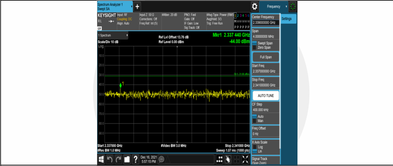
Band30-10MHz-16QAM-27710-50RB#0-Range10:2337~2341MHz
