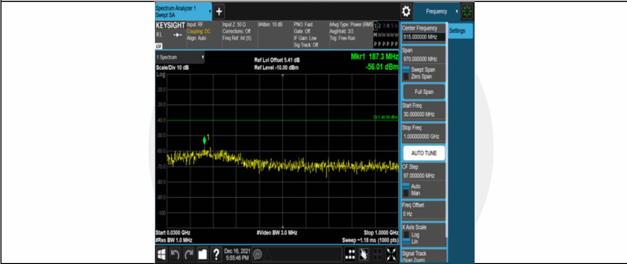
Band30-10MHz-16QAM-27710-50RB#0-Range1:30~1000MHz
