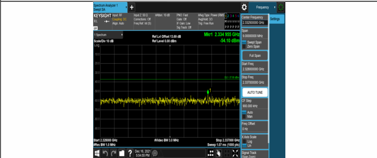
Band30-10MHz-QPSK-27710-50RB#0-Range9:2328~2337MHz
