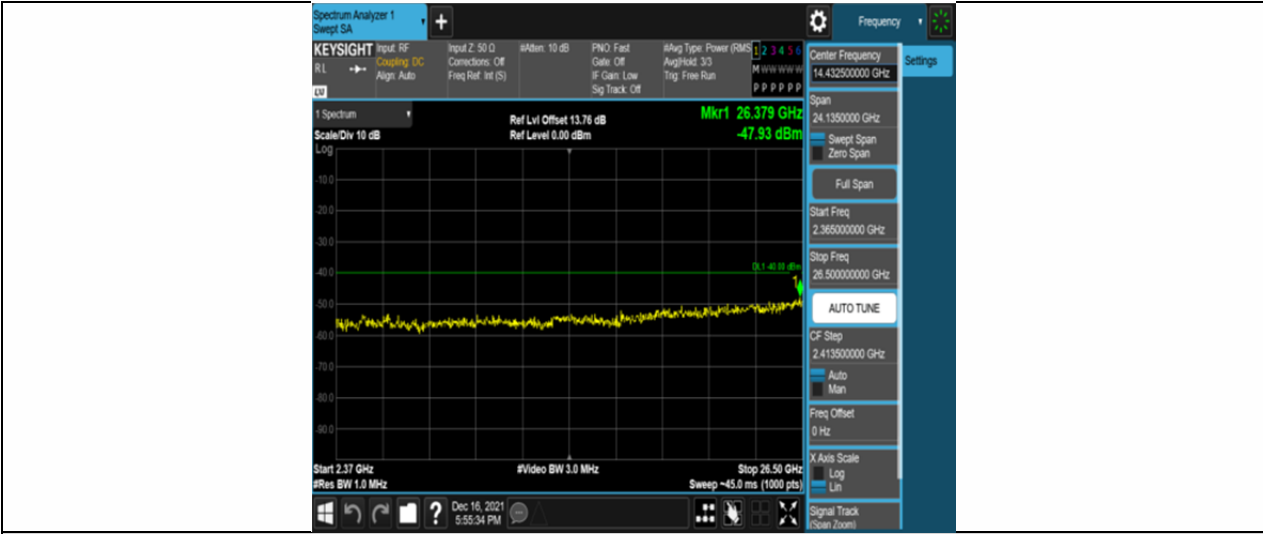
Band30-10MHz-QPSK-27710-50RB#0-Range13:2365~26500MHz
