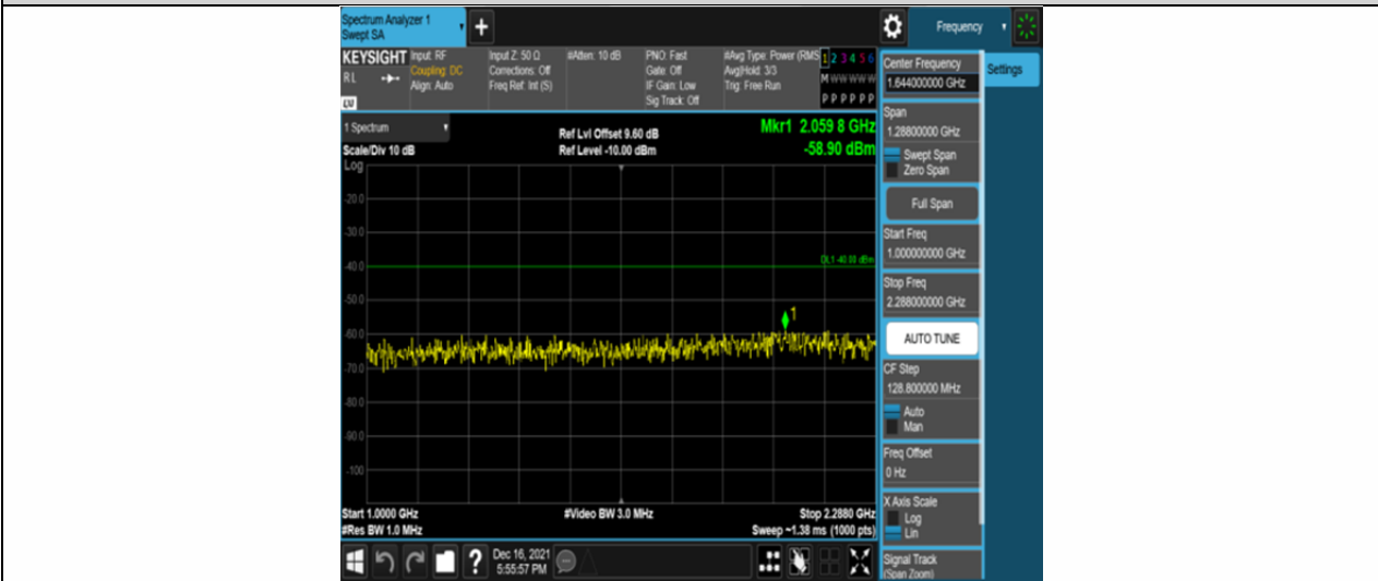
Band30-10MHz-16QAM-27710-50RB#0-Range2:1000~2288MHz
