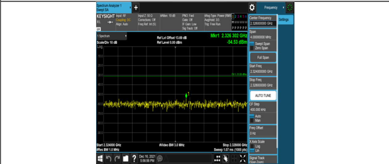
Band30-10MHz-16QAM-27710-50RB#0-Range8:2324~2328MHz
