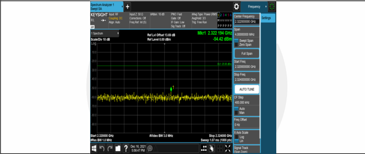
Band30-10MHz-16QAM-27710-50RB#0-Range7:2320~2324MHz
