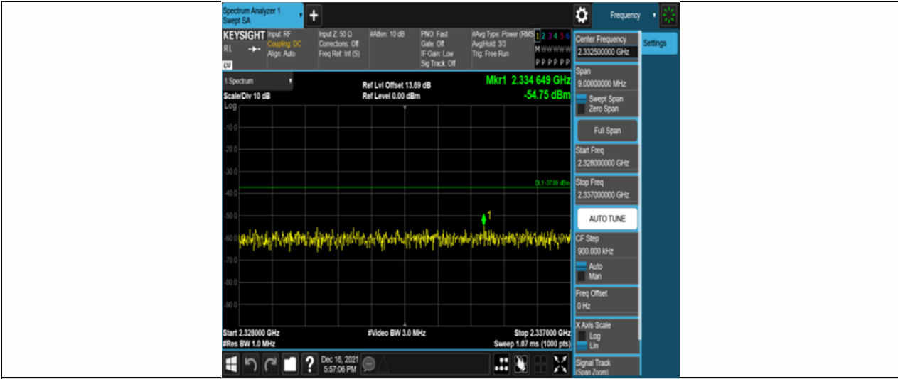
Band30-10MHz-16QAM-27710-50RB#0-Range9:2328~2337MHz
