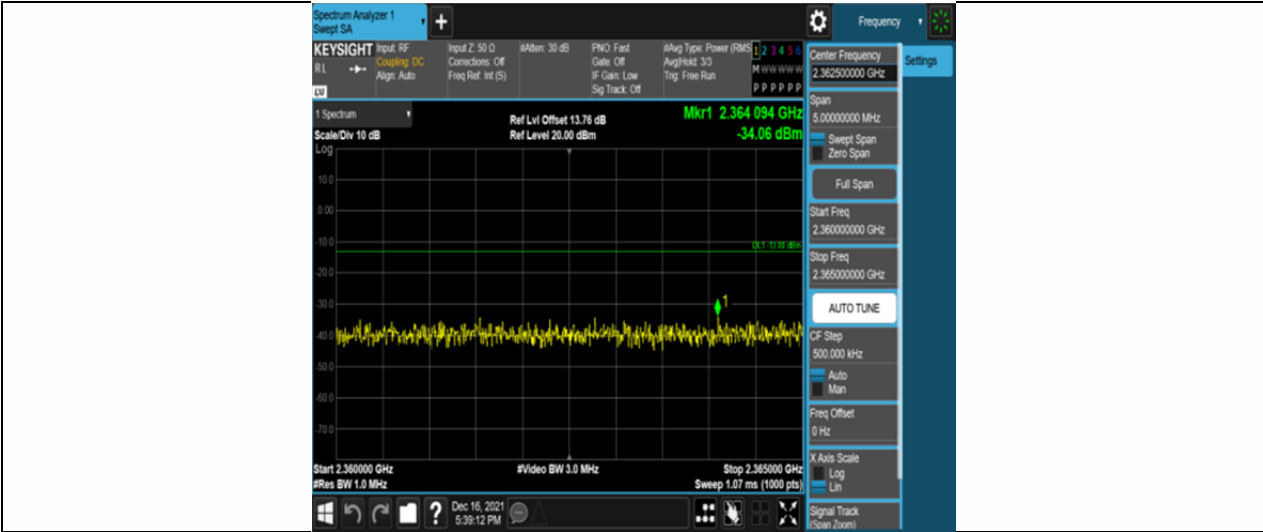
Band30-5MHz-16QAM-27710-25RB#0-Range12:2360~2365MHz
