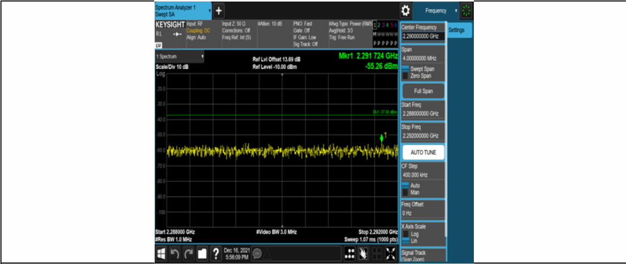
Band30-10MHz-16QAM-27710-50RB#0-Range3:2288~2292MHz
