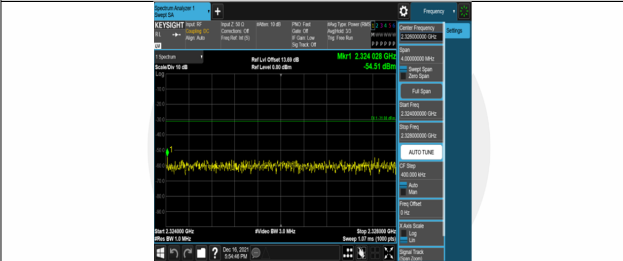
Band30-10MHz-QPSK-27710-50RB#0-Range8:2324~2328MHz
