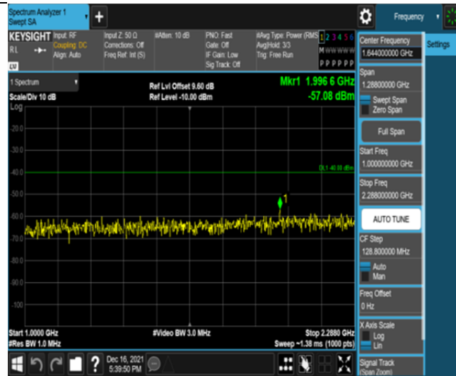
Band30-5MHz-QPSK-27735-25RB#0-Range2:1000~2288MHz
