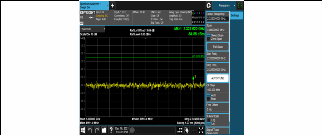
Band30-5MHz-16QAM-27685-25RB#0-Range7:2320~2324MHz
