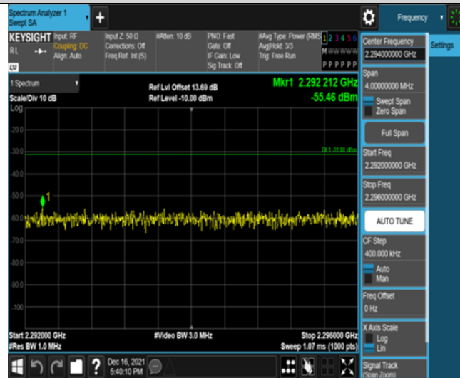
Band30-5MHz-QPSK-27735-25RB#0-Range4:2292~2296MHz
