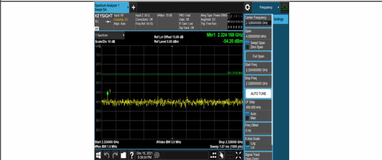
Band30-5MHz-16QAM-27710-25RB#0-Range8:2324~2328MHz
