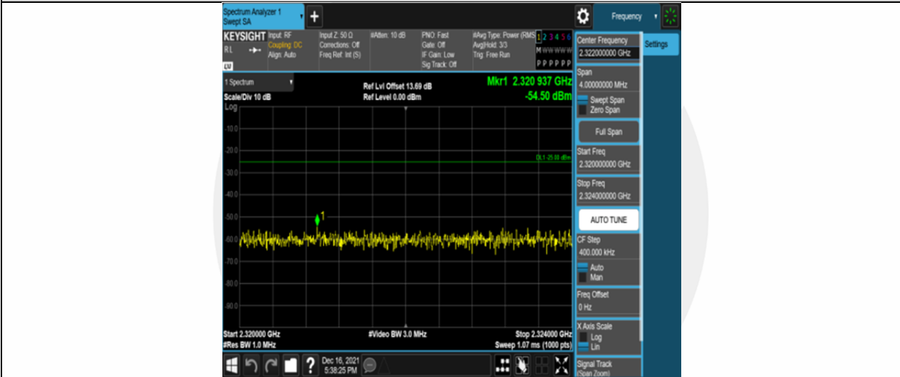
Band30-5MHz-16QAM-27710-25RB#0-Range7:2320~2324MHz
