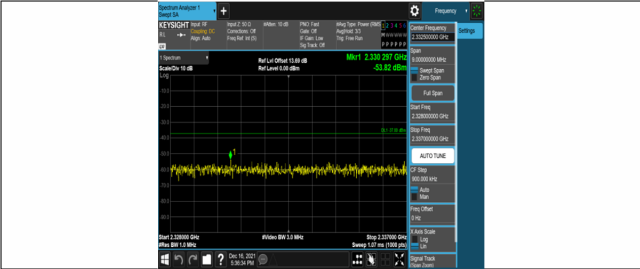
Band30-5MHz-QPSK-27710-25RB#0-Range9:2328~2337MHz
