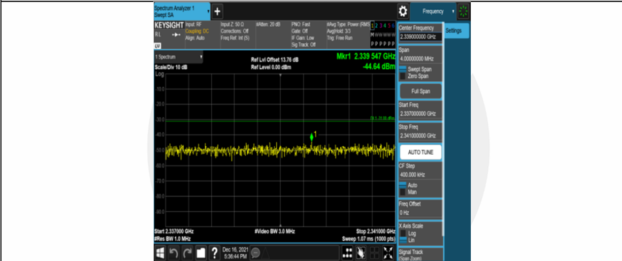
Band30-5MHz-QPSK-27710-25RB#0-Range10:2337~2341MHz
