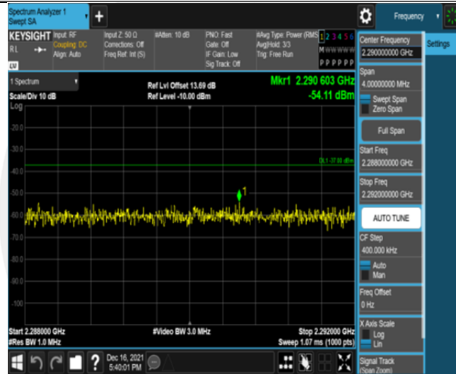
Band30-5MHz-QPSK-27735-25RB#0-Range3:2288~2292MHz
