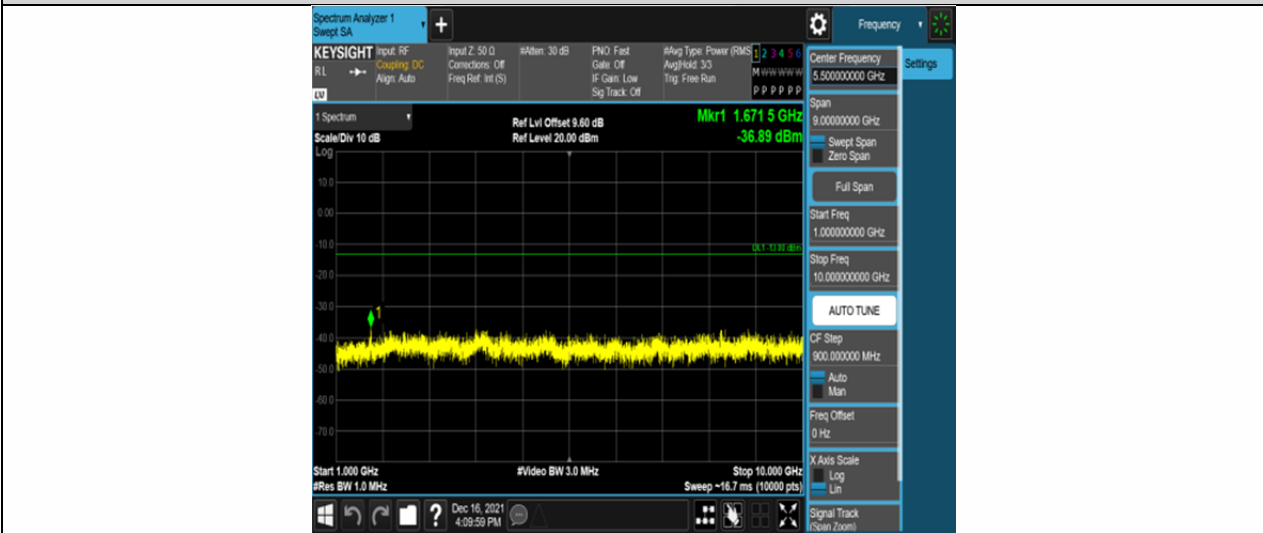
Band26-15MHz-16QAM-26915-75RB#0-Range2:1000~10000MHz
