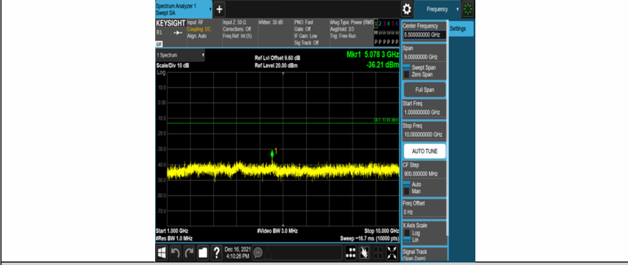
Band26-15MHz-QPSK-26965-75RB#0-Range2:1000~10000MHz
