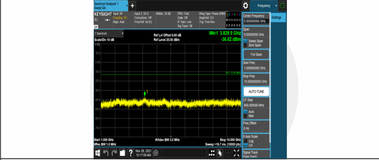
Band26-15MHz-16QAM-26765-75RB#0-Range2:1000~10000MHz
