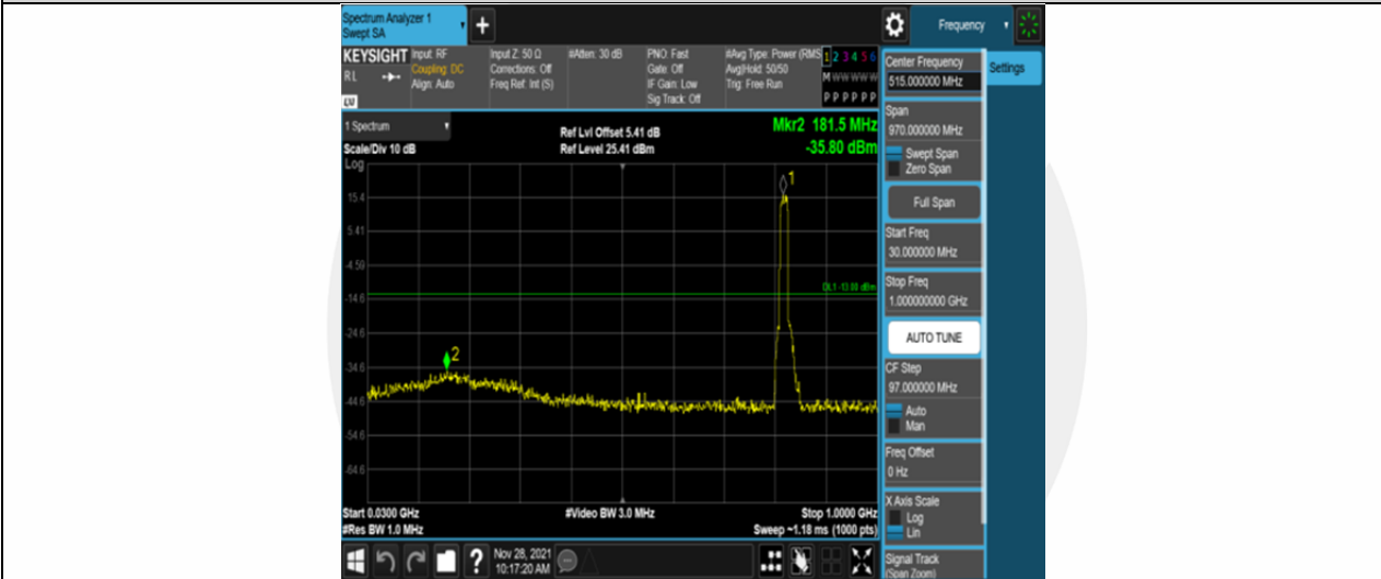
Band26-15MHz-QPSK-26765-75RB#0-Range1:30~1000MHz
