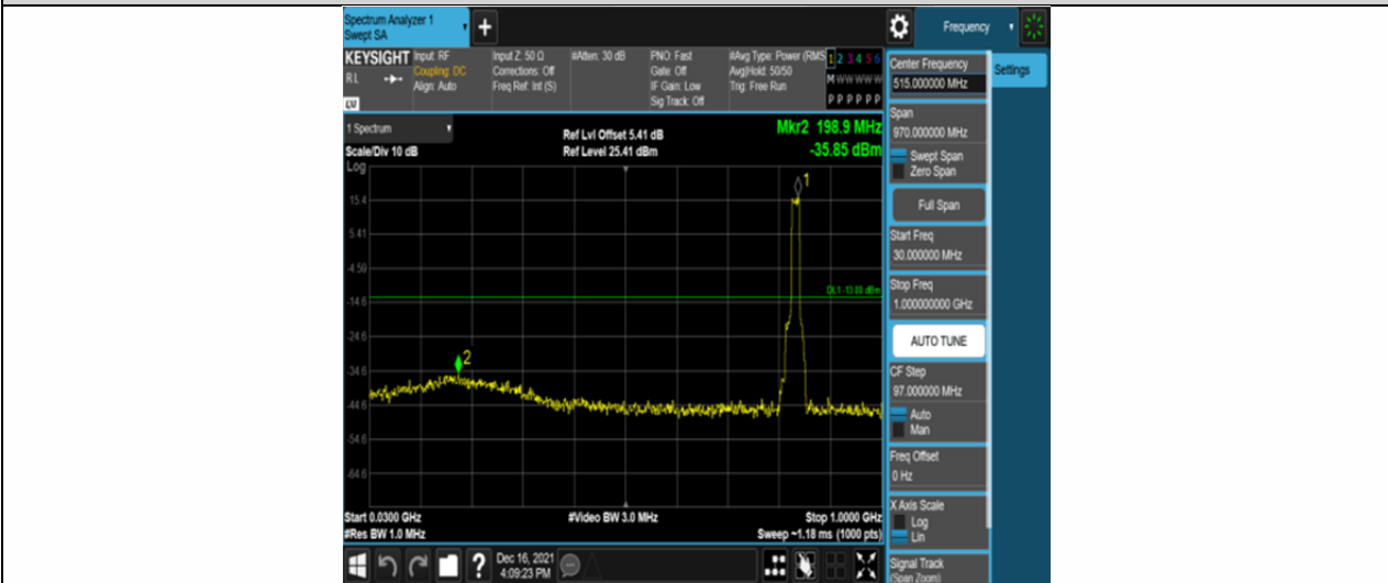
Band26-15MHz-QPSK-26915-75RB#0-Range1:30~1000MHz
