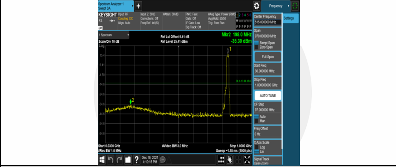
Band26-15MHz-QPSK-26965-75RB#0-Range1:30~1000MHz
