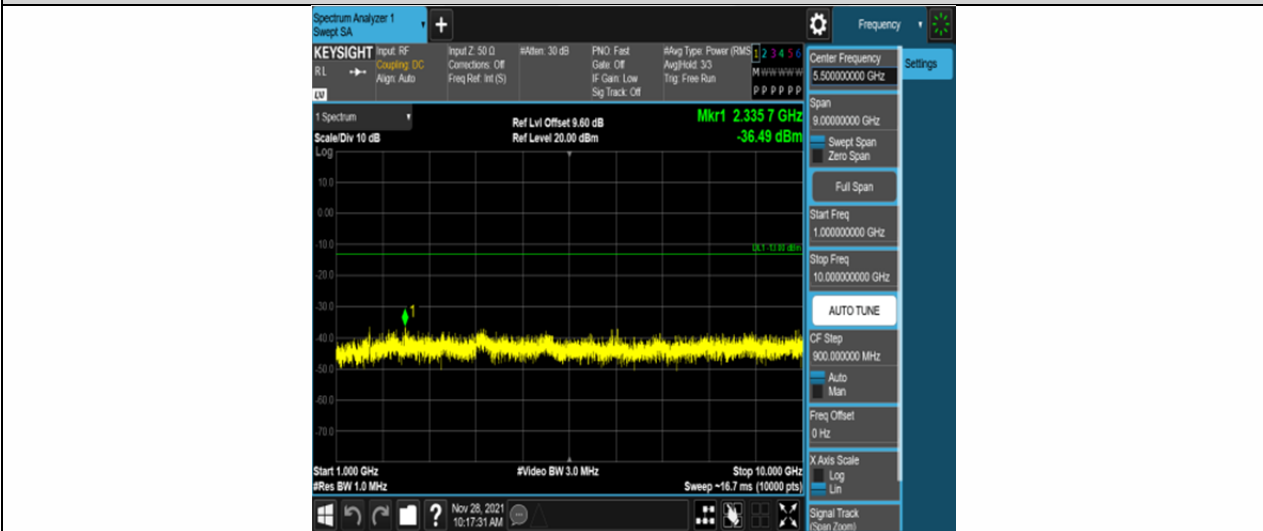
Band26-15MHz-QPSK-26765-75RB#0-Range2:1000~10000MHz
