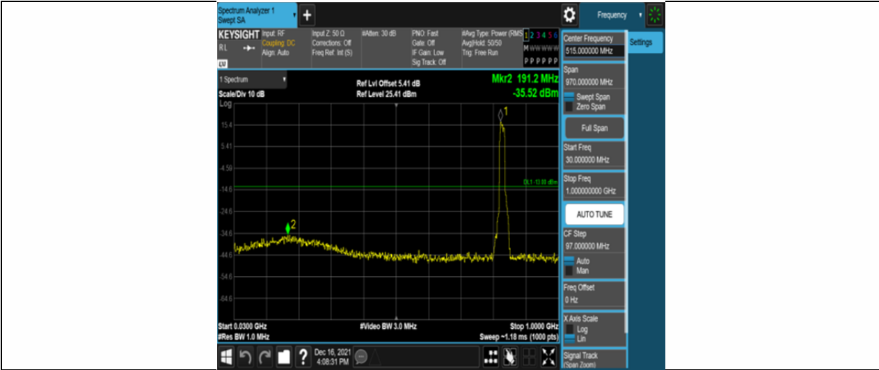
Band26-15MHz-QPSK-26865-75RB#0-Range1:30~1000MHz
