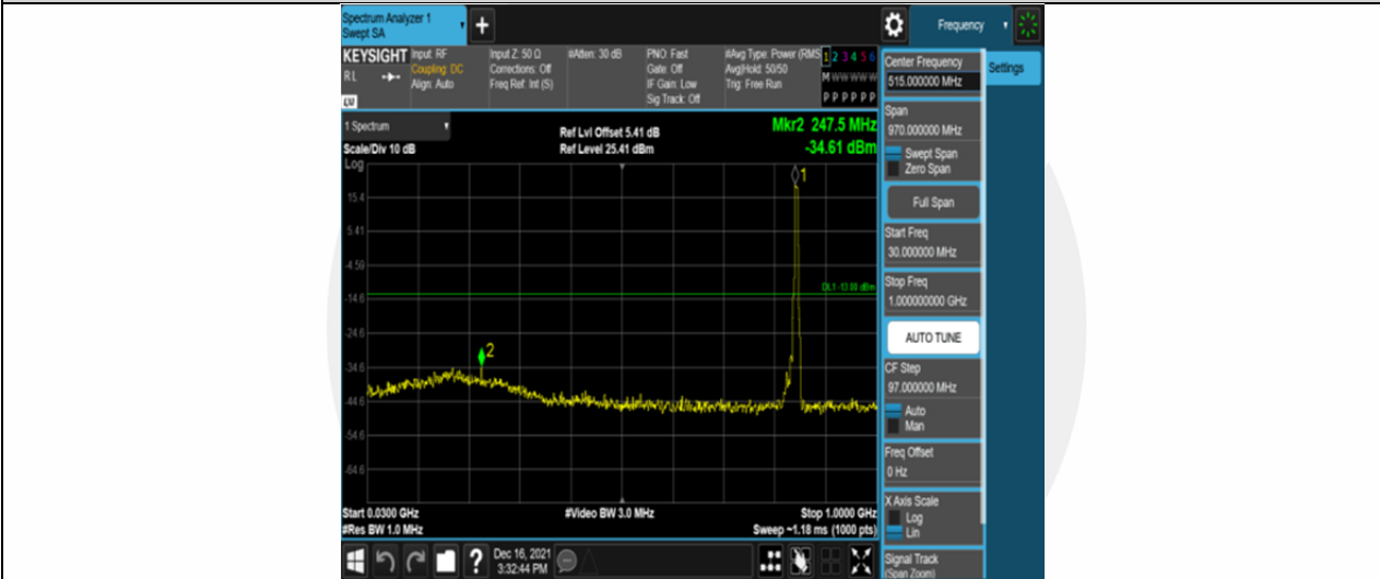
Band26-5MHz-QPSK-27015-25RB#0-Range1:30~1000MHz
