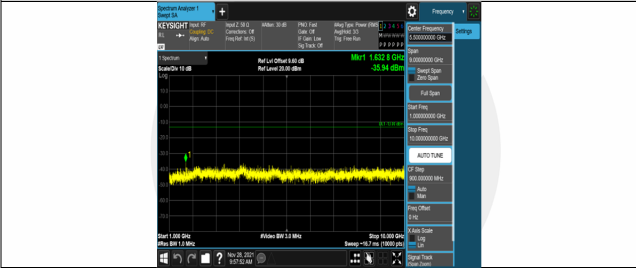
Band26-5MHz-16QAM-26715-25RB#0-Range2:1000~10000MHz
