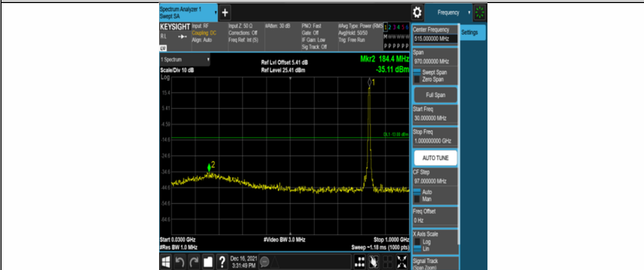
Band26-5MHz-QPSK-26915-25RB#0-Range1:30~1000MHz
