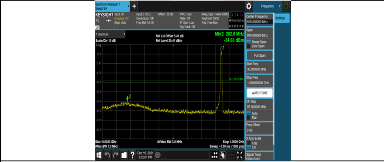
Band26-10MHz-16QAM-26990-50RB#0-Range1:30~1000MHz
