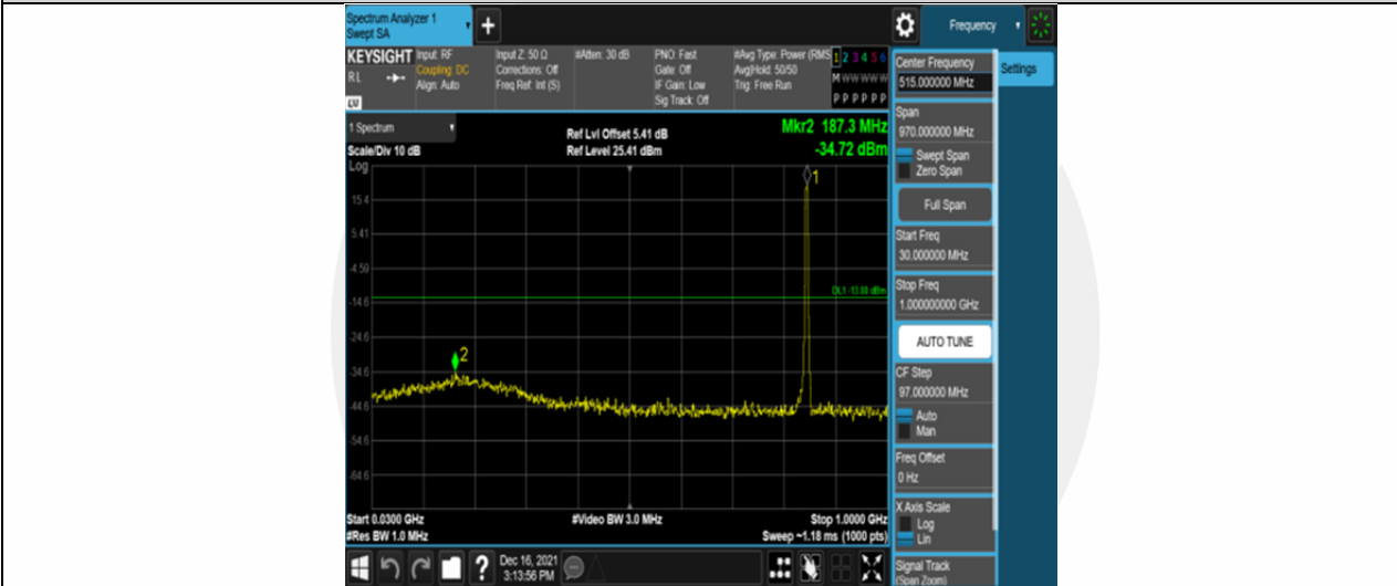
Band26-3MHz-16QAM-27025-15RB#0-Range1:30~1000MHz
