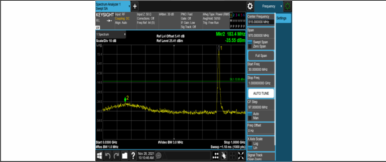
Band26-10MHz-16QAM-26740-50RB#0-Range1:30~1000MHz
