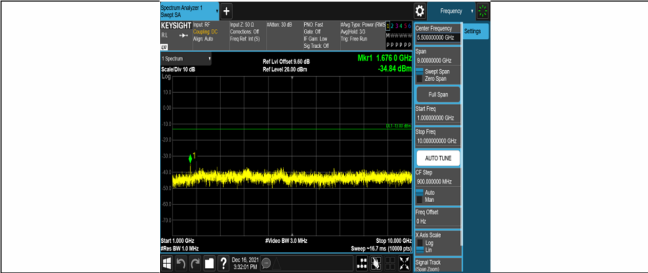
Band26-5MHz-QPSK-26915-25RB#0-Range2:1000~10000MHz
