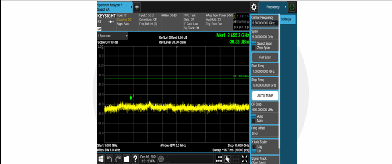
Band26-5MHz-16QAM-26815-25RB#0-Range2:1000~10000MHz
