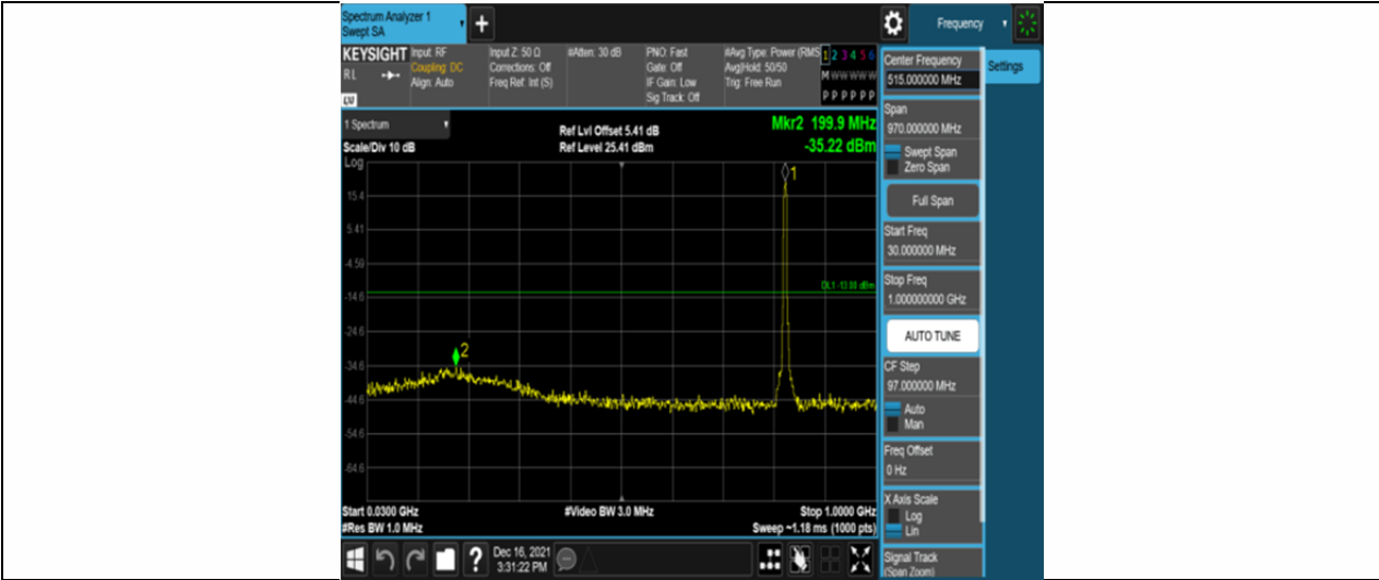
Band26-5MHz-16QAM-26815-25RB#0-Range1:30~1000MHz
