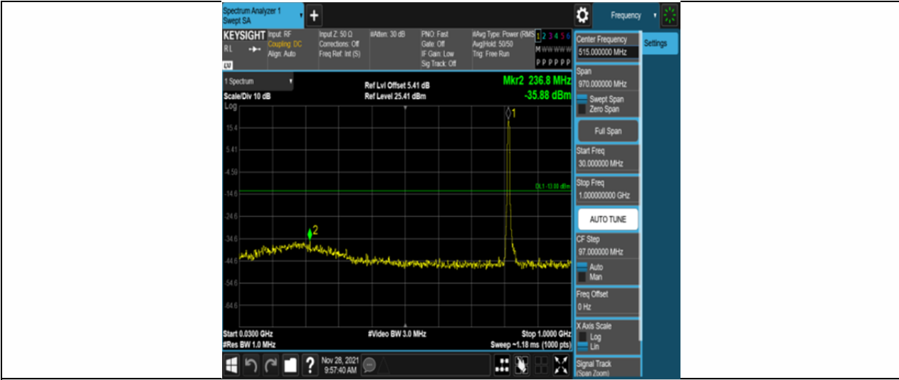
Band26-5MHz-16QAM-26715-25RB#0-Range1:30~1000MHz
