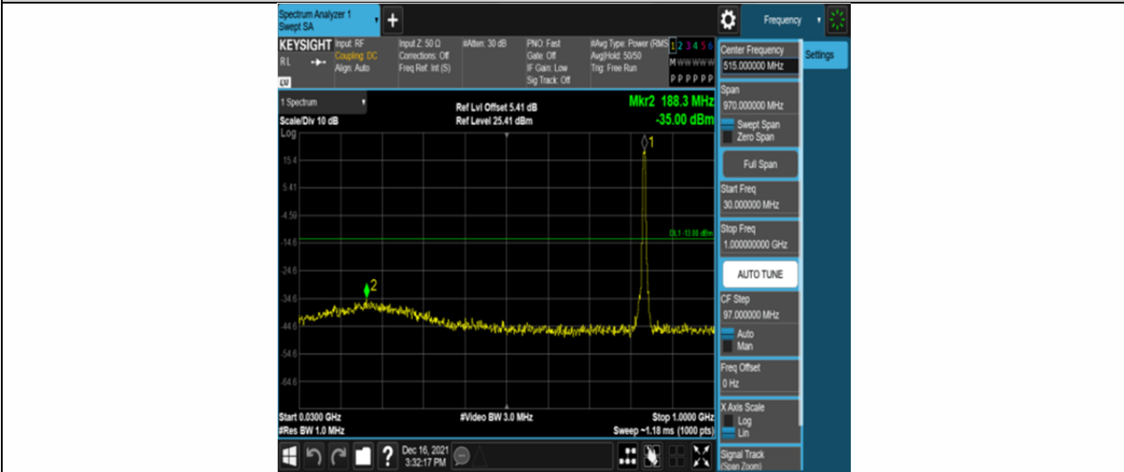
Band26-5MHz-16QAM-26915-25RB#0-Range1:30~1000MHz
