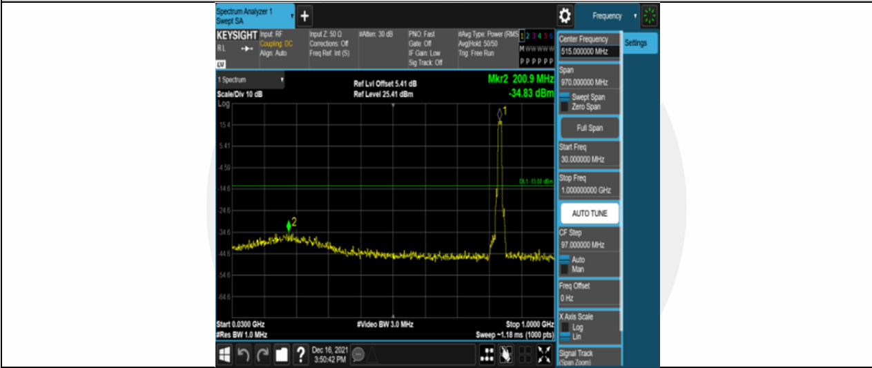
Band26-10MHz-QPSK-26915-50RB#0-Range1:30~1000MHz
