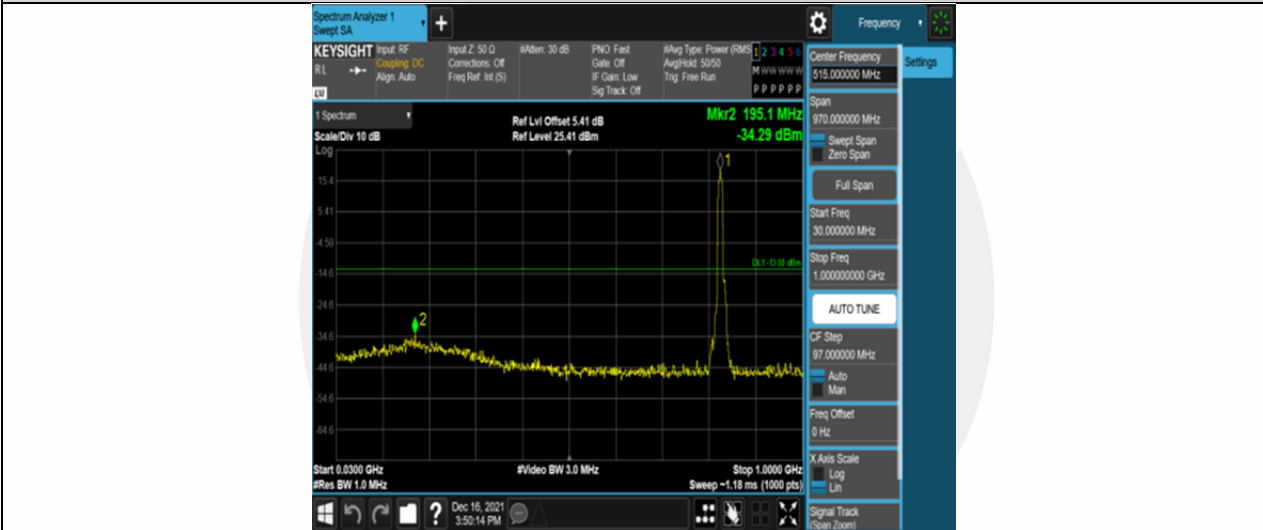
Band26-10MHz-16QAM-26840-50RB#0-Range1:30~1000MHz
