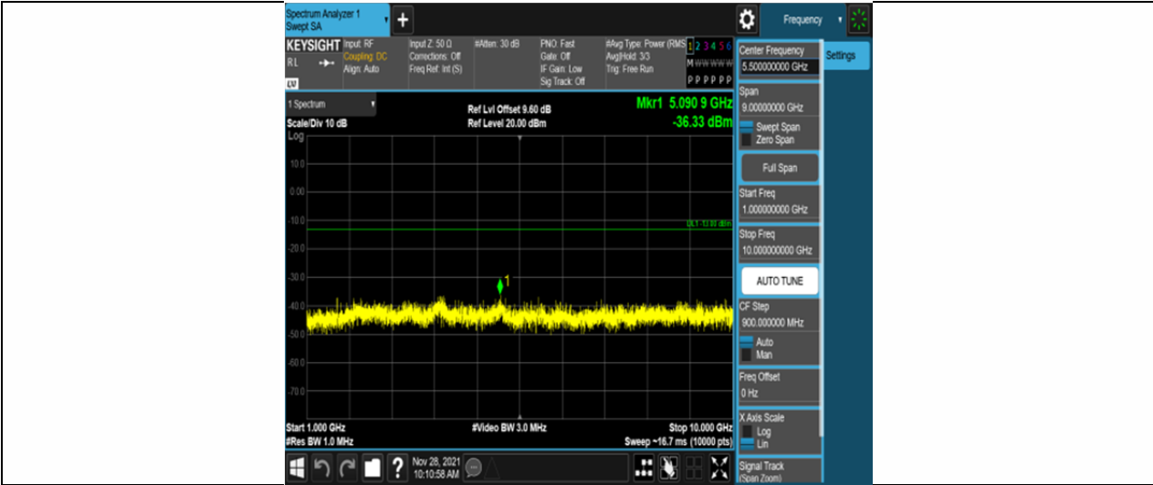
Band26-10MHz-16QAM-26740-50RB#0-Range2:1000~10000MHz
