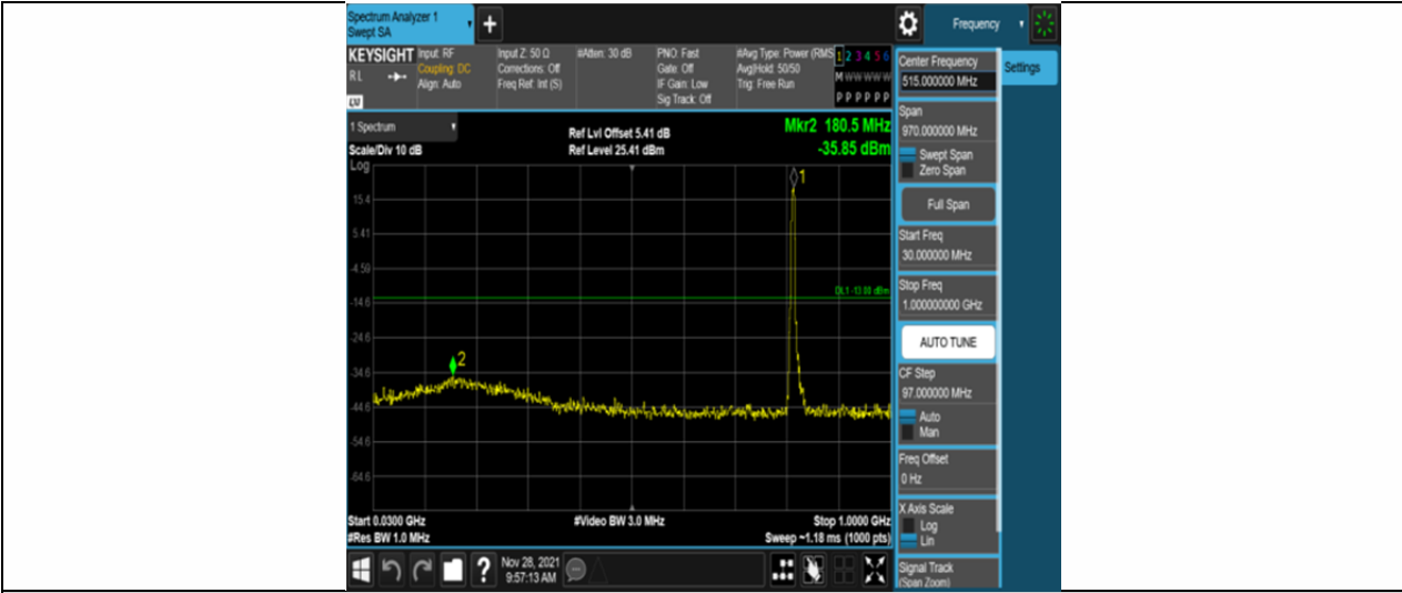
Band26-5MHz-QPSK-26715-25RB#0-Range1:30~1000MHz
