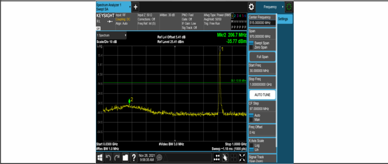
Band26-5MHz-16QAM-26740-25RB#0-Range1:30~1000MHz
