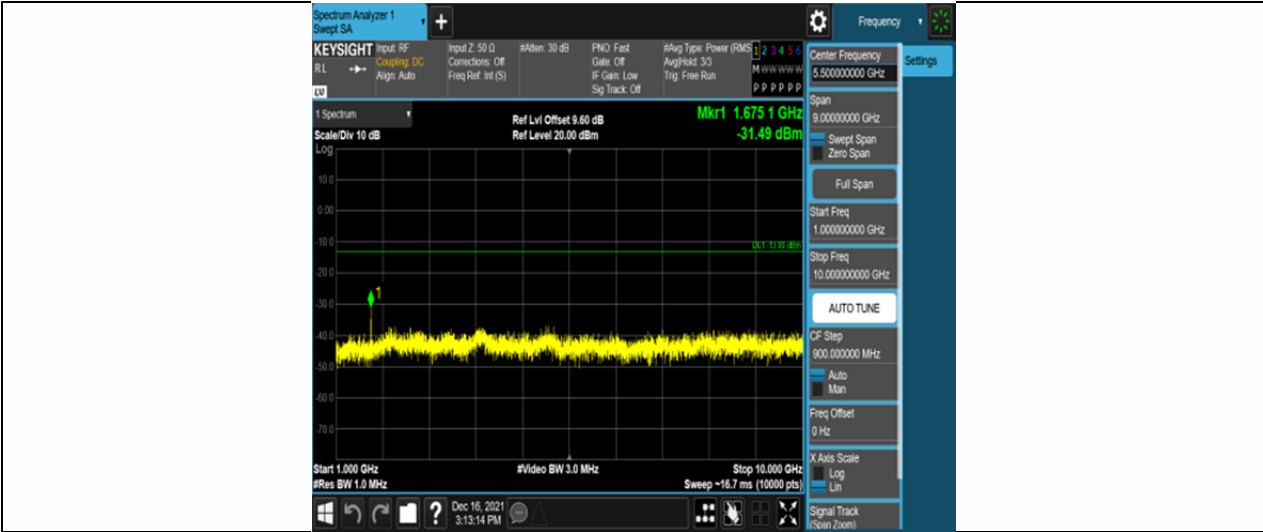
Band26-3MHz-16QAM-26915-15RB#0-Range2:1000~10000MHz
