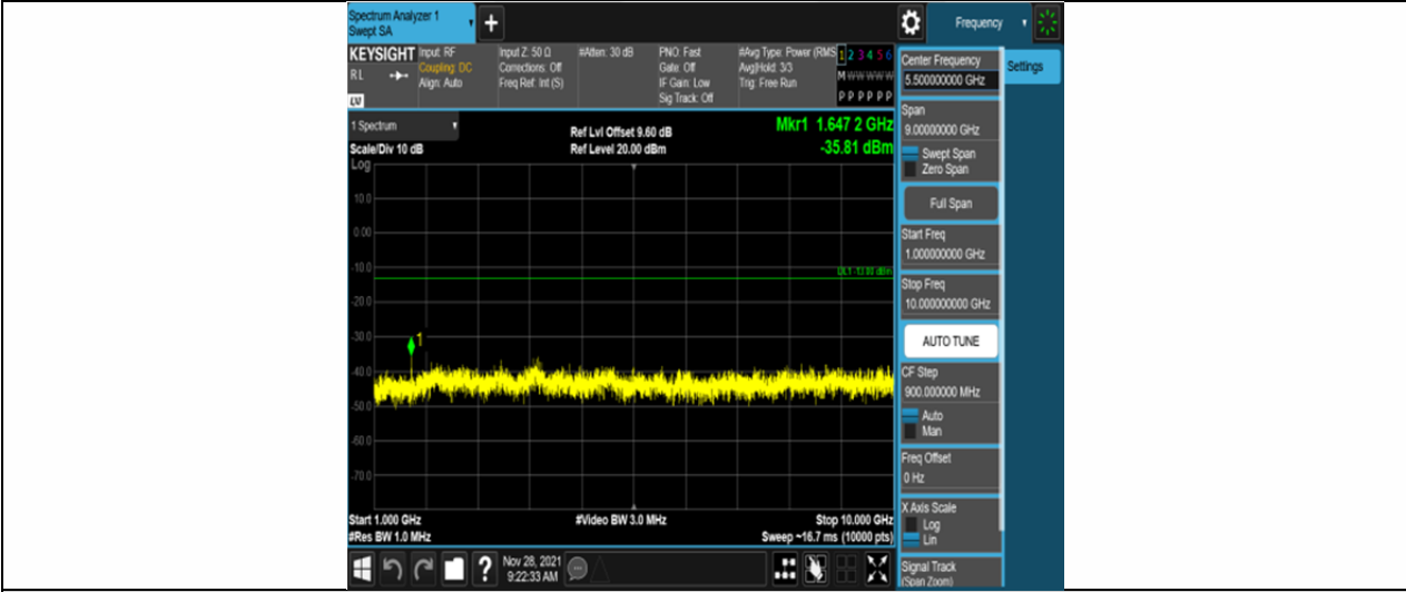
Band26-1.4MHz-QPSK-26783-6RB#0-Range2:1000~10000MHz
