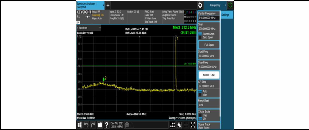
Band26-1.4MHz-QPSK-26797-6RB#0-Range1:30~1000MHz
