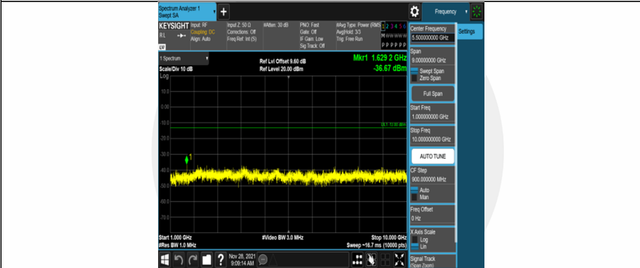
Band26-1.4MHz-16QAM-26697-6RB#0-Range2:1000~10000MHz
