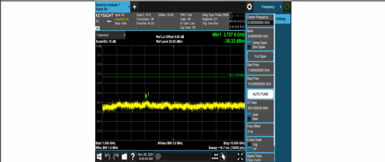
Band26-3MHz-16QAM-26775-1RB#0-Range2:1000~10000MHz
