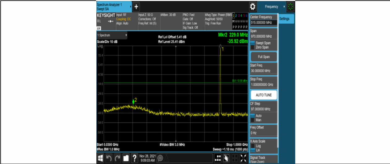
Band26-1.4MHz-16QAM-26697-6RB#0-Range1:30~1000MHz
