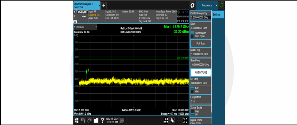
Band26-3MHz-16QAM-26705-1RB#0-Range2:1000~10000MHz
