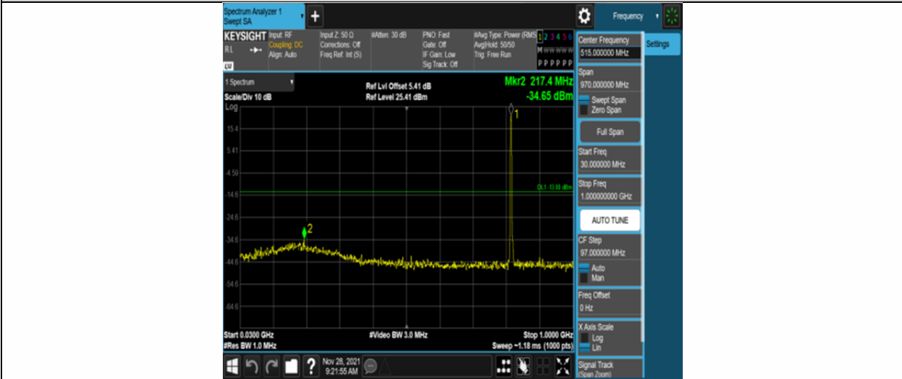
Band26-1.4MHz-16QAM-26740-6RB#0-Range1:30~1000MHz
