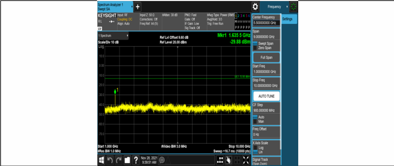
Band26-3MHz-16QAM-26740-1RB#0-Range2:1000~10000MHz
