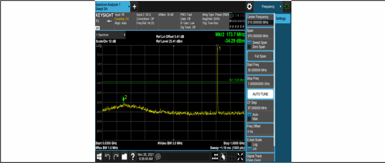
Band26-3MHz-16QAM-26705-1RB#0-Range1:30~1000MHz
