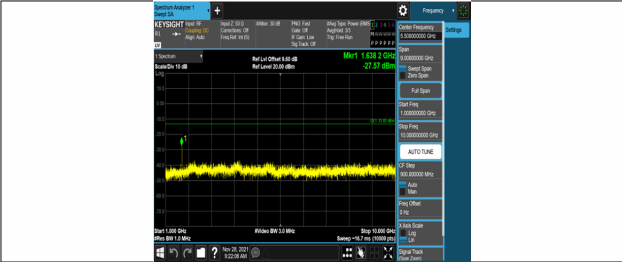
Band26-1.4MHz-16QAM-26740-6RB#0-Range2:1000~10000MHz
