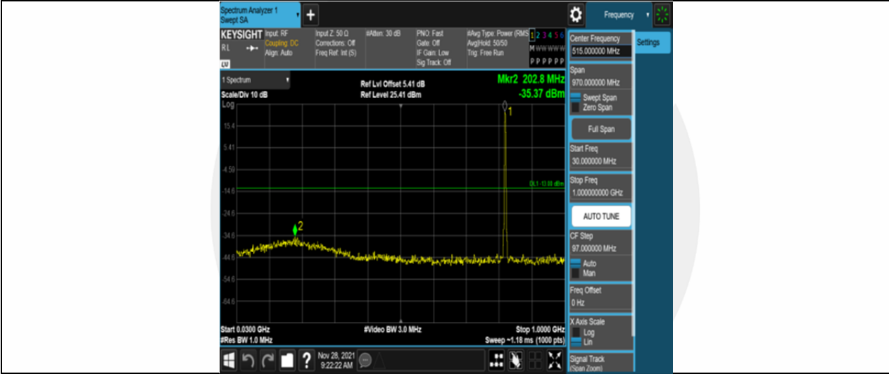
Band26-1.4MHz-QPSK-26783-6RB#0-Range1:30~1000MHz
