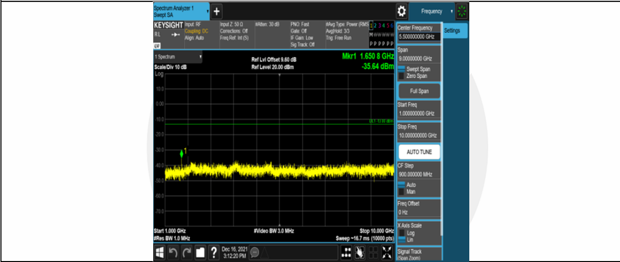
Band26-3MHz-16QAM-26805-15RB#0-Range2:1000~10000MHz
