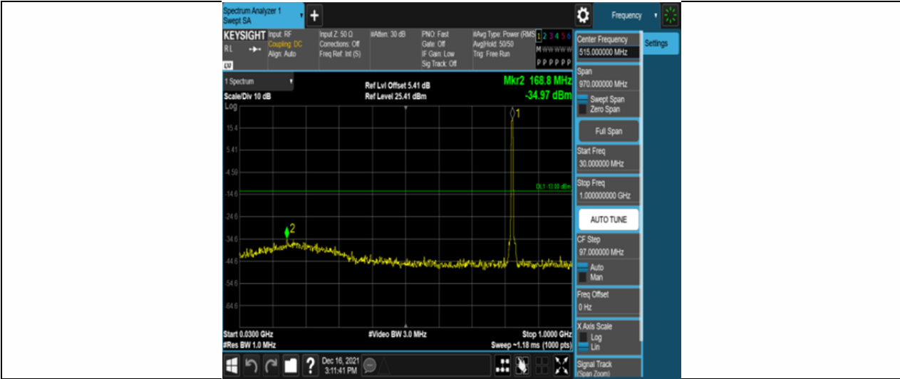
Band26-3MHz-QPSK-26805-15RB#0-Range1:30~1000MHz
