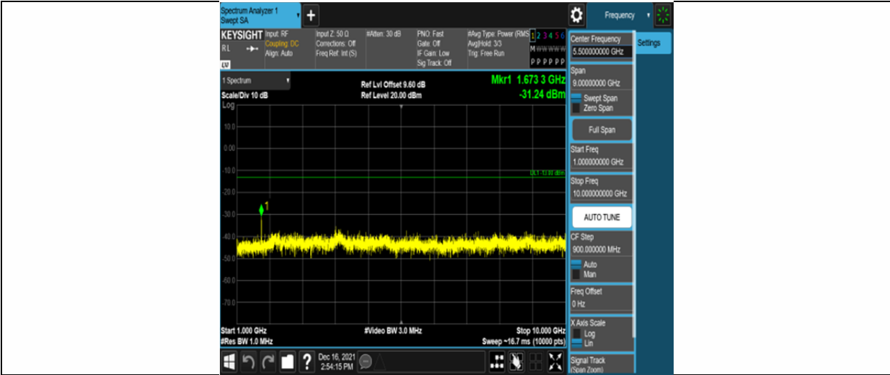
Band26-1.4MHz-QPSK-26915-6RB#0-Range2:1000~10000MHz
