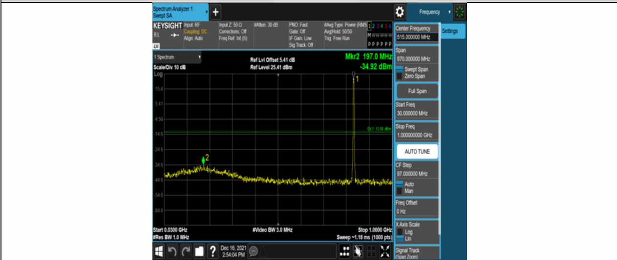
Band26-1.4MHz-QPSK-26915-6RB#0-Range1:30~1000MHz
