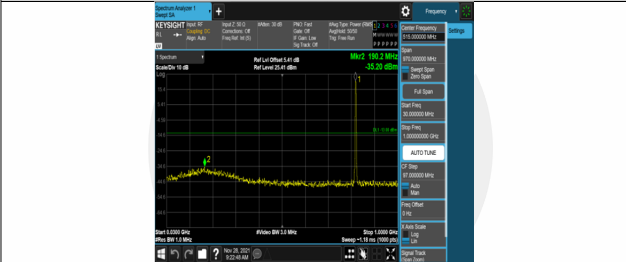
Band26-1.4MHz-16QAM-26783-6RB#0-Range1:30~1000MHz
